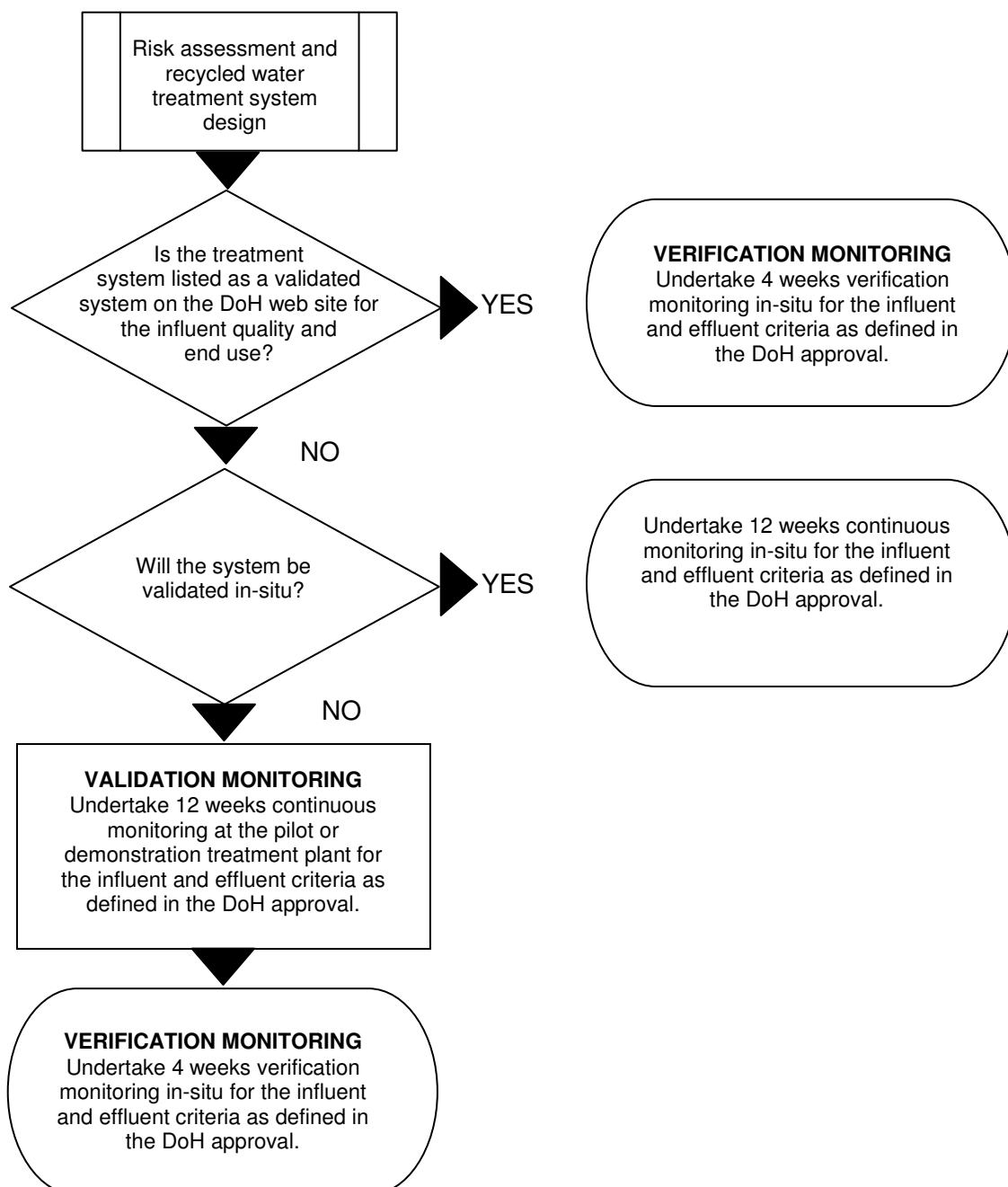
Figure 2 Flow chart validation and verification monitoring requirements
