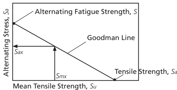
Goodman Diagram
