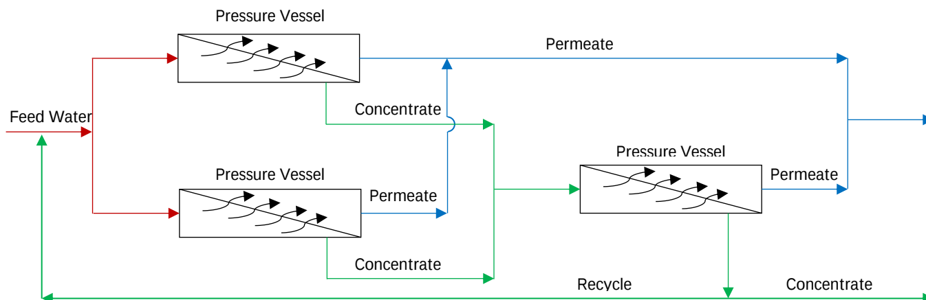
Figure 3. A two-stage system with a concentrate recycle stream back to the feed stream.
