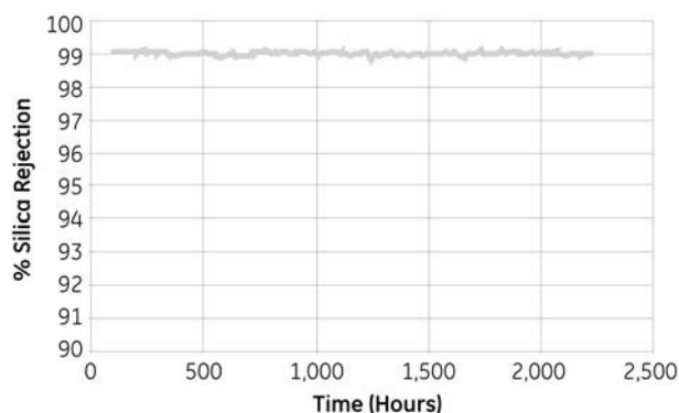
Figure 7: Percent Silica Rejection vs. Time June 1998 - Present
