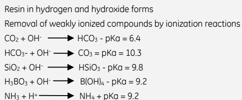
Figure 2: Ionization Reactions in EDI Diluting Compartments
