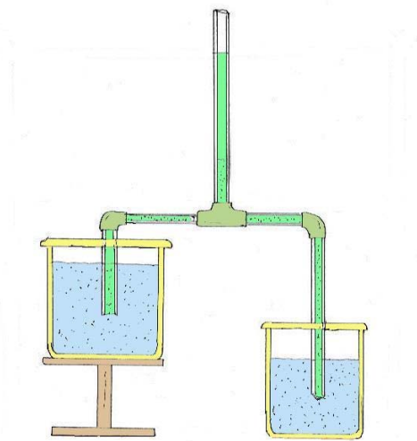
PASCAL'S SIPHON
