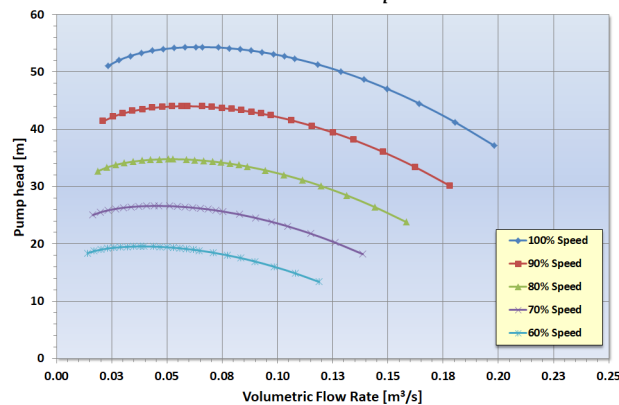
Fig 9. Pump Performance Curves – Various Speeds
