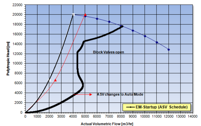
Figure 6. Case 2: Operating Point Migration
