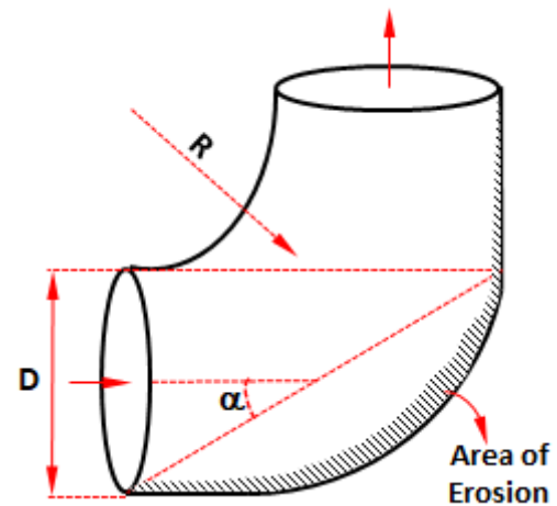
Figure 2. Impact Angle \alpha in Pipeline Bends
