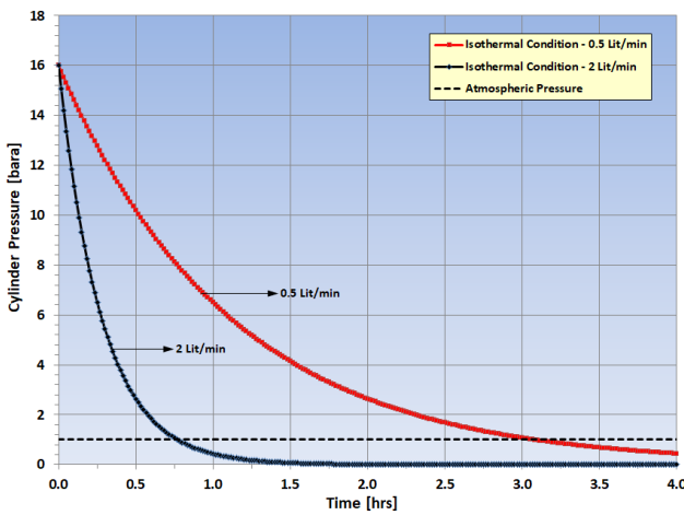
Figure 1. Cylinder Pressure vs. Time
