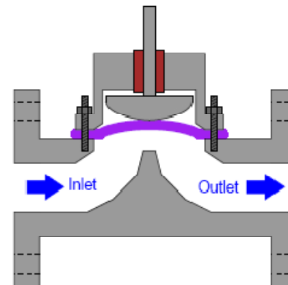
Diaphragm valve
