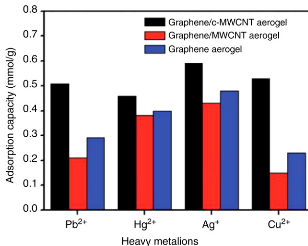
Figure 2.3. Binding capacities of graphene-MWCNTs for heavy metals ( \text{Pb}^{2+} , \text{Hg}^{2+} , \text{Ag}^{+} , \text{Cu}^{2+} ). From Sui, Z., Meng, Q., Zhang, X., Ma, R. Cao, B., 2012. Green synthesis of carbon nanotube-graphene hybrid aerogels and their use as versatile agents for water purification. J. Mater. Chem. 22, 8767–8771, Copyright © 2012, Royal Society of Chemistry.
