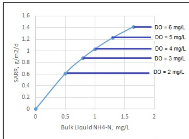
Figure 9. Adapted from Metcalf & Eddy (2014), Fig 9-25
