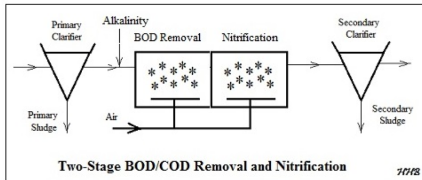
Figure 15. Two-Stage MBBR Process for BOD Removal and Nitrification
