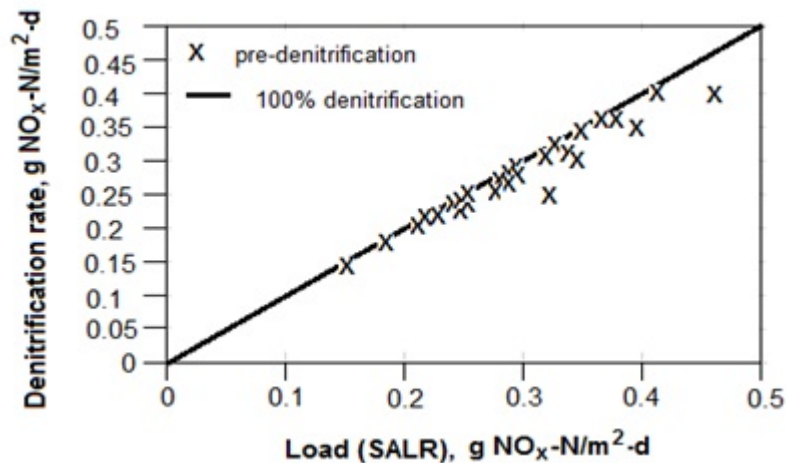
Figure 21. SARR/SALR vs SALR for Pre-Anoxic Denitrification
