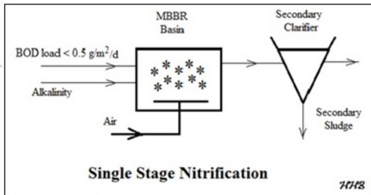
Figure 8. Single Stage MBBR Process for Nitrification
