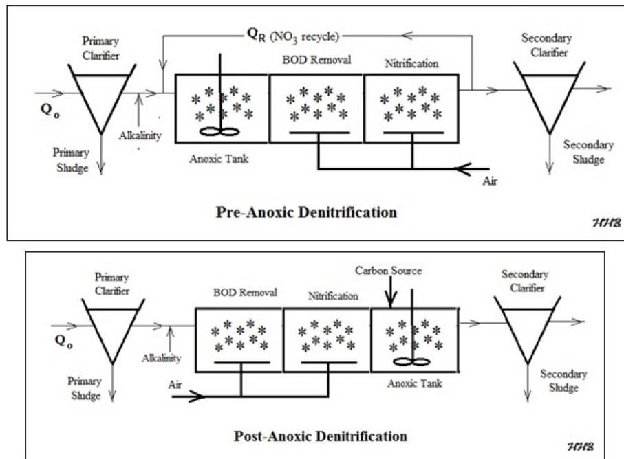
Figure 16. MBBR Denitrification Process Alternatives
