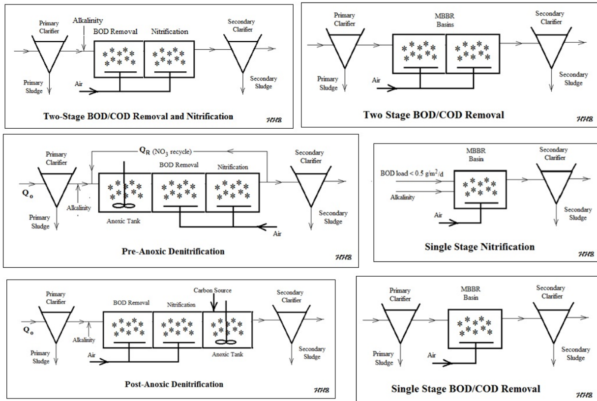
Figure 4. MBBR Wastewater Treatment Process Alternatives
