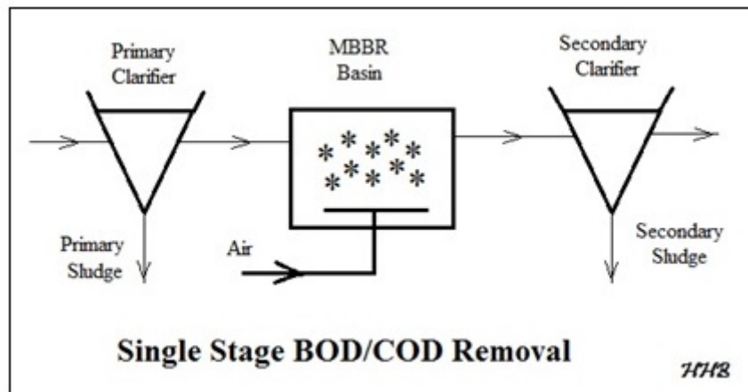
Figure 5. Single Stage MBBR Process for BOD/COD Removal
