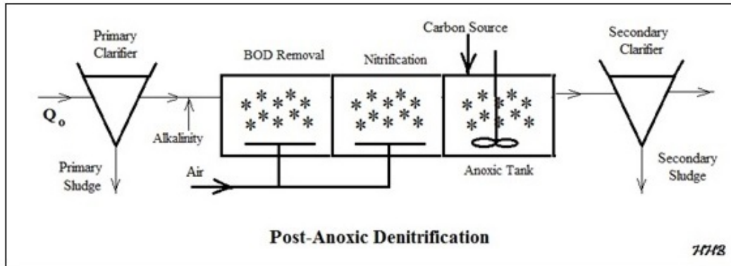
Figure 17. Flow Diagram for Post-Anoxic Denitrification
