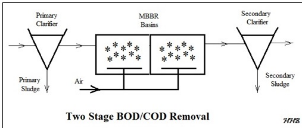
Figure 12. Two-Stage MBBR Process for BOD/COD Removal
