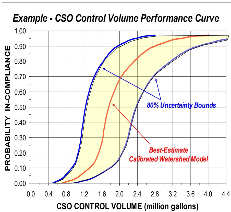
Figure 7-8 Example of Risk-Based CSO Volume Curves
