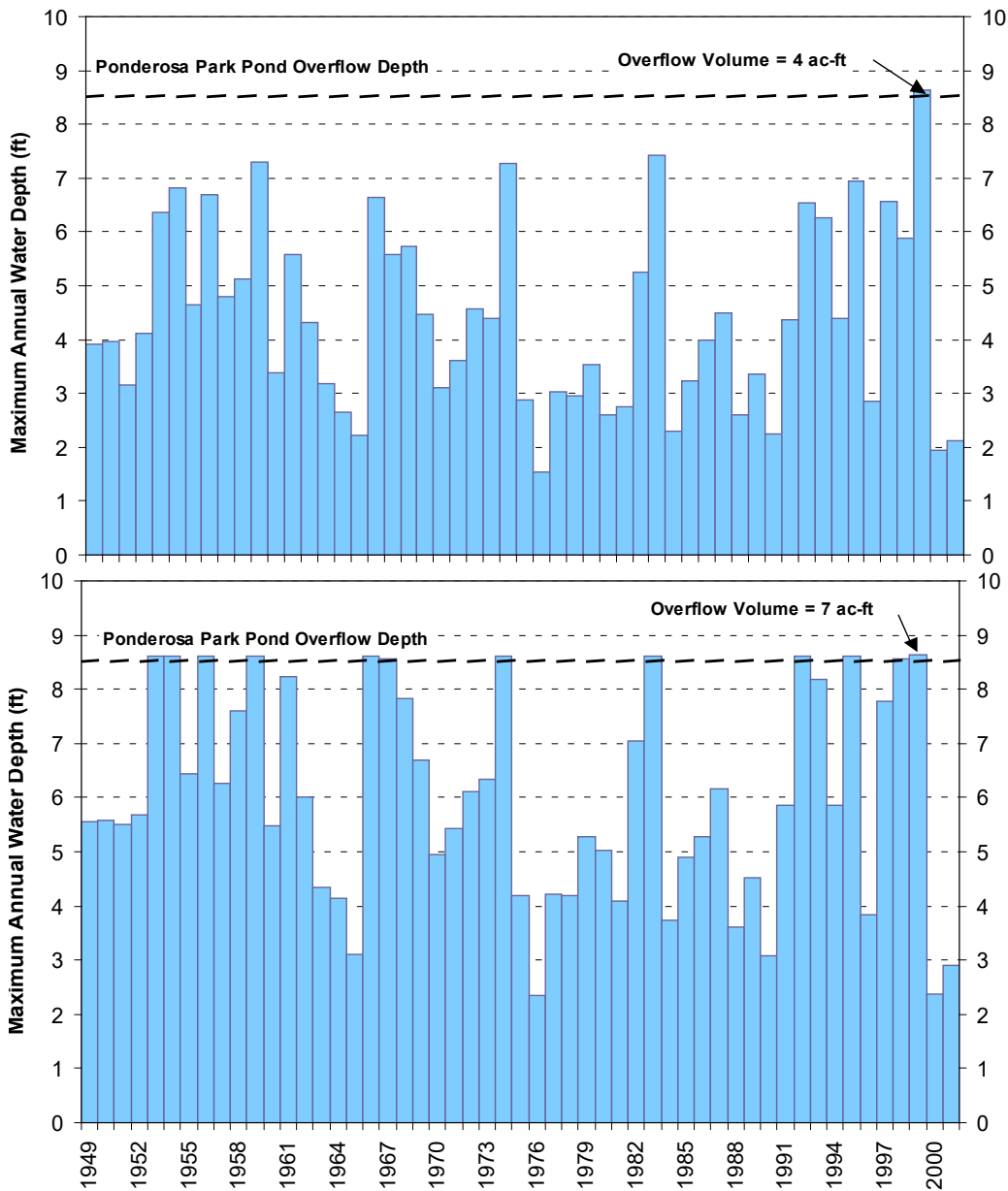
Figure 7-12 Simulated Maximum Annual Detention Pond Depth for Existing and Future Land Use
