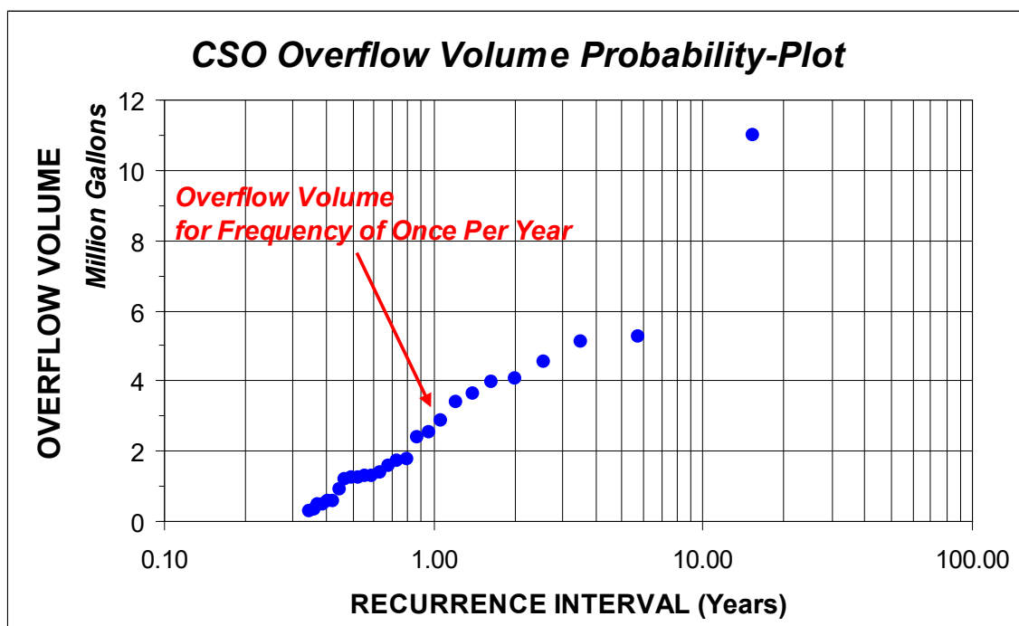
Figure 7-13 Frequency-Volume Distribution of CSO Events
