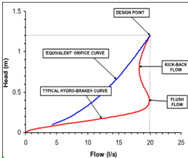
Figure 7-2 Head vs. Flow Performance Curve for a Hydrobrake
