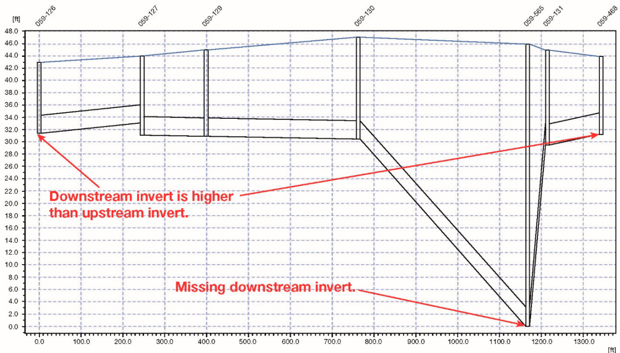
Figure 7-5 Sewer Attributes to Flag and Confirm during QA/QC for Profile Data
