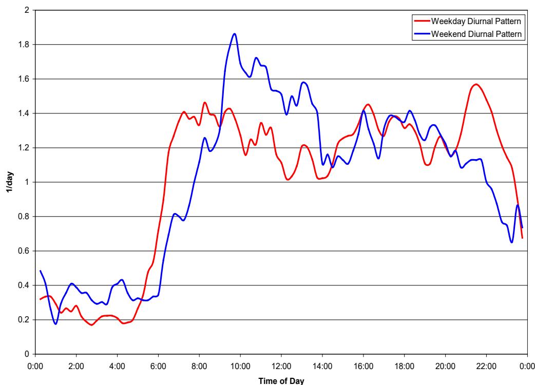
Figure 7-3 Example of Dry-Weather Flow Diurnal Patterns
