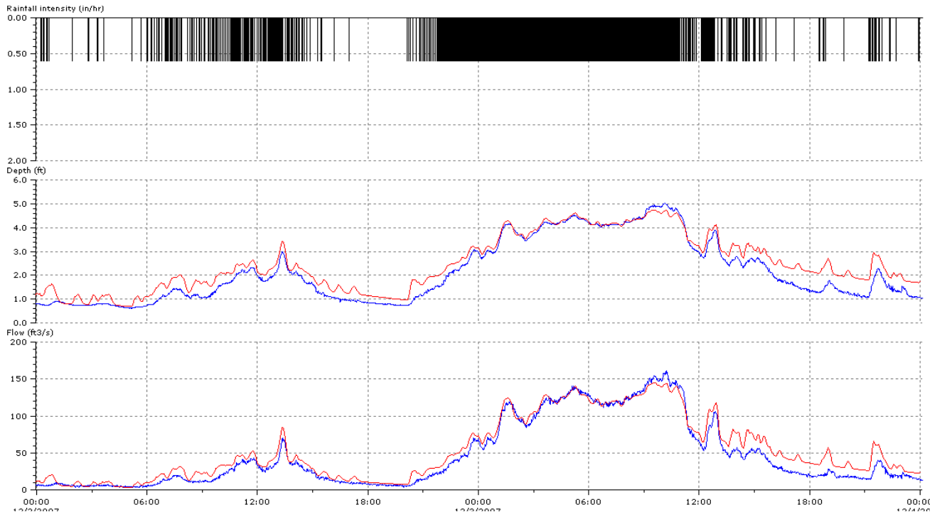
Figure 7-7 Example of Calibration Comparing Simulated and Observed Depth and Flow
