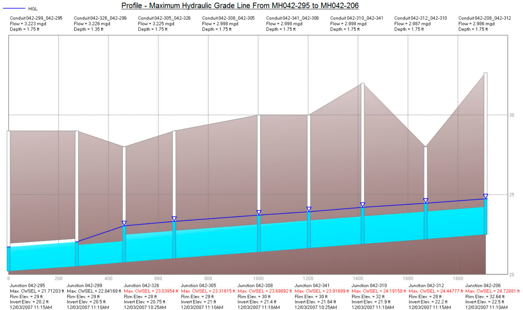
Figure 7-10 Profile View: Capacity Assessment Simulation
