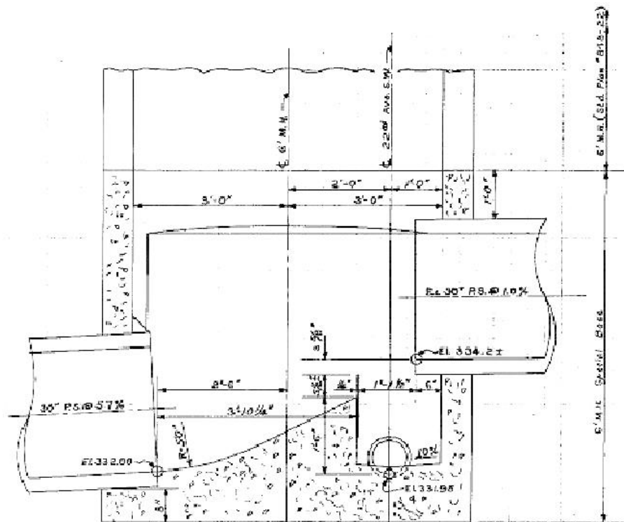
Figure 7-1 Example of Leaping Weir
