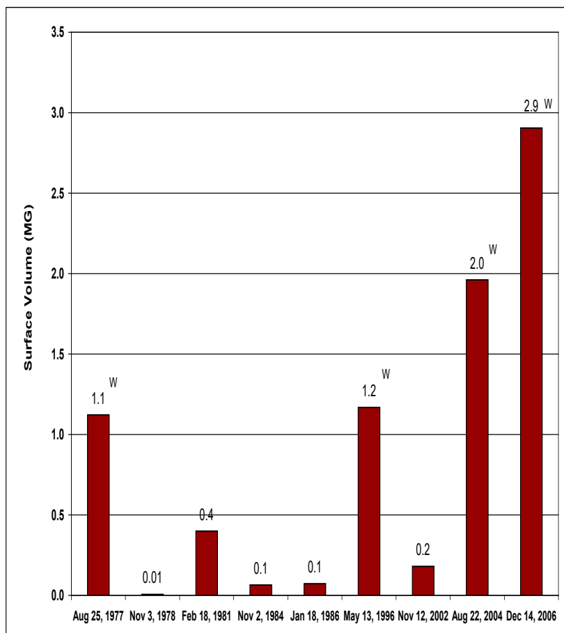
Figure 7-11 Overflow Example Derived From Long-Term Continuous Simulation
