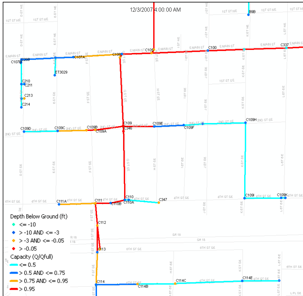
Figure 7-9 Plan View: Capacity Assessment Simulation Results
