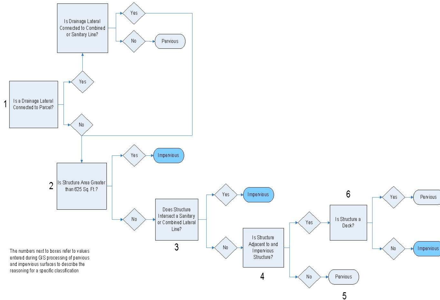
Figure 7-4 Impervious vs. Pervious Area High-Flow Diagram
