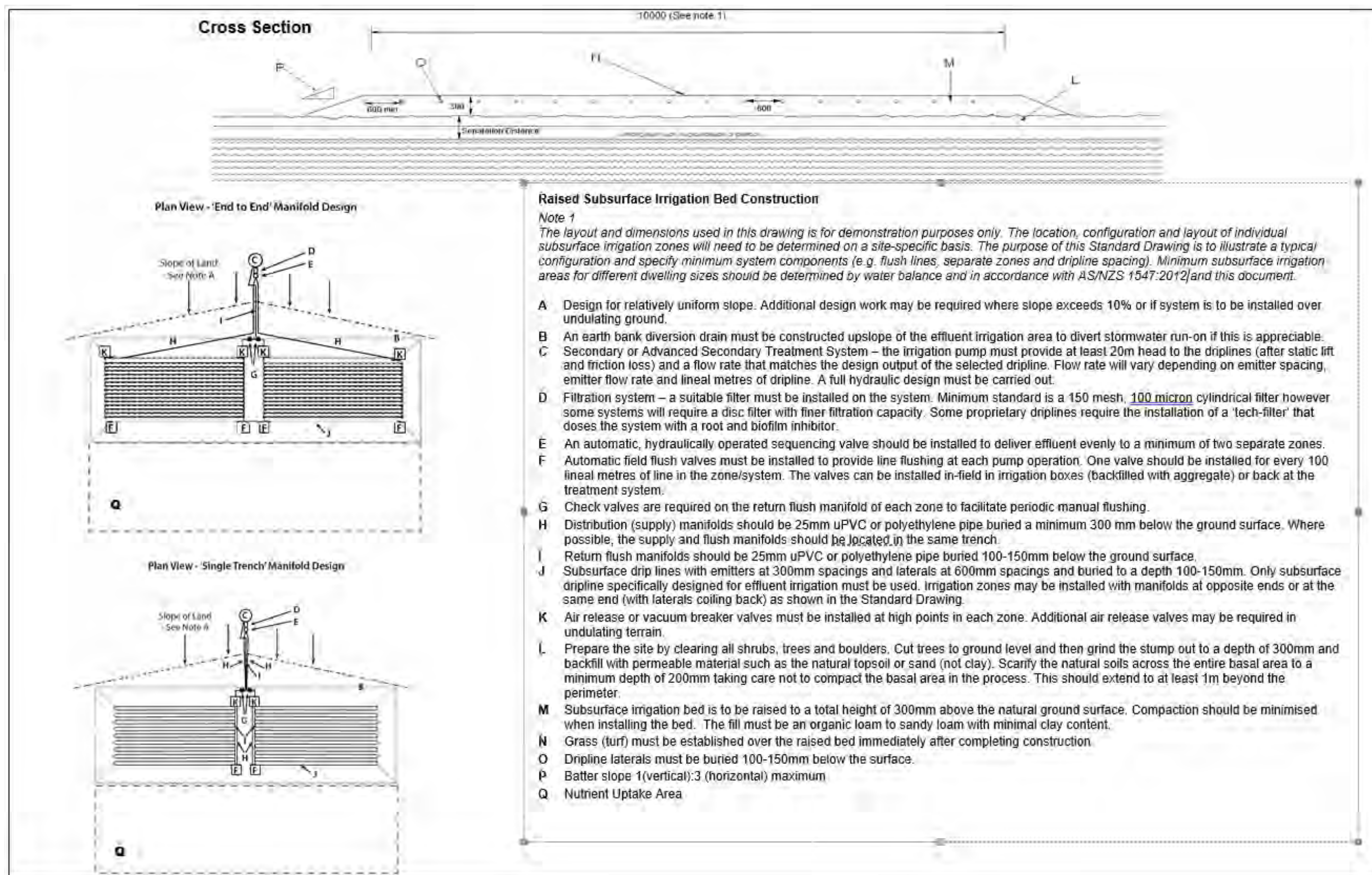
Standard Drawing 13C – Raised Subsurface Irrigation Bed
