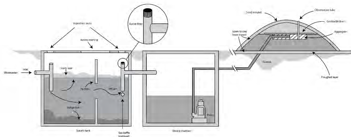
Figure 9.1 Components of a Wisconsin sand mound system
