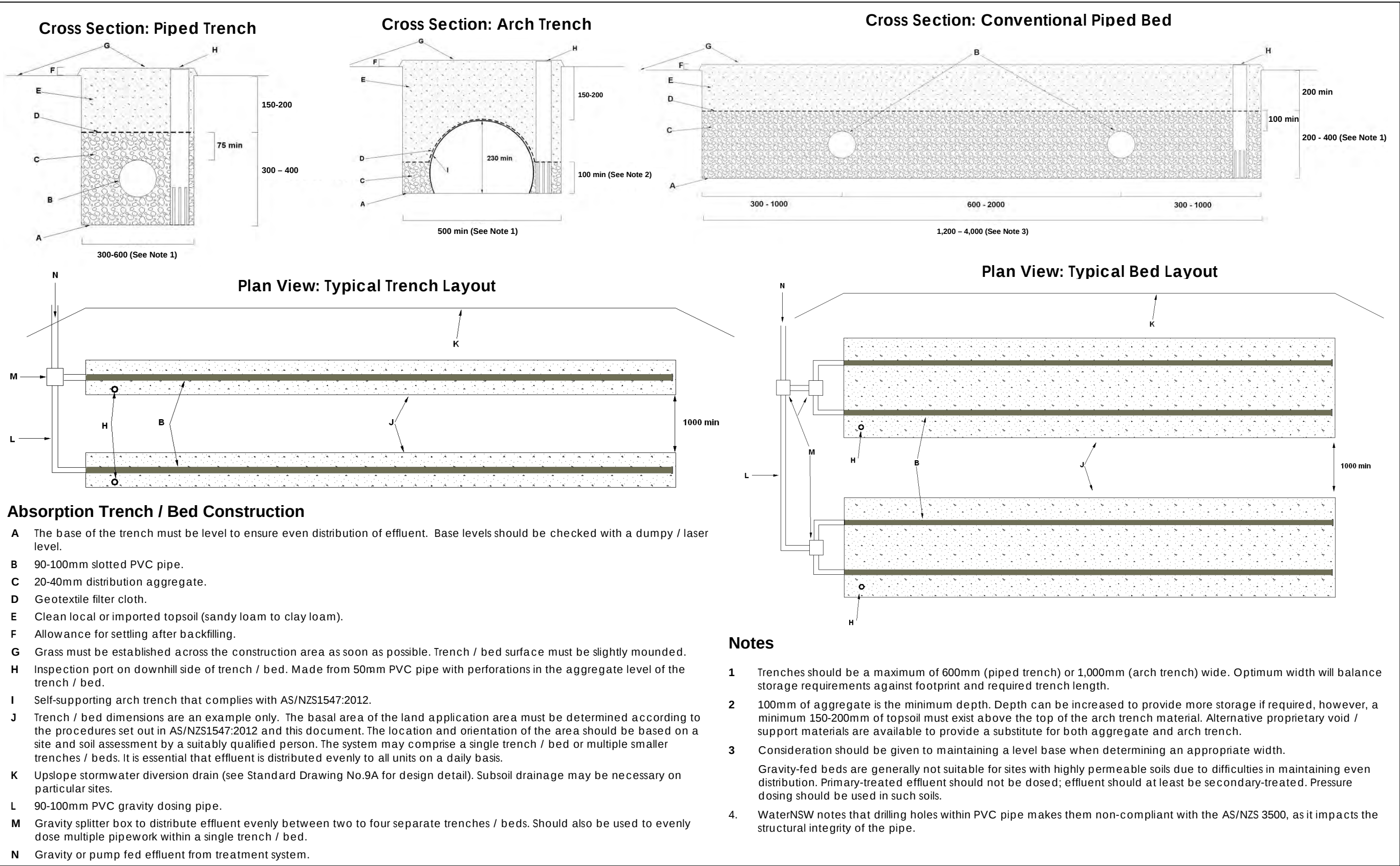
Standard Drawing 10B – Absorption Trench / Bed
