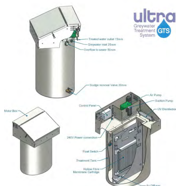
Figure 7.2 Schematic of an Ultra GTS (Wastewater Australia)
