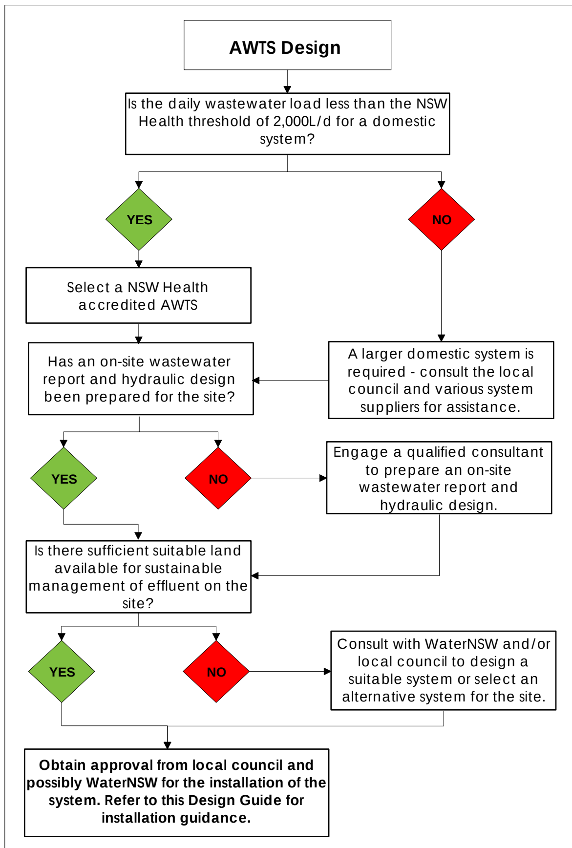
Figure 4.2 AWTS Design
