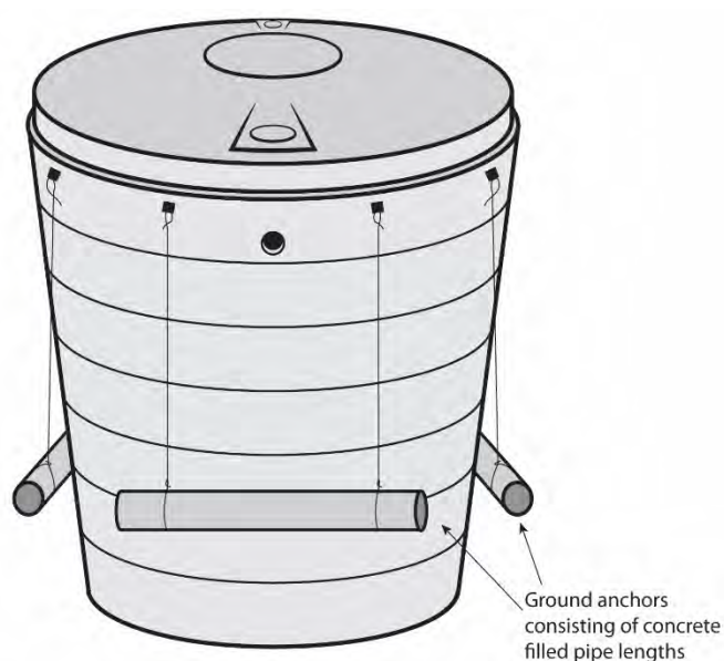
Figure 3.4 Ground anchors
