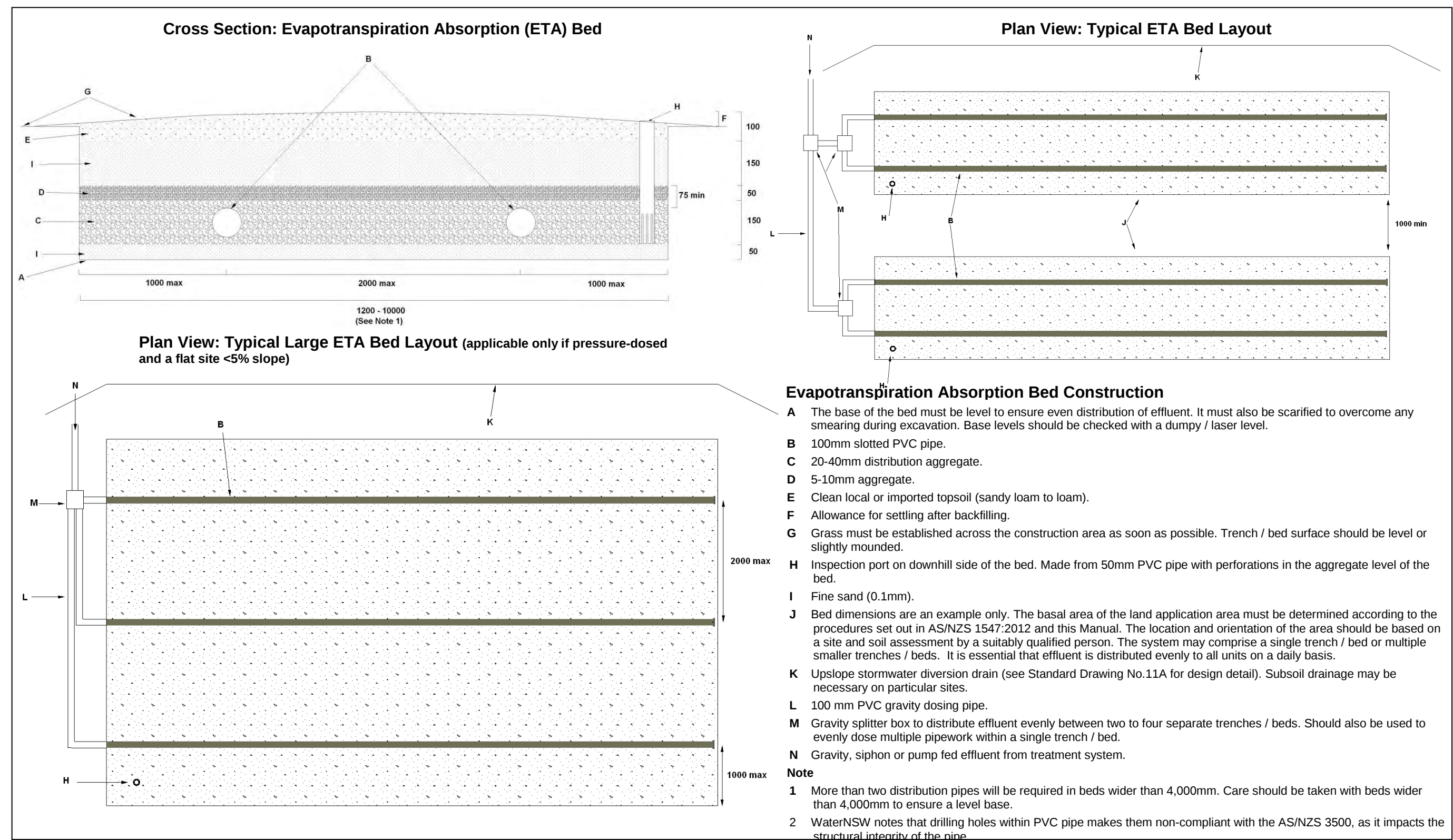
Standard Drawing 11B – Evapotranspiration Absorption Bed
