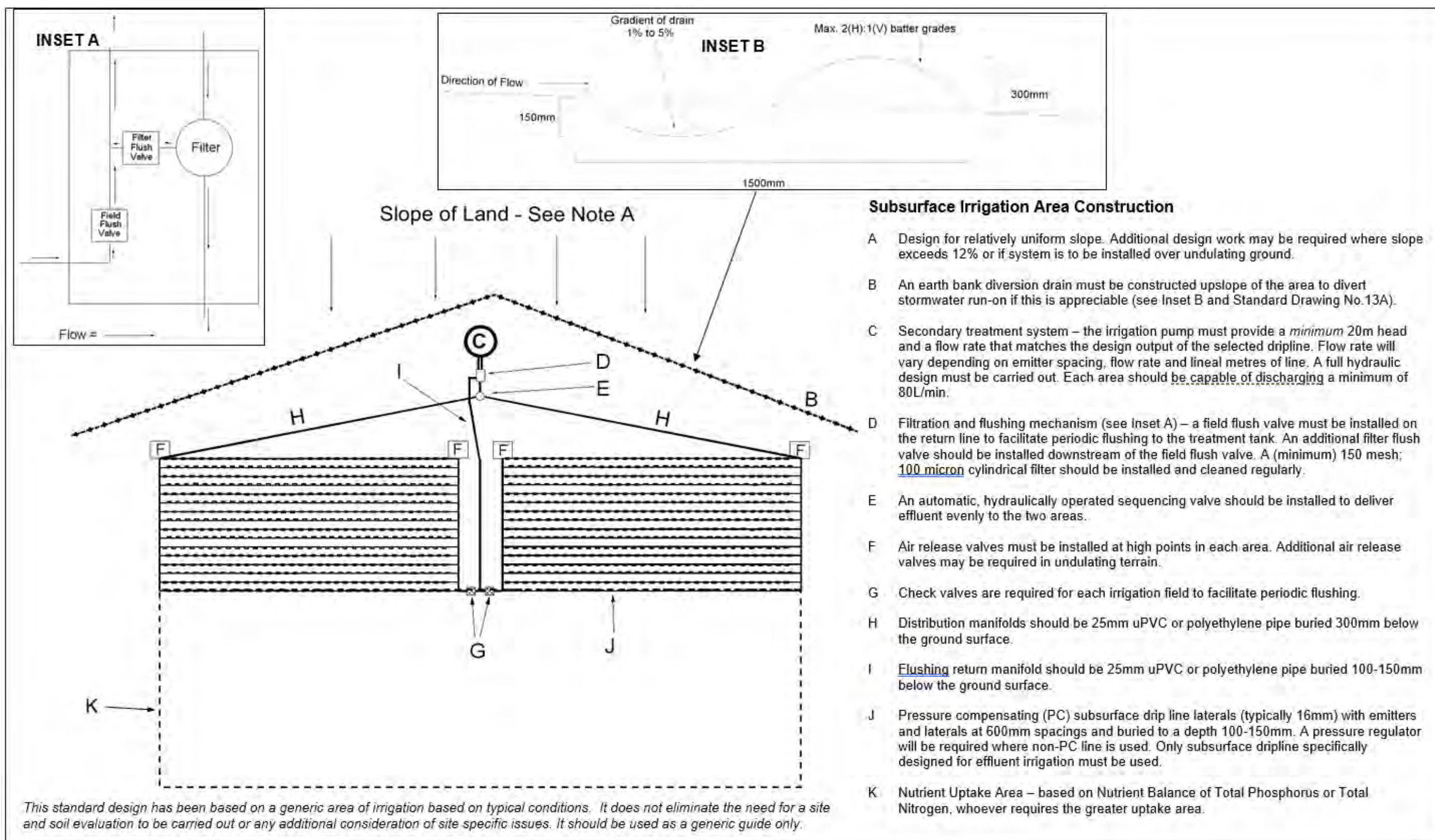
Standard Drawing 13B – Subsurface Effluent Irrigation
