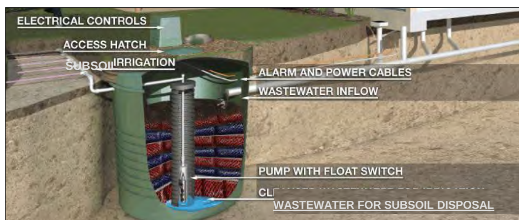
Figure 5.1 A Biological Filter System (after Biolytix, 2009)
