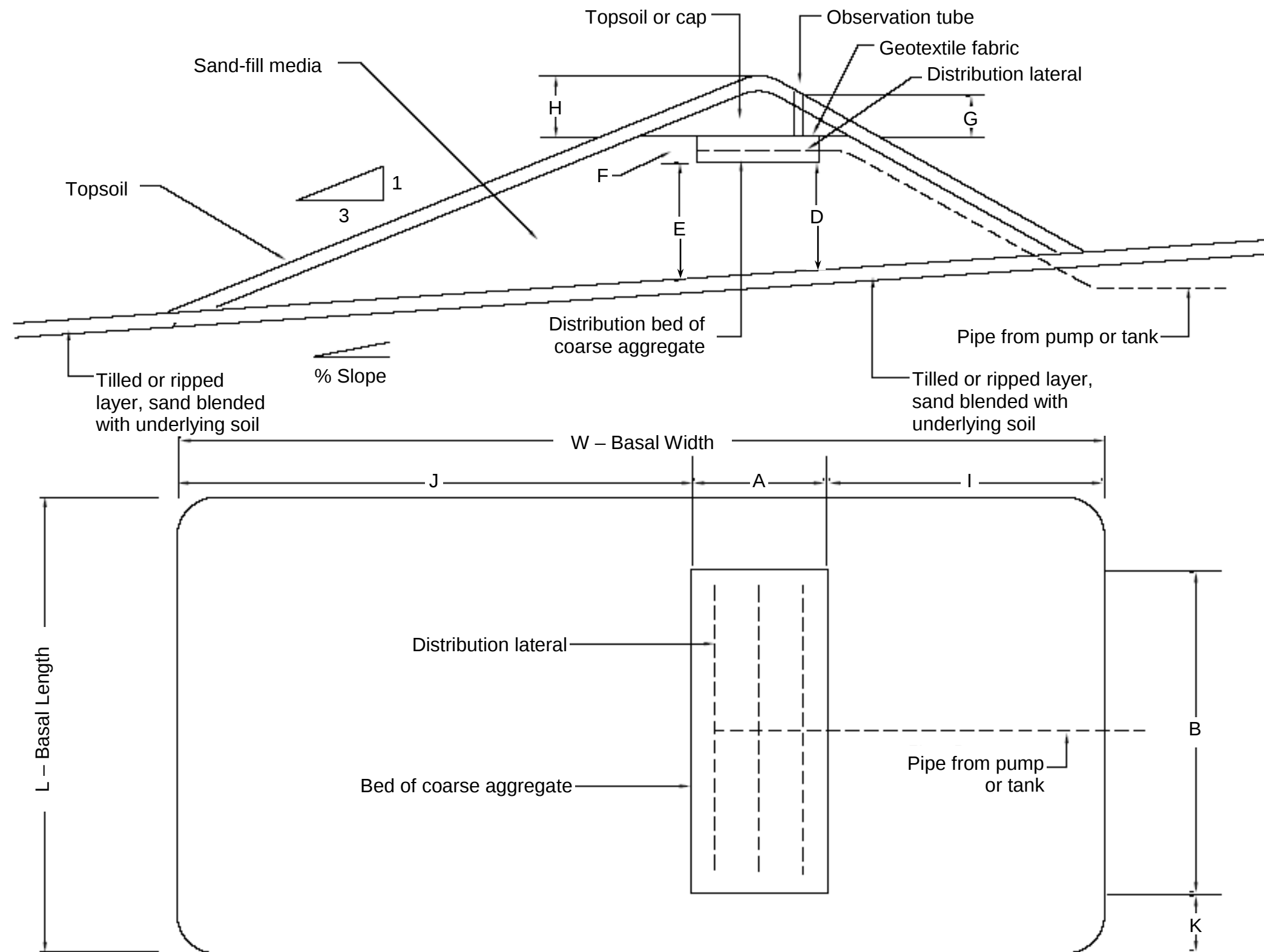
Standard Drawing 9B – Wisconsin Sand Mound (not to scale)
