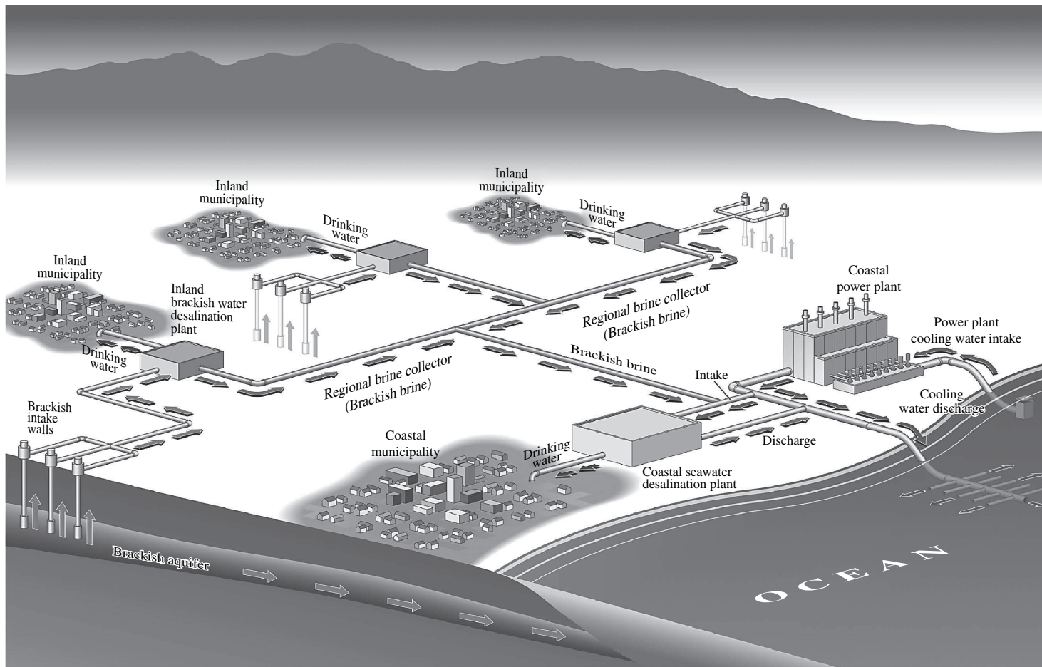
FIGURE 16.55 Integrated inland desalter brine disposal and seawater desalination.
