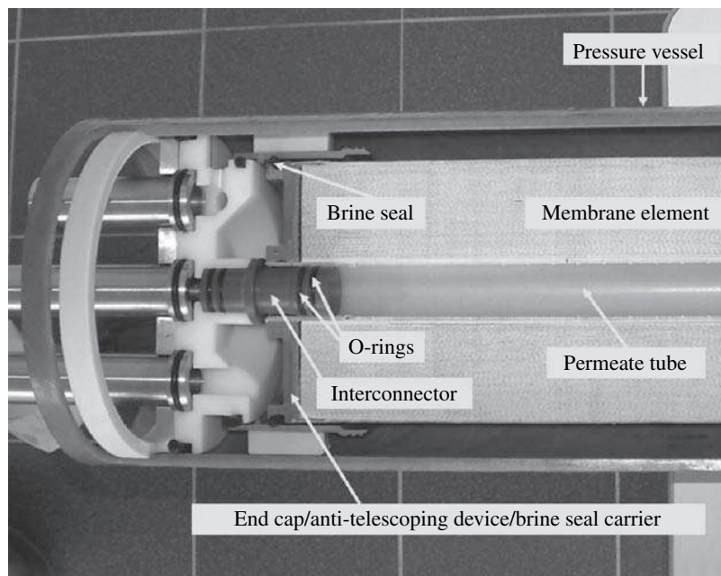
FIGURE 3.8 Cross-section of an RO membrane element installed in a pressure vessel.
