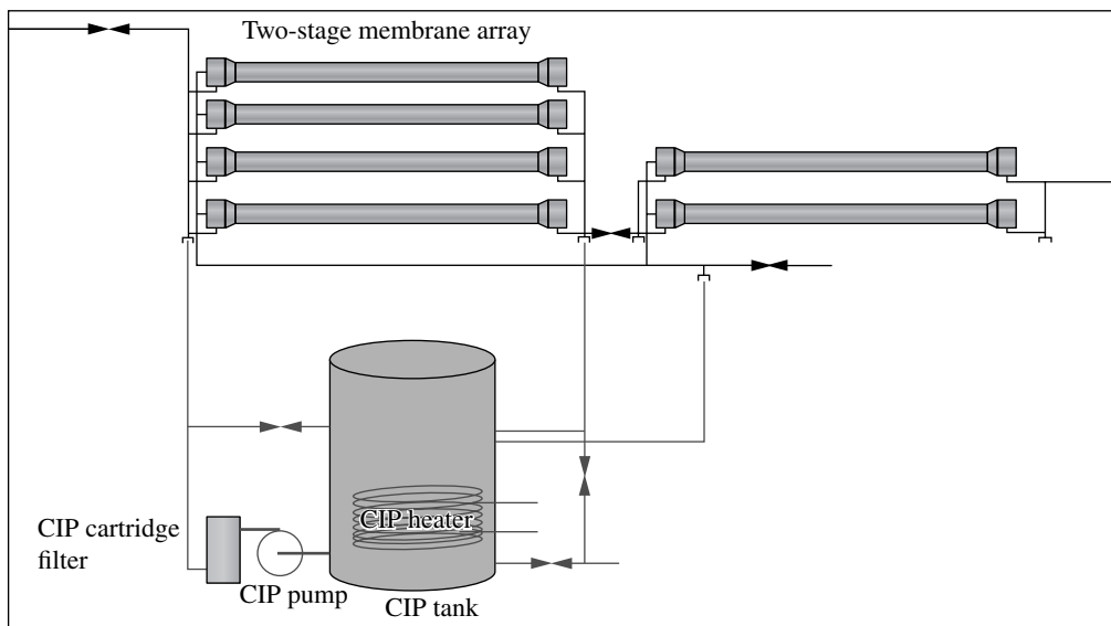
FIGURE 14.25 Schematic of a typical RO membrane cleaning system.
