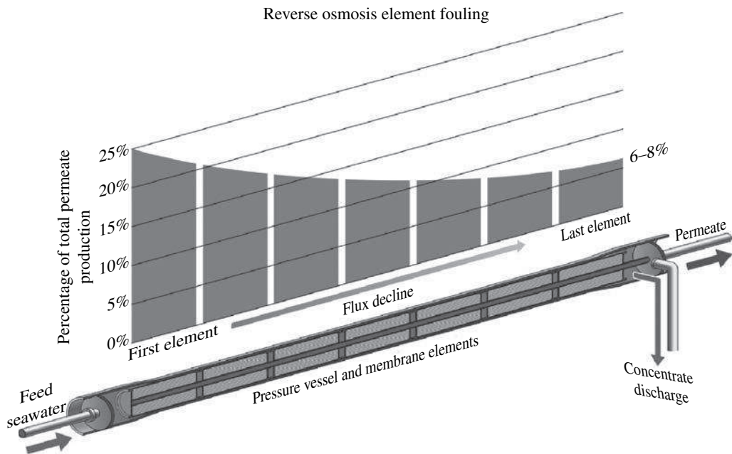
FIGURE 3.19 Membrane fouling and flux distribution in a membrane vessel.
