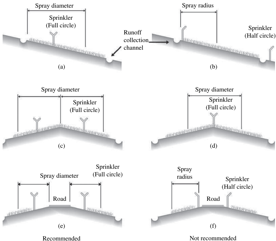
FIGURE 16.31 Sprinkler system configuration. (Source: US EPA, 2004.)
