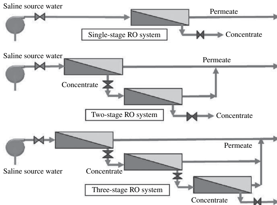
FIGURE 14.29 Single and multistage RO systems.
