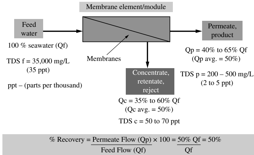
FIGURE 3.17 Recovery of a typical SWRO system.
