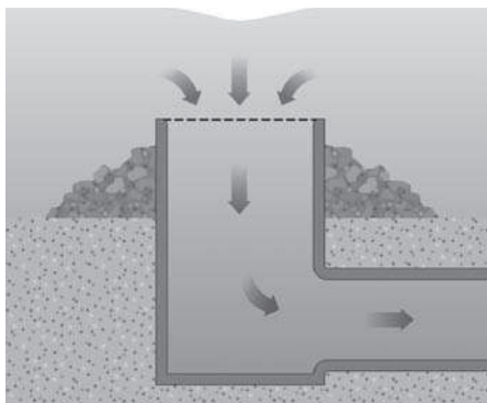
FIGURE 5.4 Velocity cap for entrainment reduction. (Source: US EPA.)
