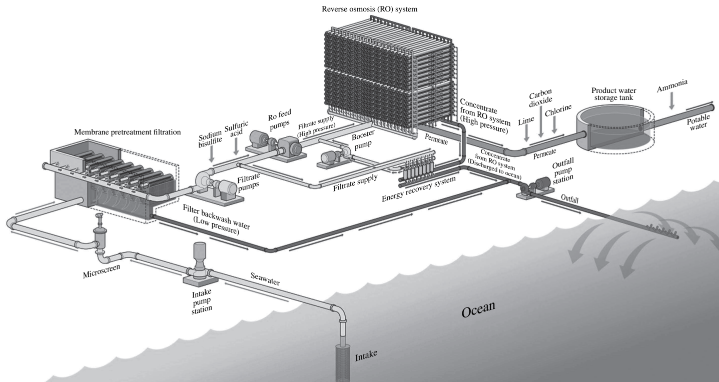
FIGURE 12.1 General schematic of a desalination plant with membrane pretreatment.
