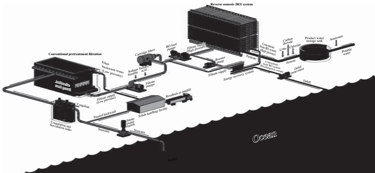
FIGURE 3.24 Schematic of a typical seawater desalination plant.
