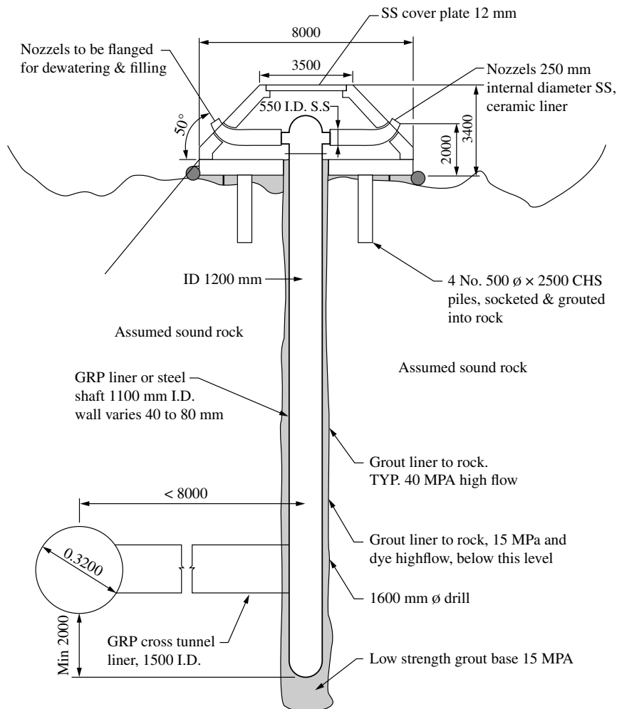
FIGURE 16.5 Outfall diffusers of Victorian SWRO plant (Source: Melbourne Water).
