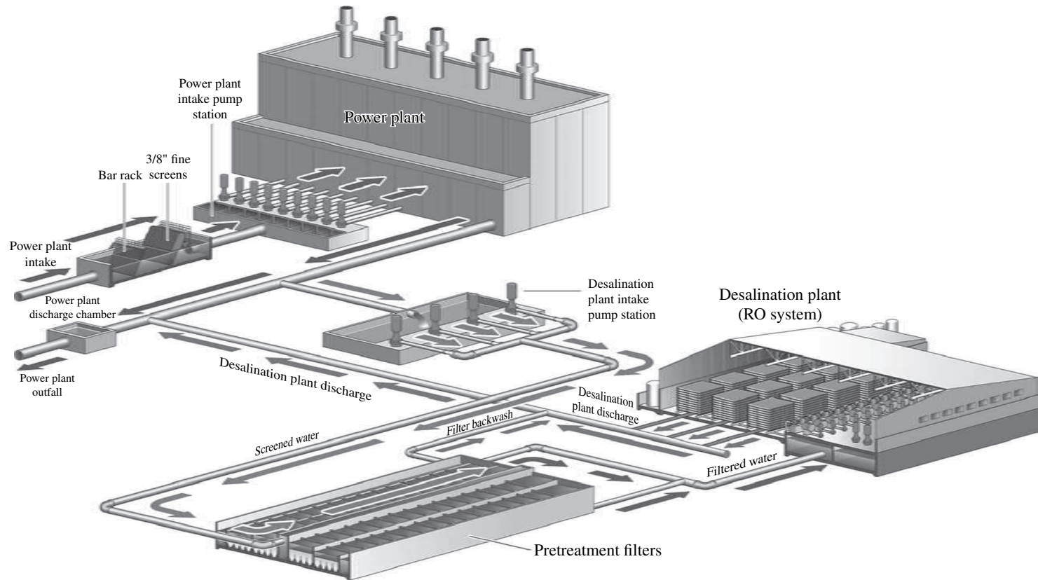
FIGURE 16.21 Configuration of co-located coastal desalination plant.
