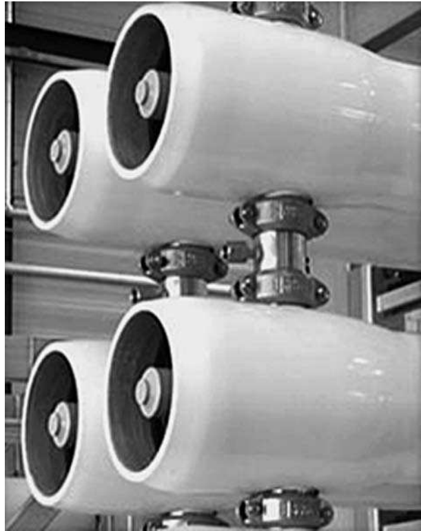
FIGURE 14.12 Multiple-port pressure vessels.
