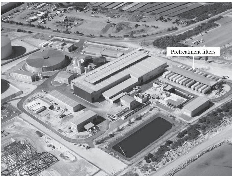
FIGURE 11.6 Single-stage horizontal pressure filters, Perth I SWRO plant. (Source: Water Corporation.)
