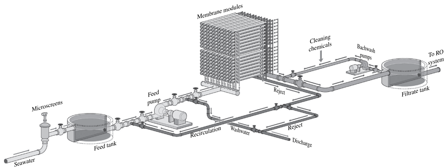
FIGURE 12.4 General schematic of a pressurized membrane pretreatment system.
