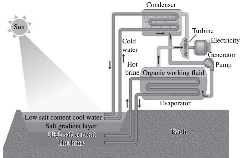
FIGURE 16.43 Solar pond schematic.
