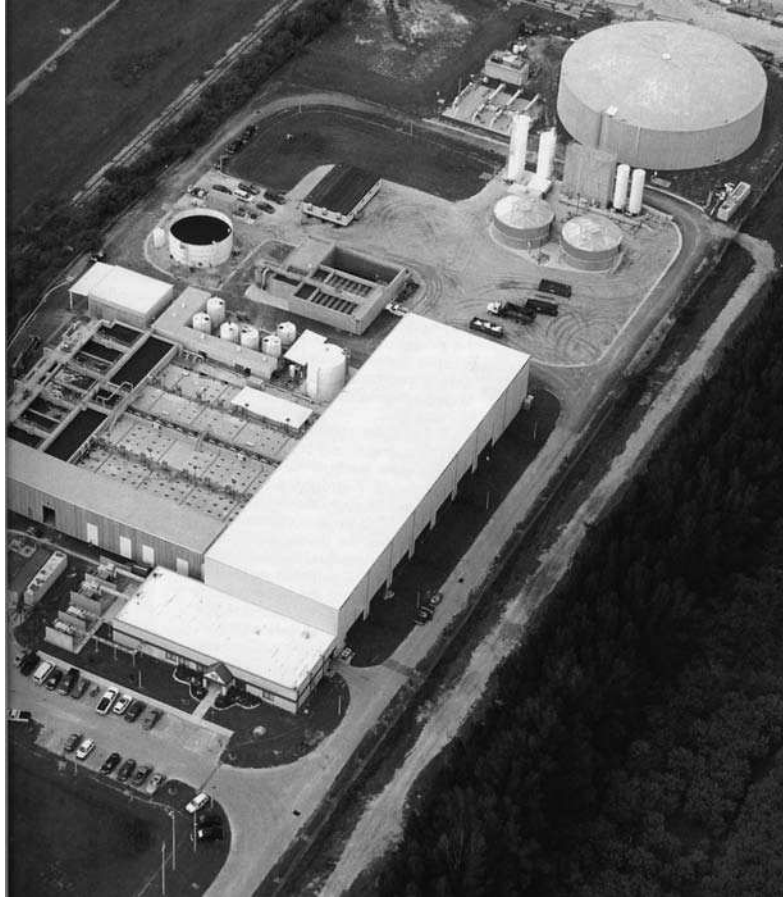
FIGURE 4.10 Layout of the Tampa Bay SWRO desalination plant, Florida. ( Tampa Bay Water. )
