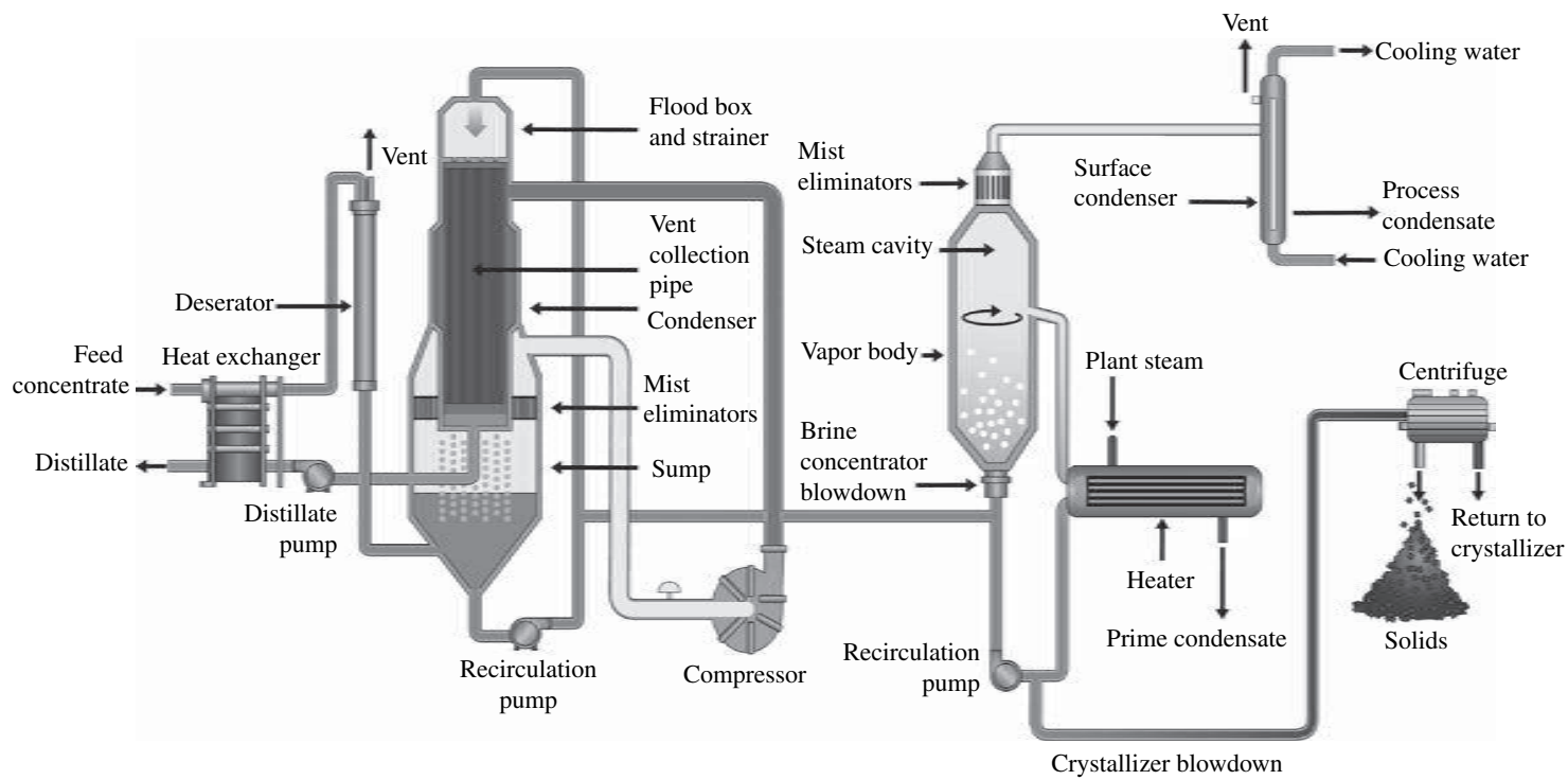
FIGURE 16.50 General schematic of evaporator crystallizer system.
