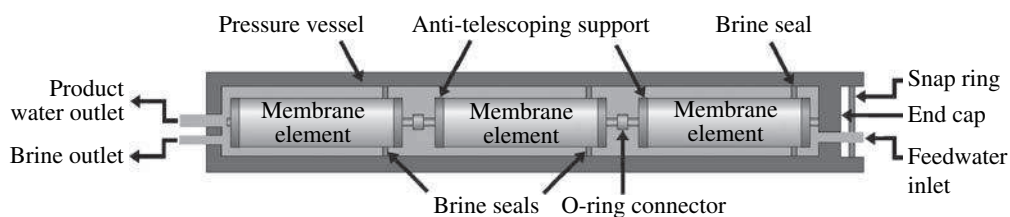
FIGURE 3.9 Membrane elements installed in a pressure vessel.
