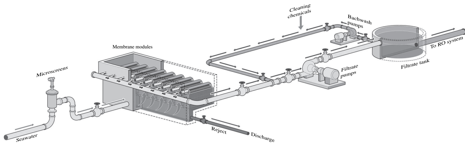
FIGURE 12.6 General schematic of a submerged membrane pretreatment system.
