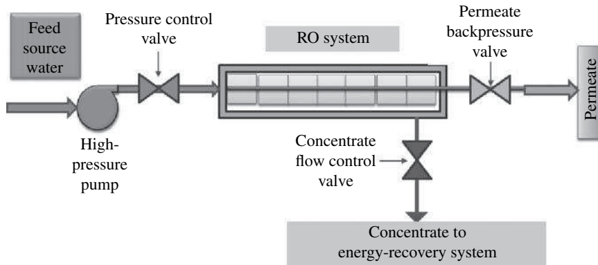
FIGURE 14.4 Main RO system control valves.
