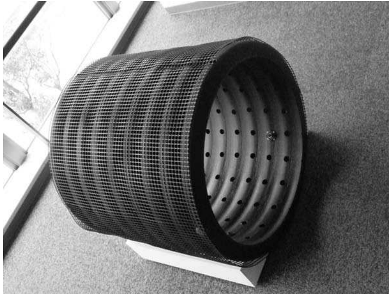
FIGURE 6.16 Segment of a 600-mm intake collector screen.
