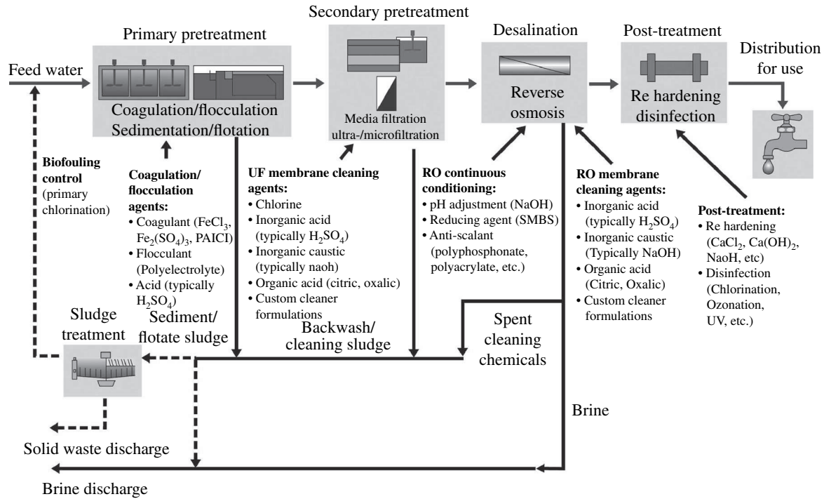
FIGURE 4.7 SWRO desalination plant schematic.
