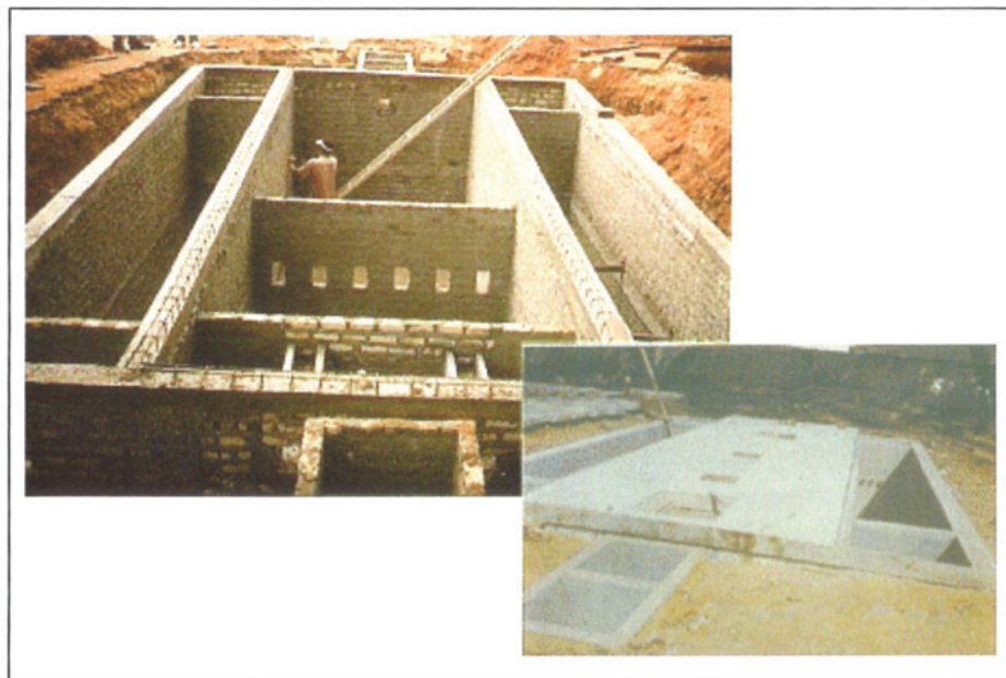
Figure 7: Photos of an Anaerobic Filter During Construction
