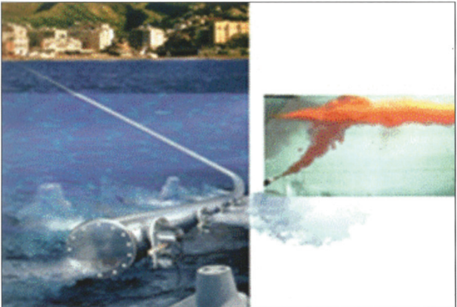
Figure 18: Setup and Dilution Mechanism of an Effective Submarine Outfall
