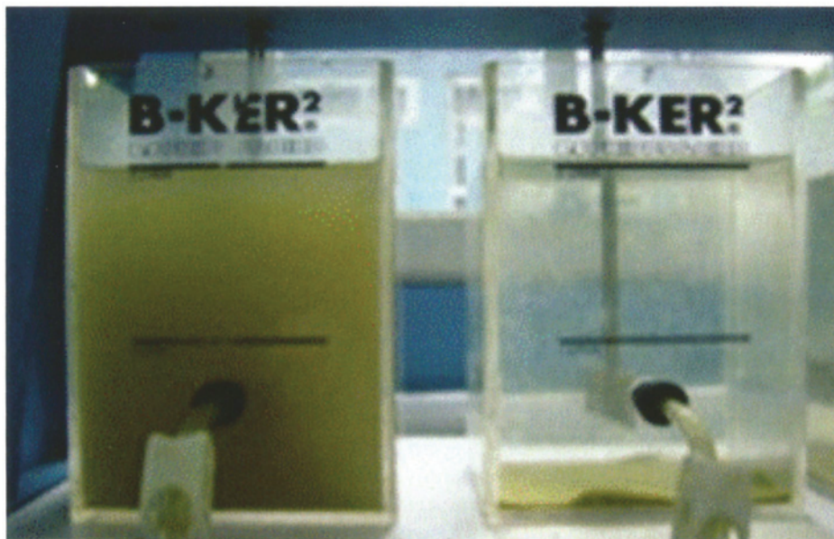
Figure 14: Bench-Scale CEPT and Conventional Primary Treatment Effluents, Source: Prof. Harlemann, MIT (2004)
