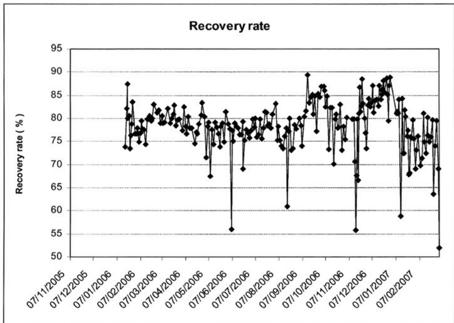
Figure 6: Evolution of the water recovery rate through the grey water treatment unit from January 2006 to March 2007 (Doullami and Lasserre 2007)
