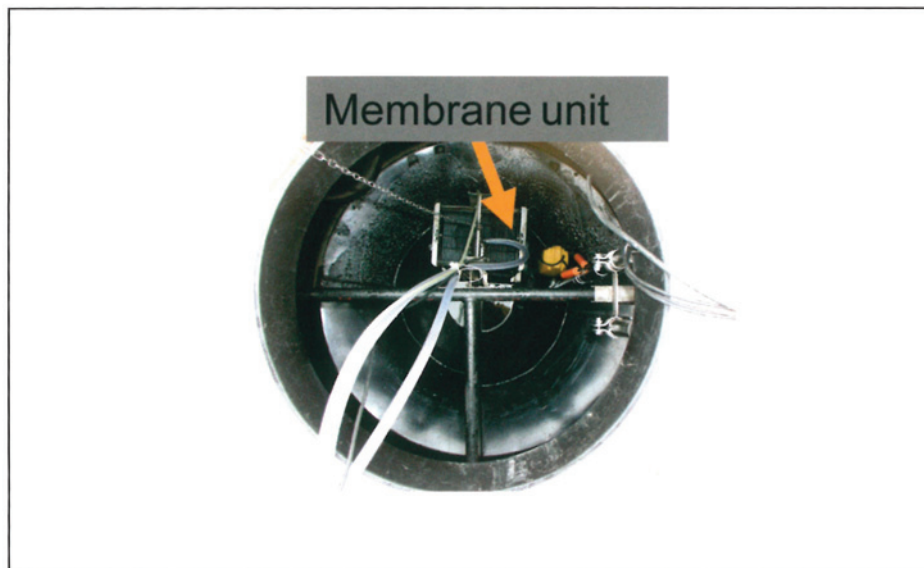
Figure 4: Upgrading of a low-tech small wwtp to a high-tech MBR system by introducing a membrane module plus aeration, Dorgeloh and Defrain (2006).
