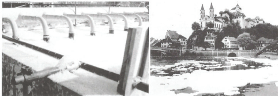
Figure 6: Excessive foaming in an aeration tank (left) and in receiving waters (right) due to nonbiodegradable detergents (branched alkylbenzene sulfonates). Pictures taken around 1964 before the introduction of LAS (archive Eawag)
