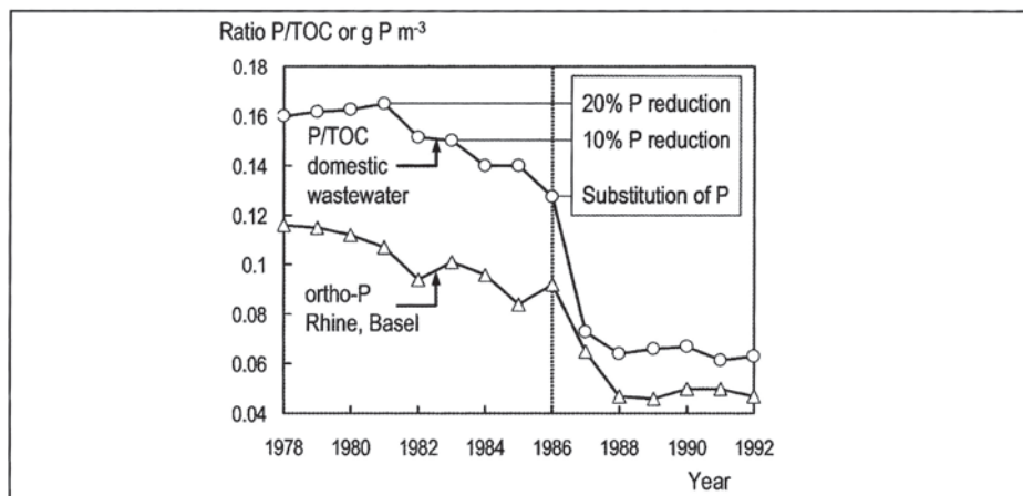
Figure 9: Typical ratio of Phosphorus to TOC in primary effluent of a domestic wastewater treatment plant in Switzerland as a function of successive phosphate substitution in detergents (Siegrist and Boller, 1999). Observed concentration of ortho-P in the river Rhine in Basel (data NADUF, BUWAL, adapted)
