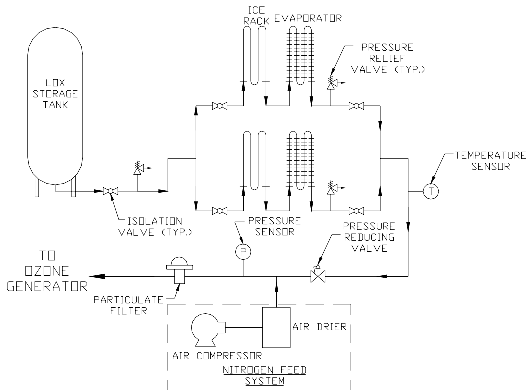
Figure 2.2 – Liquid Oxygen (LOX) Feed System Schematic
