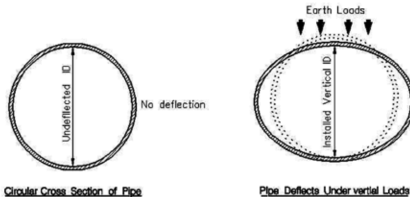
Figure 17: Pipe deflection
