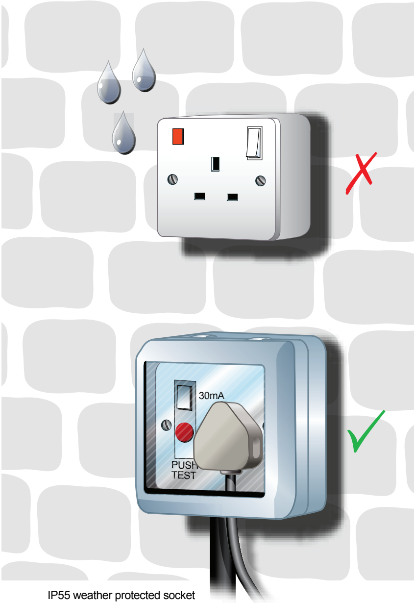
IP55 weather protected socket outlet with 30mA RCD
