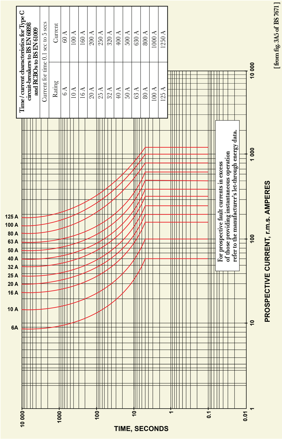
A6(c) Time-current characteristic of Type C MCBs
