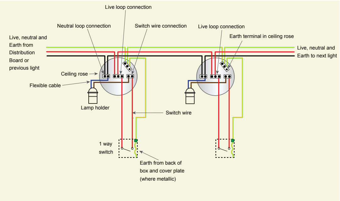
Standard lighting Circuit arrangement
