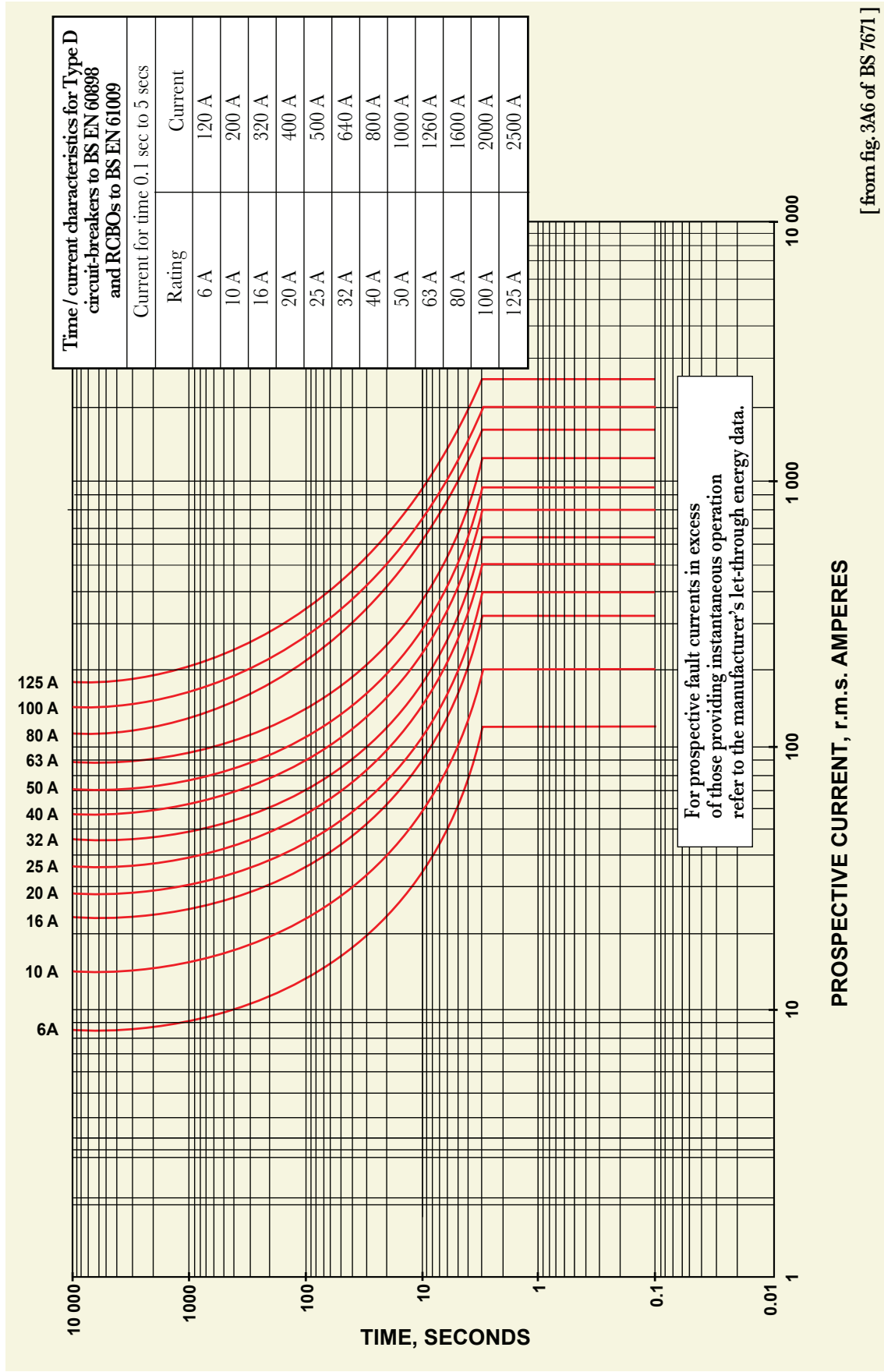
A6(d) Time-current characteristic of Type D MCBs
