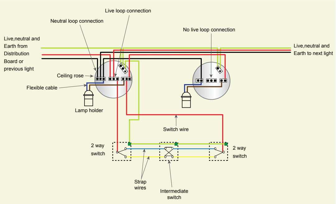
Two way switch lighting Circuit arrangement
