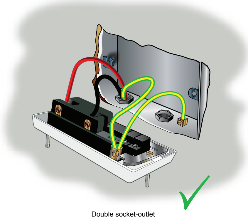
Double socket-outlet
