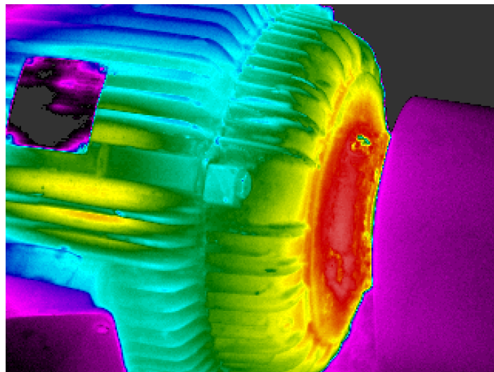
Figure 72 Thermal imaging
