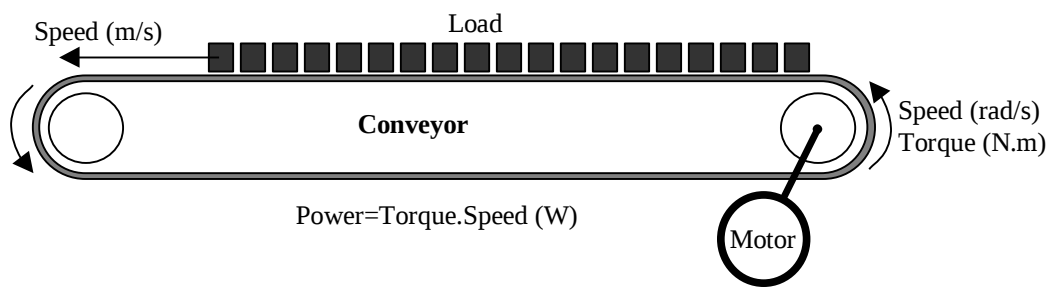
Figure 49 Power required by a conveyor.
