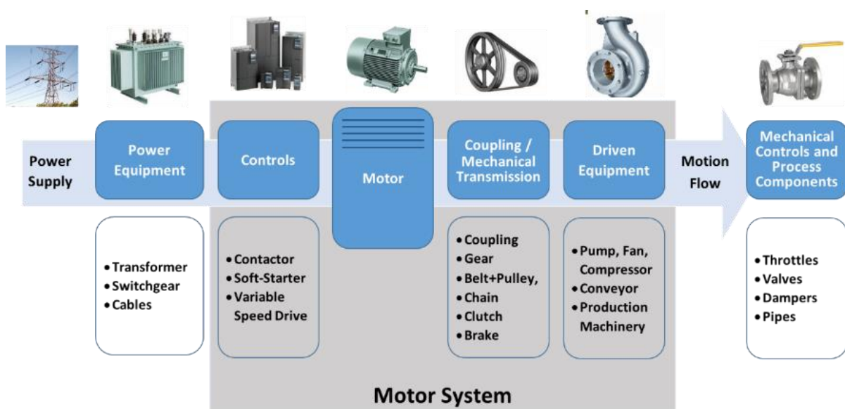
Figure 22 Motor system
