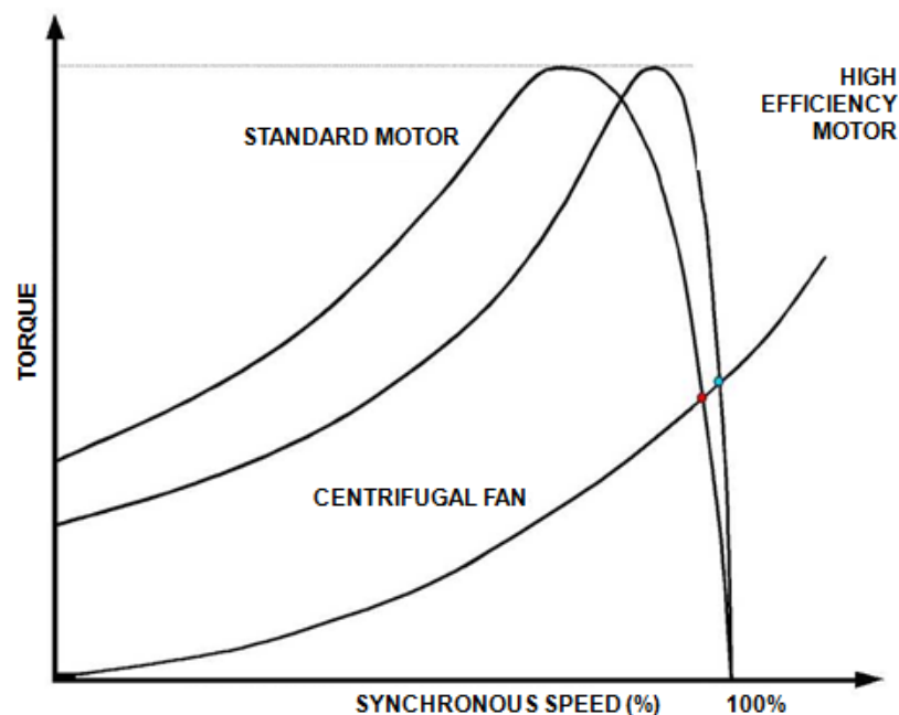
Figure 69 Standard and high efficiency motor Torque speed-curves
