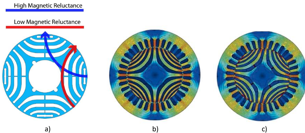
Figure 18. Synchronous Reluctance Motor Operating Principle a) rotor areas of high and low reluctance b) the rotor is aligned with the magnetic field so no torque is produced; c) the rotor is not aligned with the magnetic field and (counter-clockwise) torque is produced (Source: Oemer and ABB)
