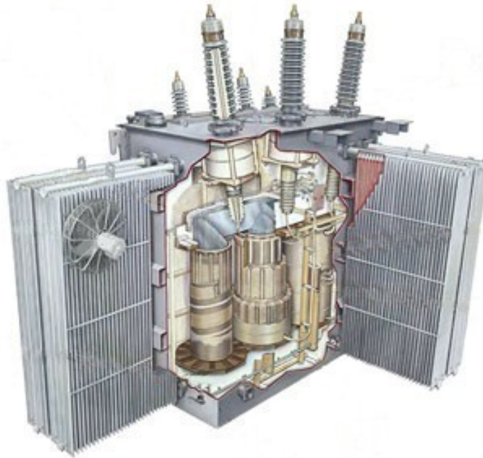
Figure 2 - Transformer Cutaway Representation
