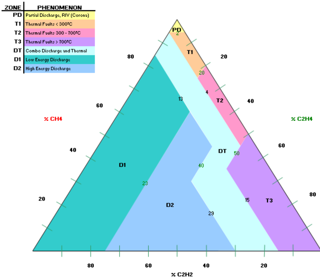
Figure 7 – DUVAL TRIANGLE
