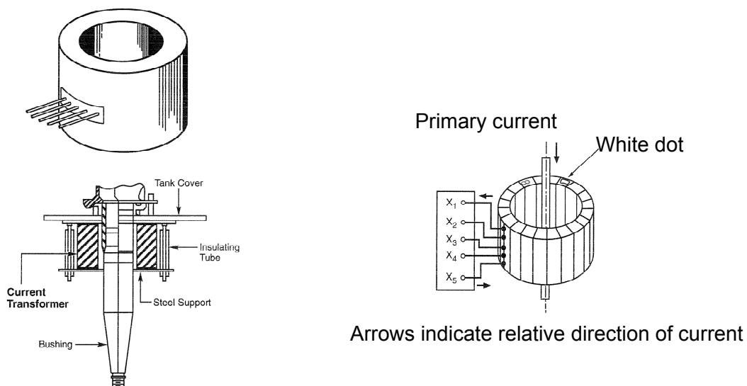
Figure 15: Multi-Ratio Bushing Type Current Transformer Typical of the type found on Transformers and Oil Circuit Breakers
