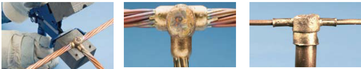
Figure 3: Examples of Cadwelded connections
