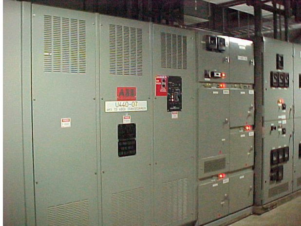
Figure 4: Dry-Type Load Center
