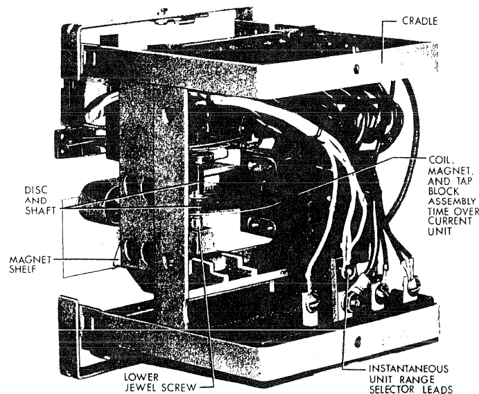
(Rear View)
