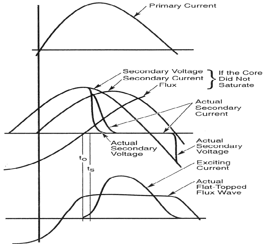
Figure 18: Effect of excessive burden on a Current Transformer
