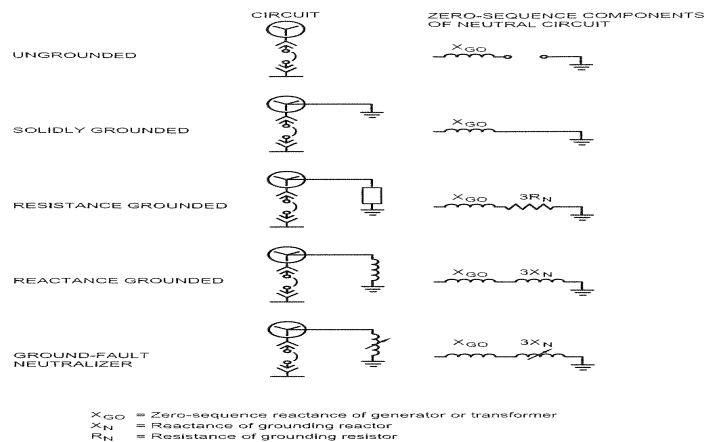
Figure 1: Equivalent diagrams for ungrounded and grounded systems
