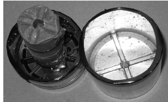
Figure 4: Can and Capacitive Element
