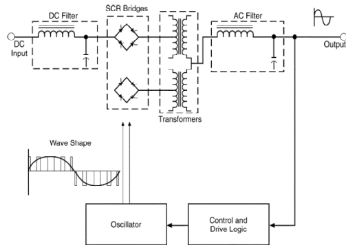
Figure 6: PWM Inverter Diagram
