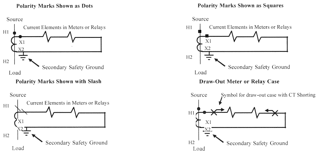
Figure 9: Examples of polarity markings for CT's
