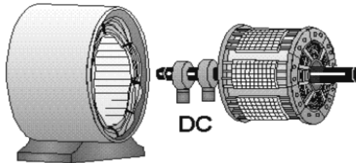
Figure 3: Synchronous Motor Illustration
