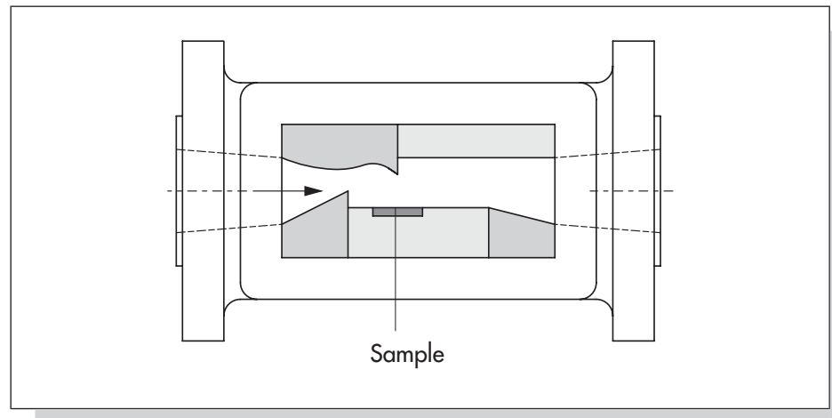
Fig. 11: Cavitation chamber
