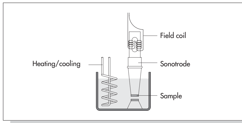
Fig. 12: Magnetostrictive transducer
