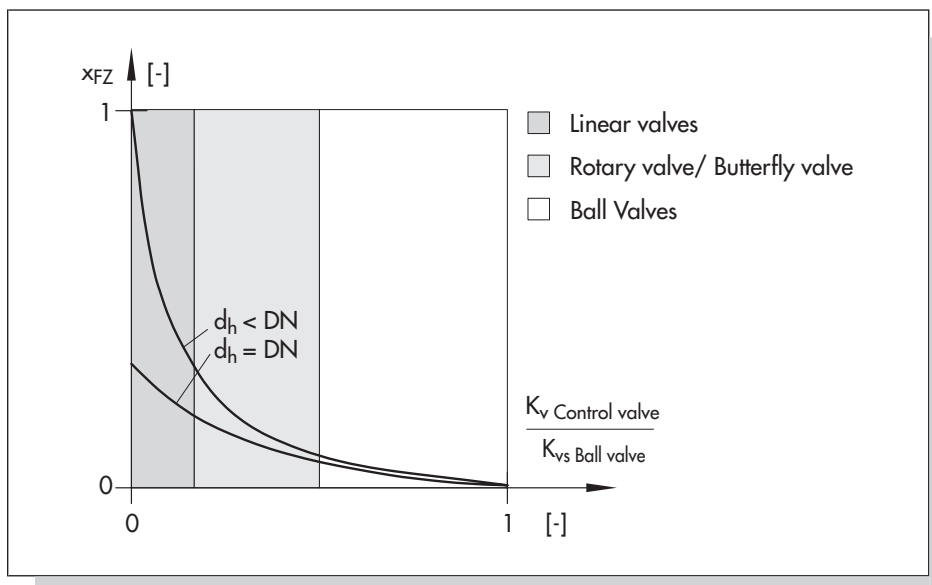
Fig. 15: Control valve operating range without cavitation
