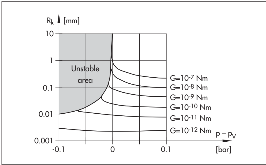
Fig. 3: Critical nucleus radius with varying gas concentrations
