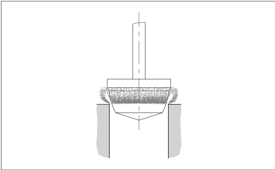
Fig. 20: Areas of a parabolic plug at risk from erosion
