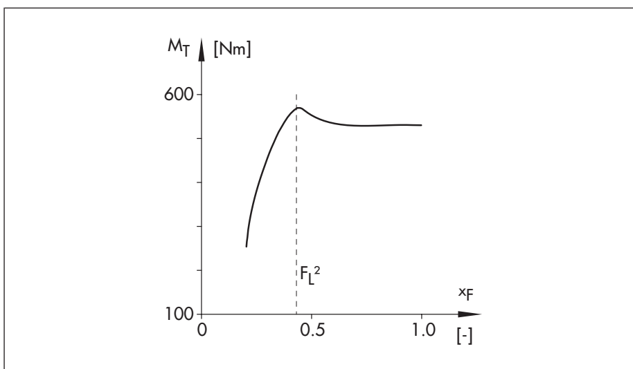
Fig. 26: Course of torque in a butterfly valve
