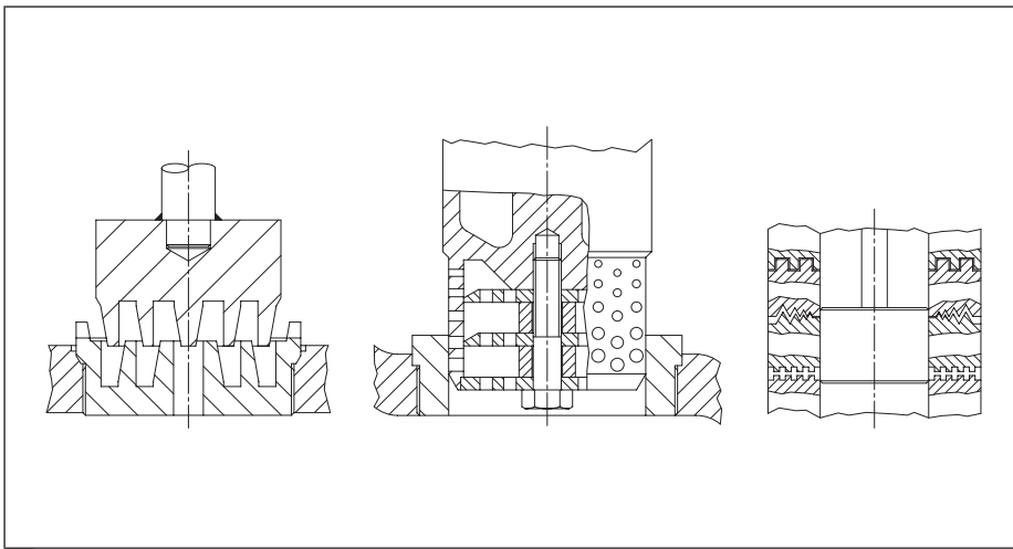
Fig. 19: Plug designs
