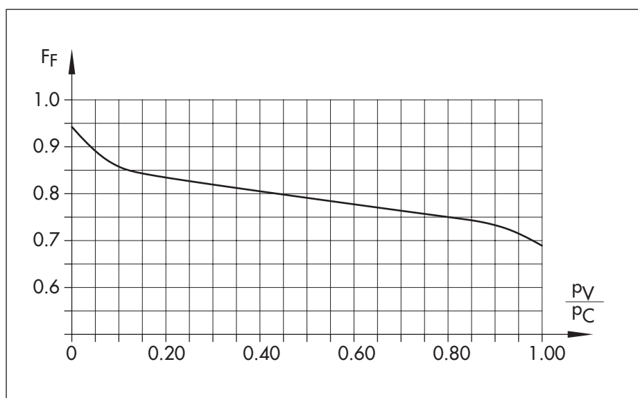
Fig. 25: F_F factor used to determine the critical pressure ratio
