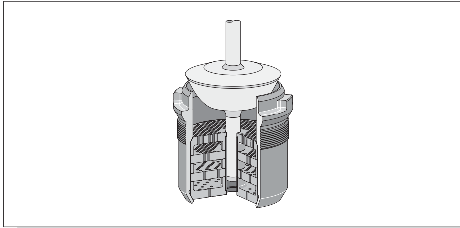
Fig. 16: AC trim system (SAMSON)
