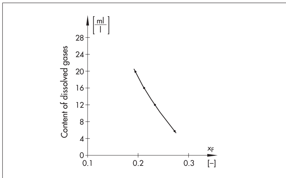
Fig. 7: Relation between the pressure ratio x_F and the gas content
