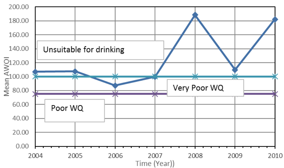
Fig. 4 Variation of annual mean values of WQI in Euphrates River within Al-Anbar province during 2004-2010.
