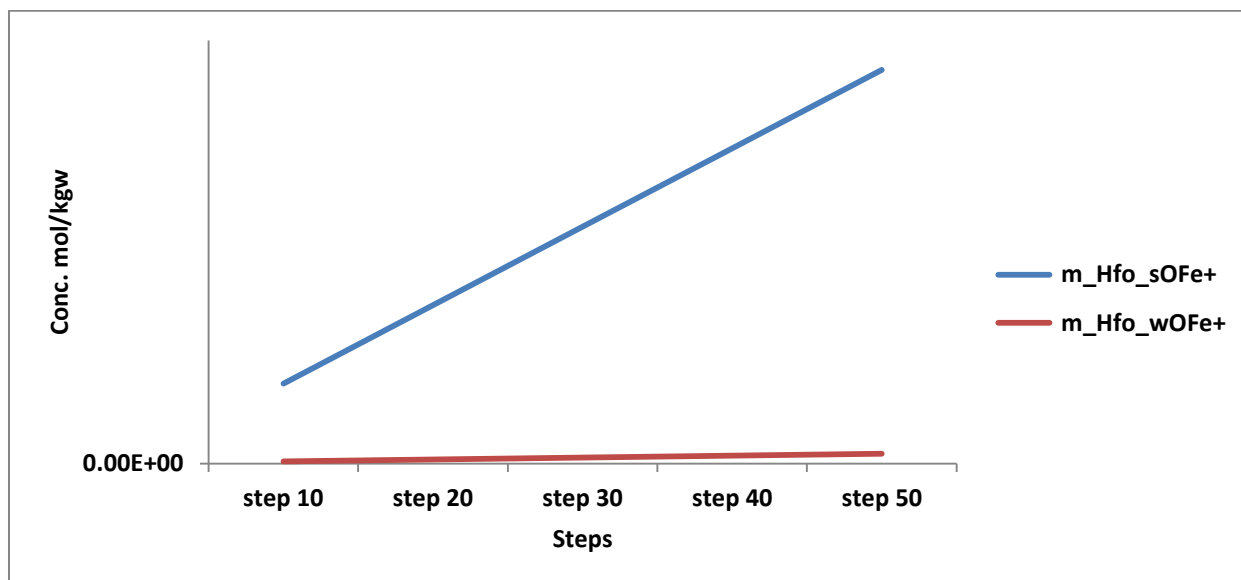
Figure 6.13: sorption of iron in cell no 6 by of hydrous ferric oxide.
