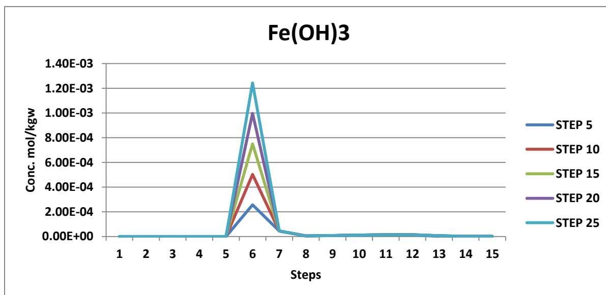
Figure 6.8: Concentration of Fe (OH) 3 in cells 1-15 at steps 5-25.
