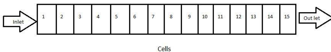
Figure 4.16: One dimensional flow in PHREEQC
