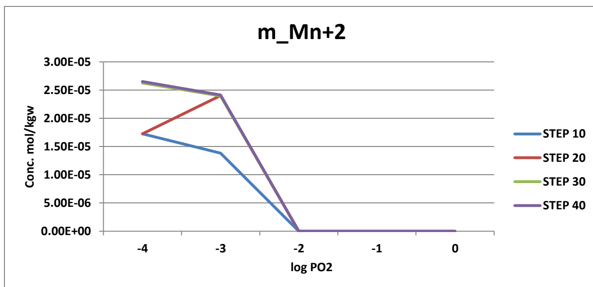
Figure 4.10: Concentration of manganese at different log PO2 levels in cell no 6 at steps 10-40
