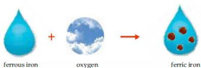
Figure 2.1: Oxidation of ferrous iron into ferric iron under influence of oxygen (Teunissen 2007)
