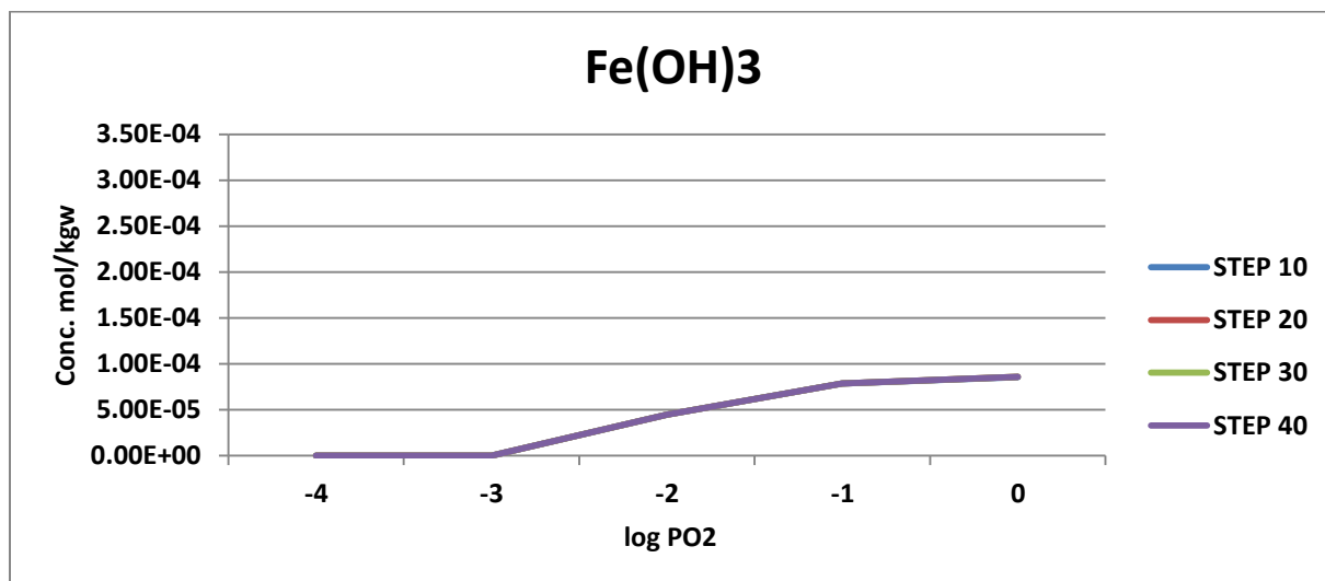
Figure 4.13: Concentration of \text{Fe}(\text{OH})_3 at different log PO 2 levels in cell no 6 at steps 10-40.
