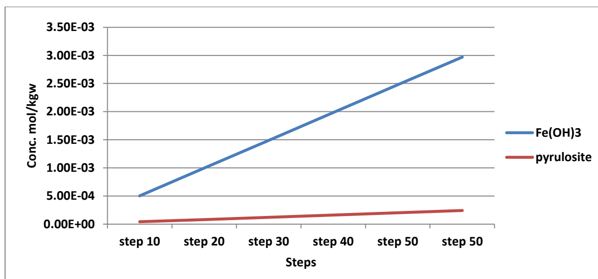
Figure 6.10: Concentration of \text{Fe(OH)}_3 and pyrolusite in cell no 6.
