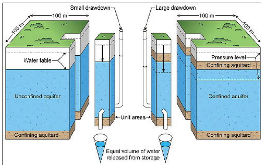
Figure 8 Larger drawdown in confined aquifer compared to unconfined aquifer (Connected Waters Initiative 2013)
