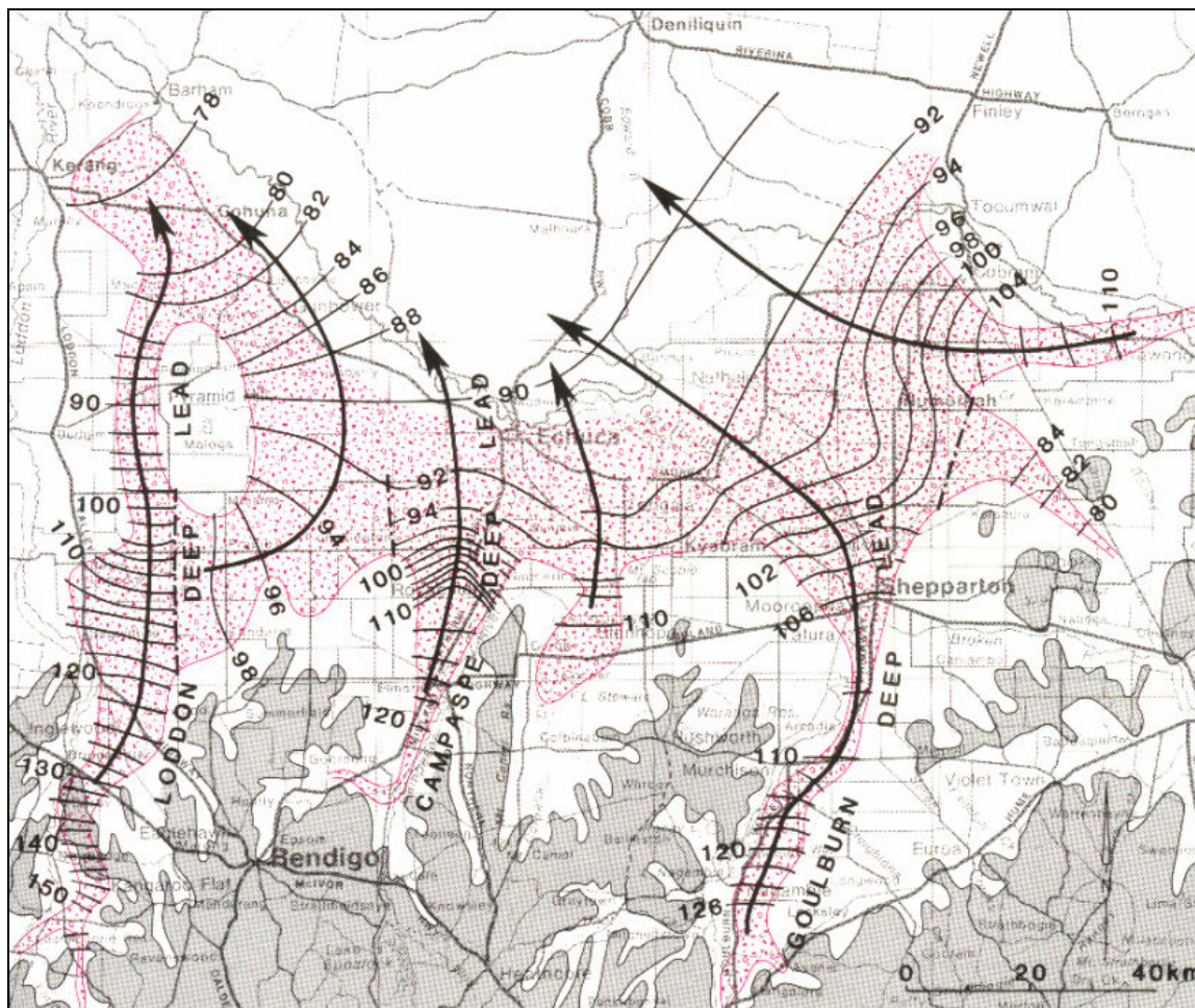
Figure 24: Potentiometric surface of the deep lead system of Northern Victoria – August 1981 illustrating northward groundwater flow (Macumber, 1991)
