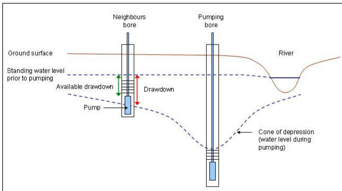
Figure 18: Pumping interference to neighbouring bore and stream
