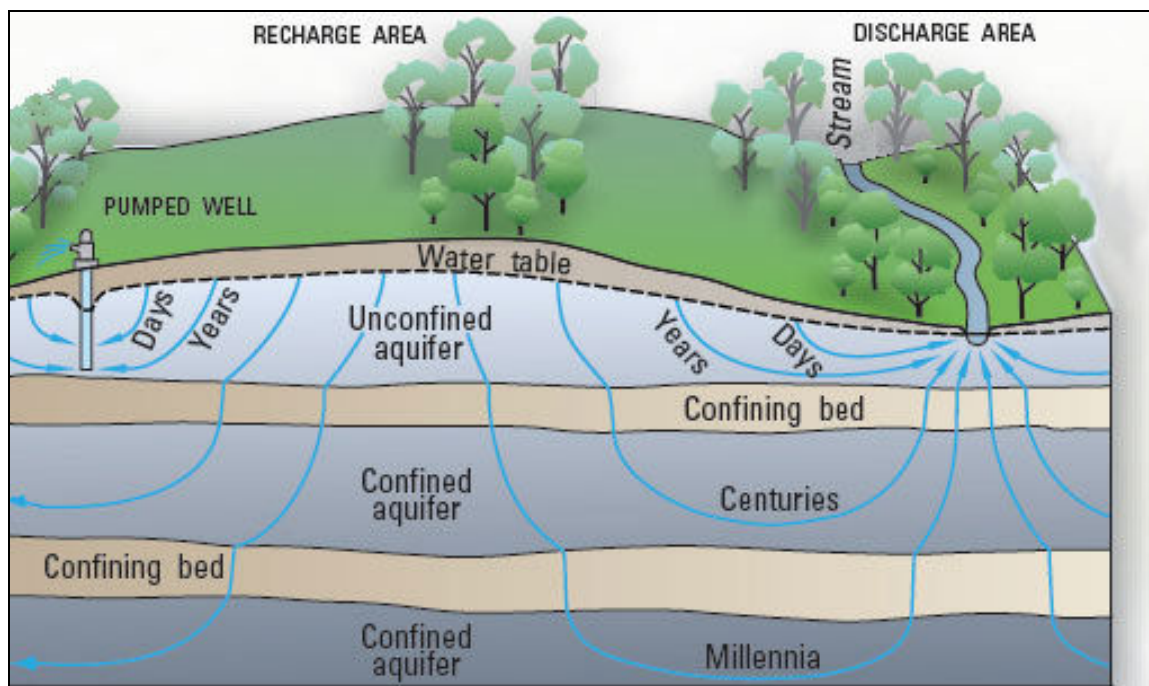
Figure 9 Groundwater flow (USGS 2015)
