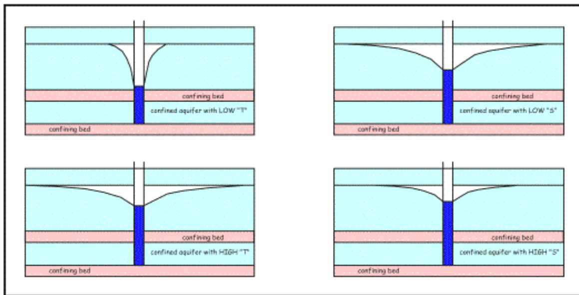
Figure 16 Cone of depression for various confined aquifer characteristics (modified from Freeze and Cherry 1979 by Utah Division of Water Rights, date unknown)
