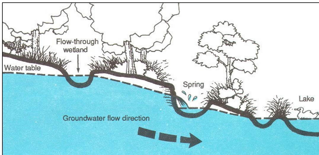
Figure 12 Spring occurrence (Raymond 1988)
