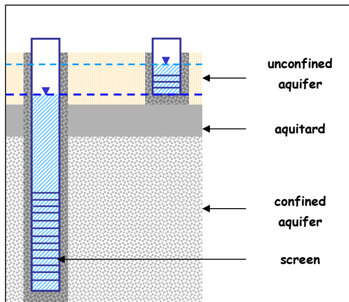
Figure 21 Nested monitoring bores in cross-section
