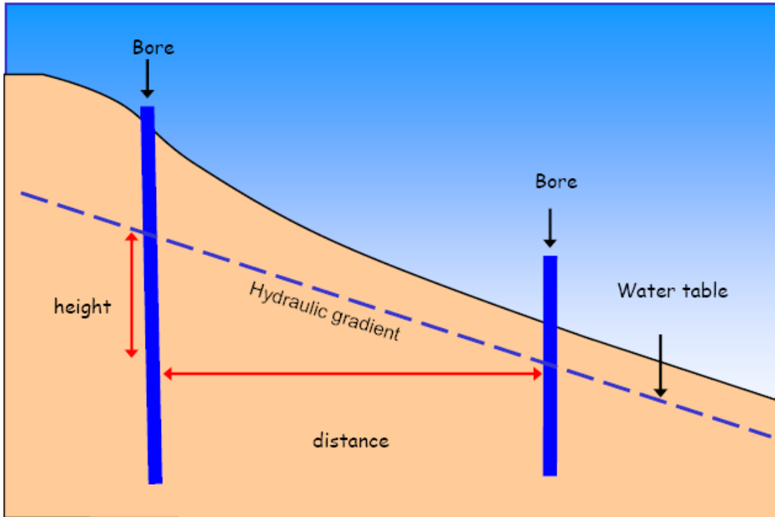
Figure 6: Hydraulic gradient slope between two bores
