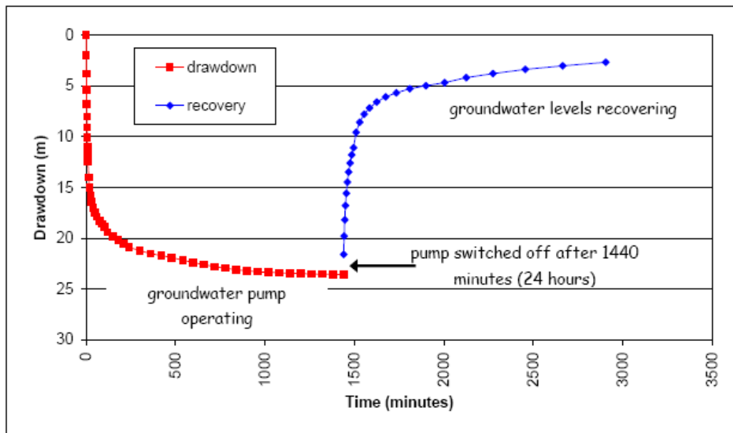
Figure 15 Pumping test time-drawdown data
