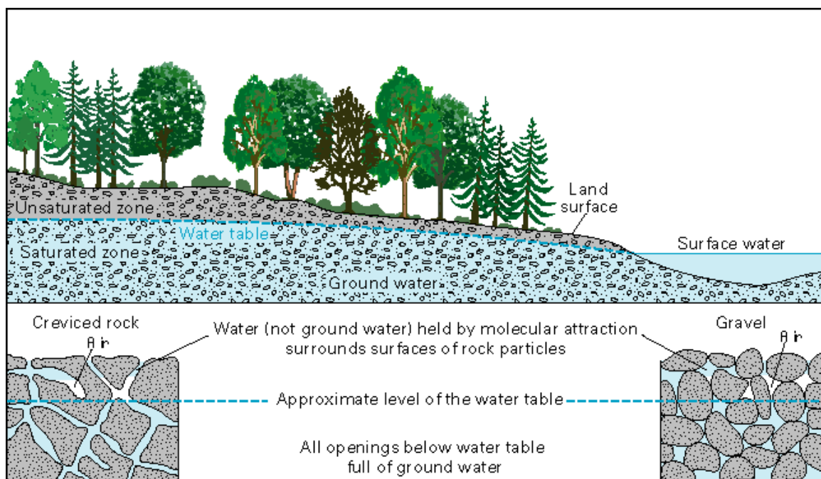
Figure 2 Groundwater occurrence (Ghost Watershed Alliance Society 2015)
