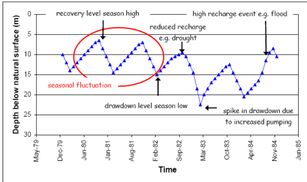
Figure 20 Example of a groundwater hydrograph
