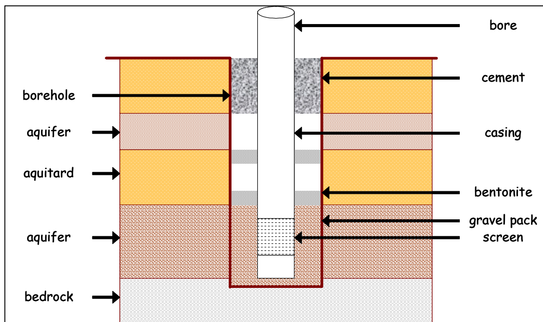
Figure 17: Example Bore Construction
