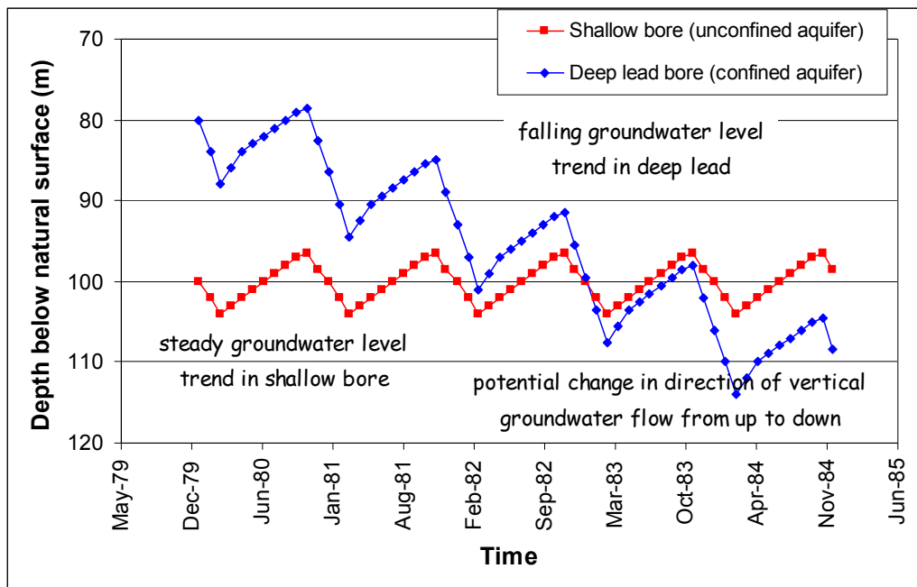
Figure 22 Example of a hydrograph for nested monitoring bores
