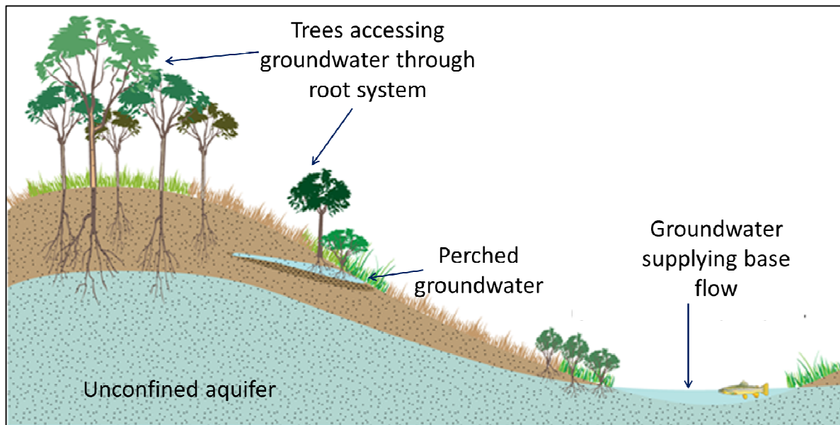
Figure 14 Examples of groundwater dependent ecosystems (modified from Texas A&M University 2013)
