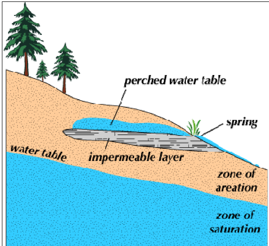
Figure 4 Perched aquifer (Arizona State University, date unknown)
