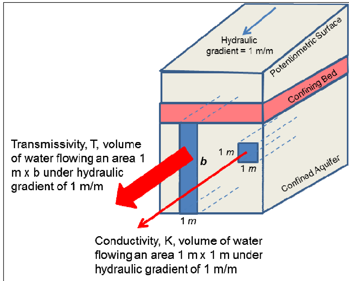
Figure 7 Aquifer transmissivity and hydraulic conductivity (McKinney, 2015)
