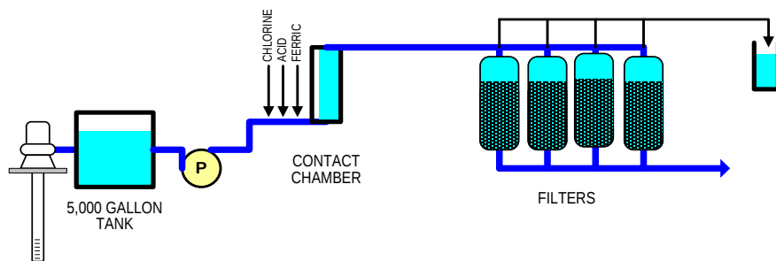
FIGURE 1: CHLORINE/ACID/FERRIC/CONTACT TANK
