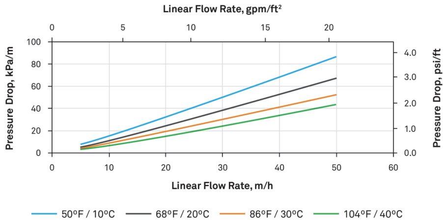
Figure 3 – Pressure drop
