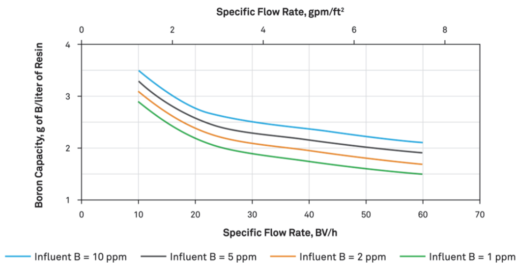
Figure 1: Boron capacity vs. influent boron concentration and service flow rate
