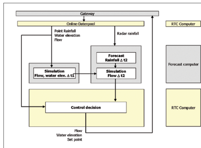
Figure 10: Dataflow for the integrated control system
