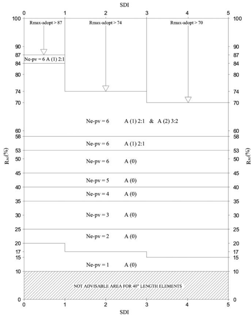
Fig. 2. RO elements per pressure vessel.
