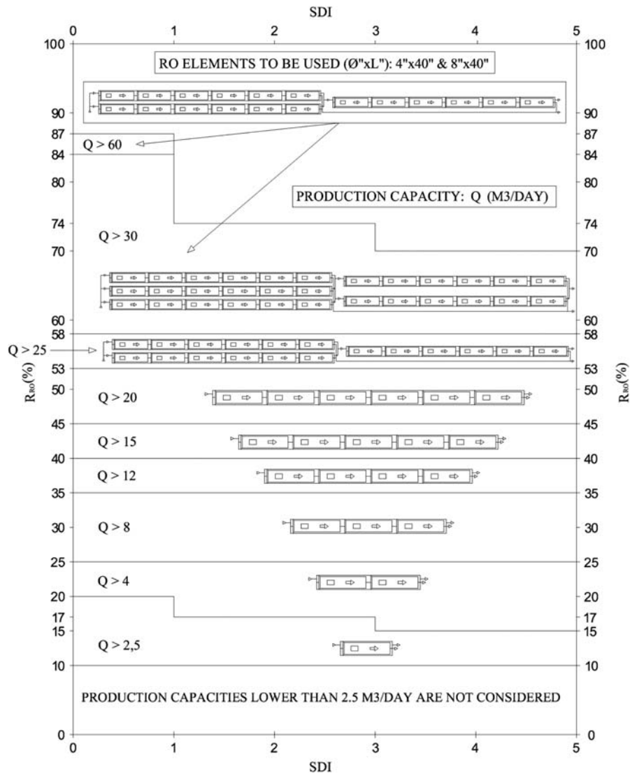
Fig. 3. Basic arrangement and production capacity distribution.
