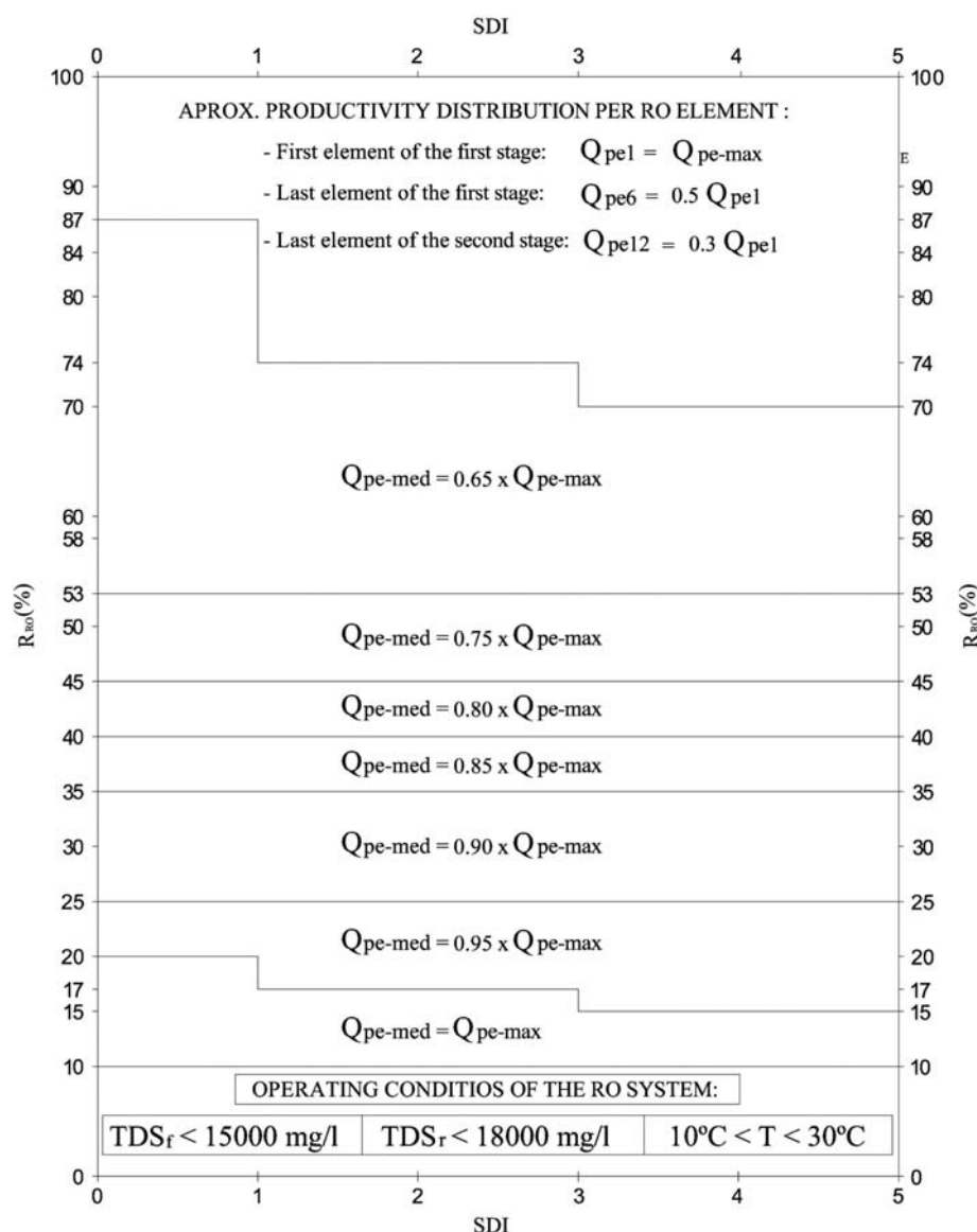
Fig. 5. Average product flow per RO element.
