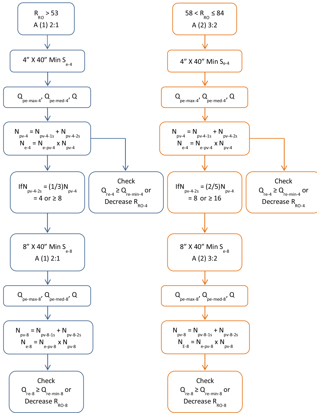
Fig. 7. RO system checks and settings ( R_{RO} > 53\% ).
