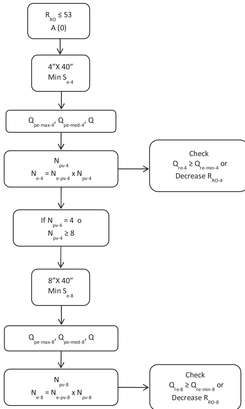
Fig. 6. RO system checks and settings ( R_{RO} \leq 53\% ).
