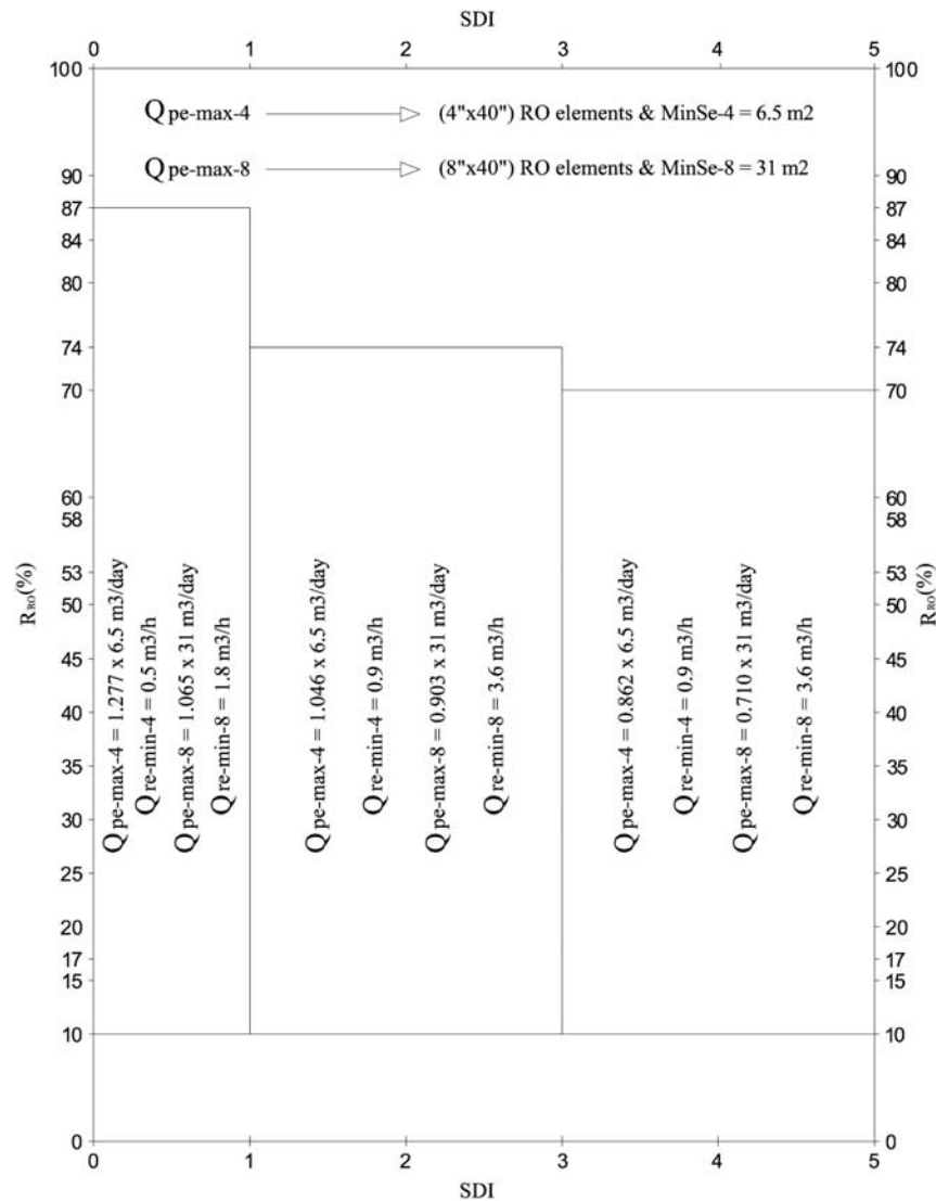
Fig. 4. Maximum product flow and minimum reject flow per RO element.
