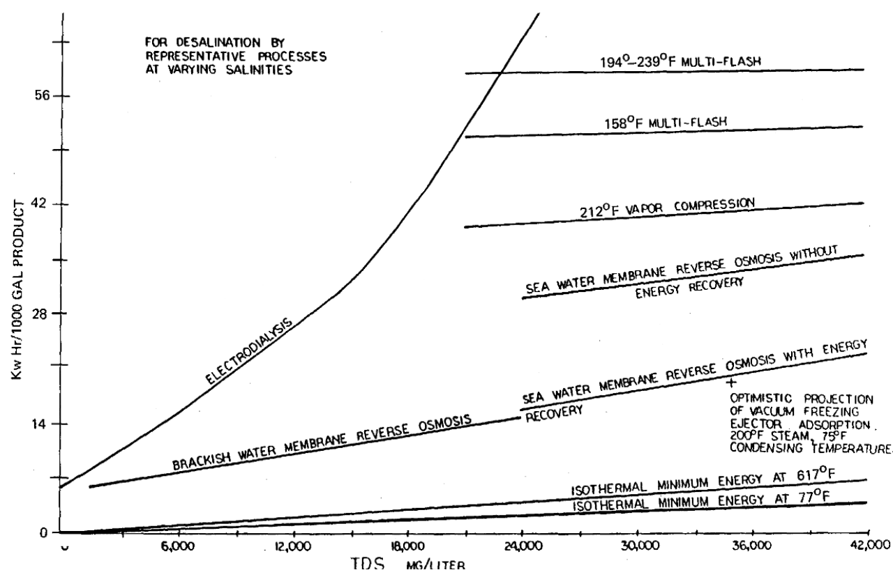
Figure 3-3 Energy Consumption
