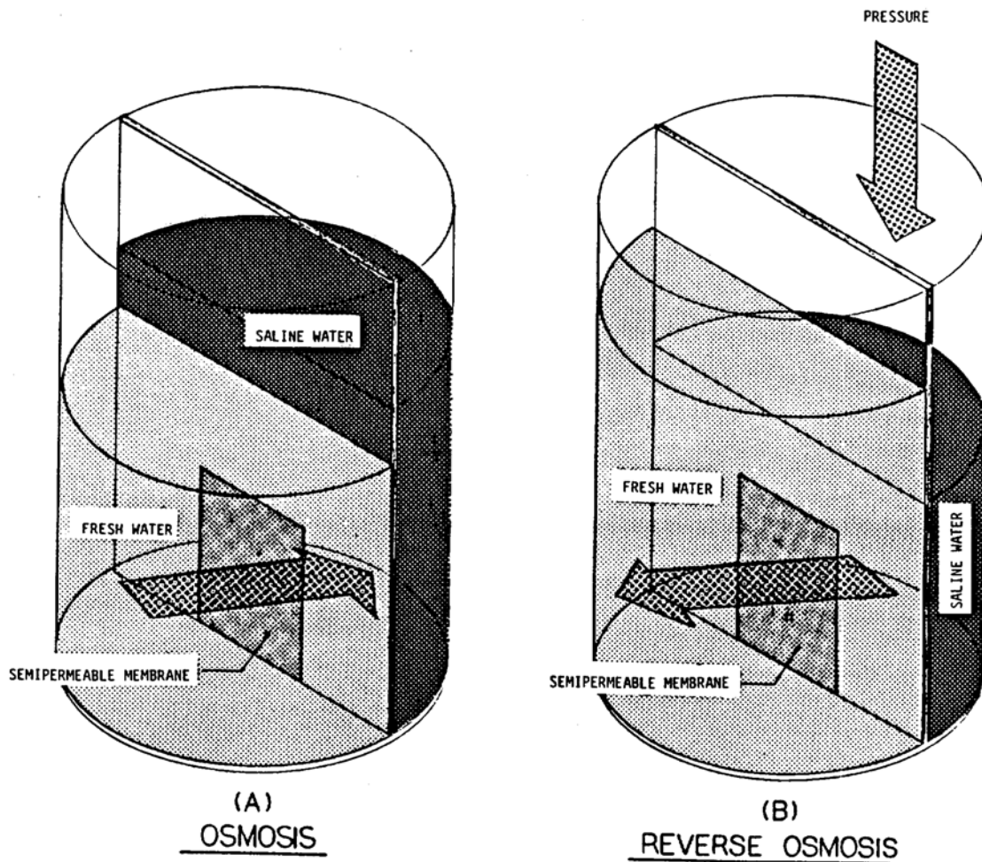
Figure 4-2 Reverse osmosis principles
