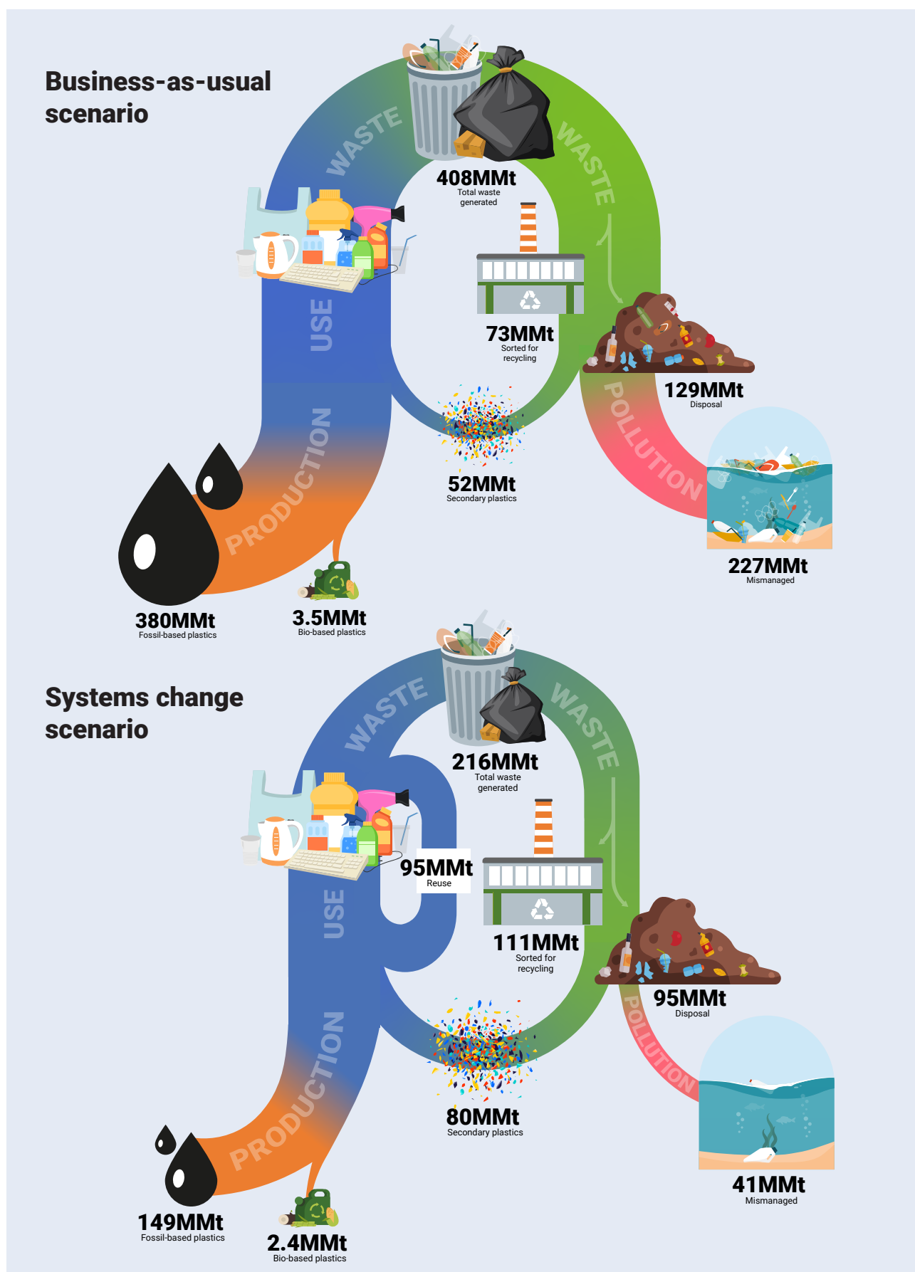
Figure 9: Top: Modelled short-lived plastic flows in 2040 under a business-as-usual scenario. Bottom: Modelled short-lived plastic flows in 2040 under a systems change scenario to deliver the necessary market transformation.
