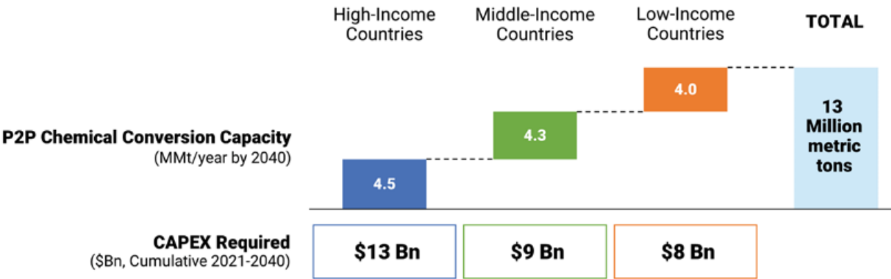
Figure 14: Chemical conversion capacity in 2040 (MMt/year) by region.
