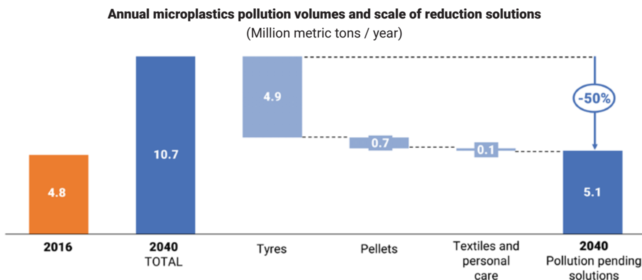
Figure 16: Microplastic pollution under BAU and reduction from four sources under the systems change scenario in 2040.
