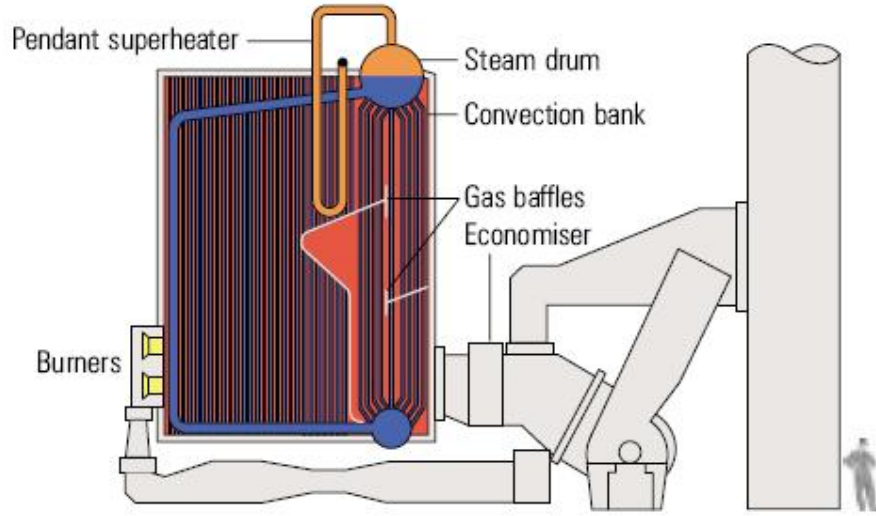
Fig. 3.3.1 Water-tube boiler
