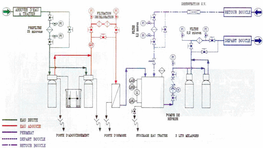
Plant for desalination of sea water using reverse osmosis (doc. CFM)
