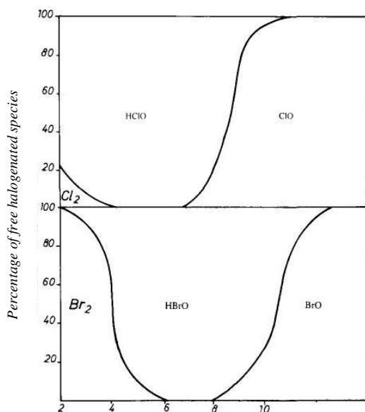
Chemical species encountered in oxidizing halogen solutions at 20 - 25 °C.
