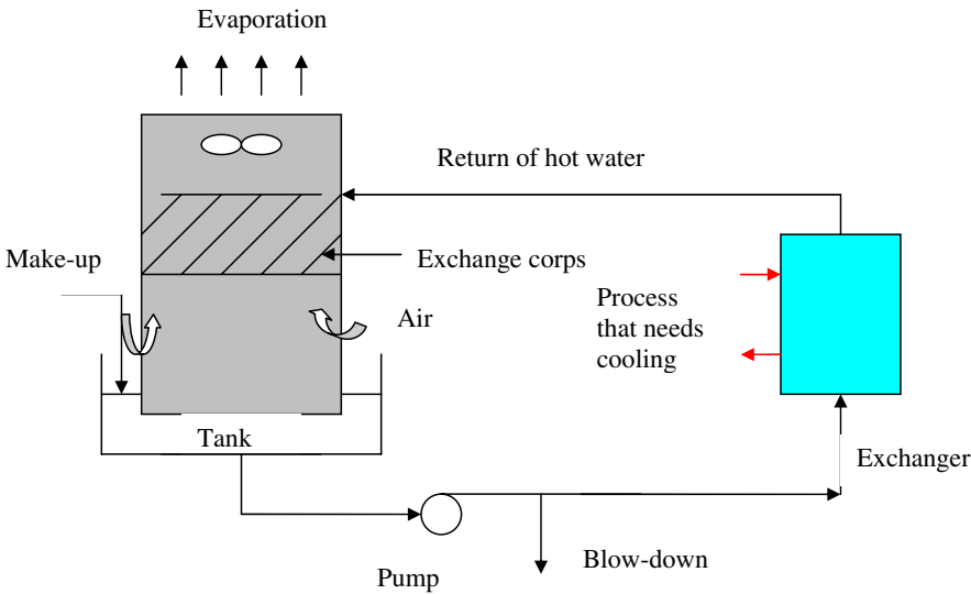
Simplified diagram of an open recirculating circuit
