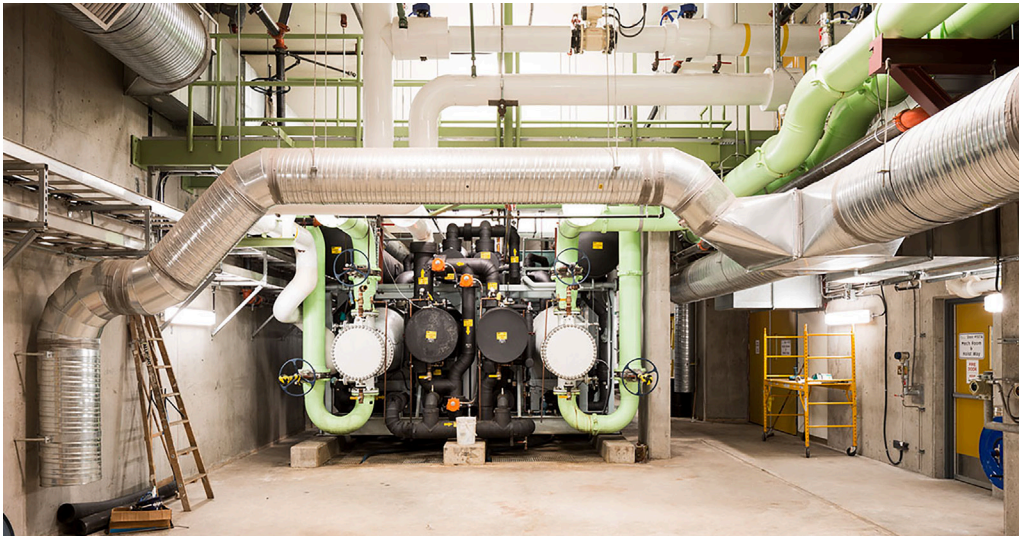
Figure 14.9 A large scale heat pump (~4 MW) extracts heat directly from screened raw wastewater to serve the Southeast False Creek District (courtesy city of Cancouver).
