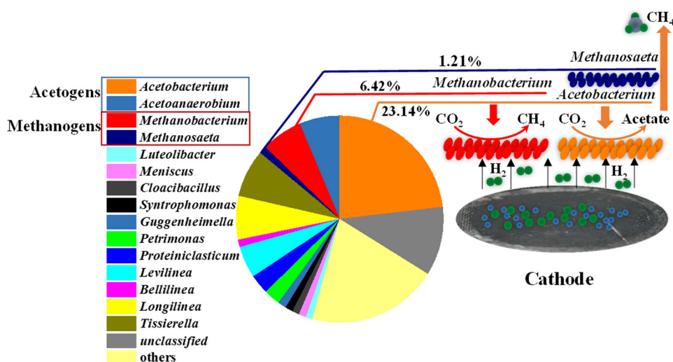
Figure 13.2 Putative pathways of cathodic methanogenesis (Cai et al. , 2016b).
