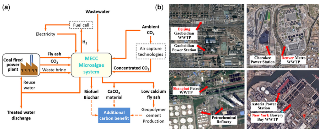
Figure 6.7 (a) schematic of the mutual benefits between an MECC equipped water resource recovery facility (WRRF) and a CO 2 point emission source. (b) example co-locations of CO 2 point sources and WRRFs enable complementary CCU in Beijing, Shanghai, New York city, and Denver (Lu et al. , 2015, 2018).
