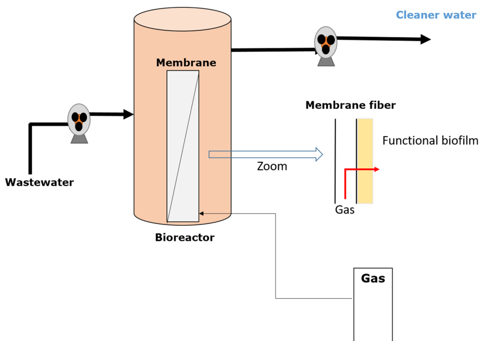
Figure 11.3 Membrane biofilm reactor (MBfR) for wastewater treatment.
