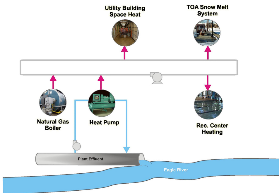
Figure 17.5 Avon, CO, wastewater heat recovery schematic. Image courtesy of Jennifer Strehler/CDM Smith.
