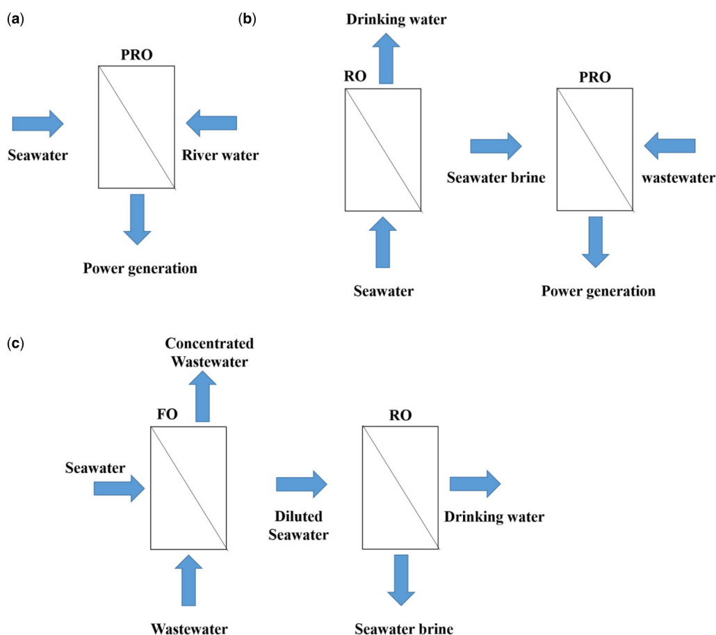
Figure 11.5 (a) System configuration of river-to-sea PRO system for power generation, (b) SWRO-PRO system for desalination and power generation and (c) FO and RO hybrid system for desalination and wastewater concentration.
