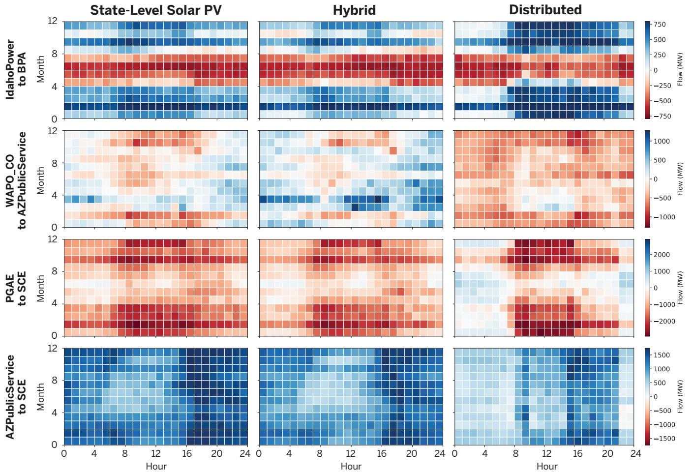
FIGURE 23 12x24 Flow Heat Maps
