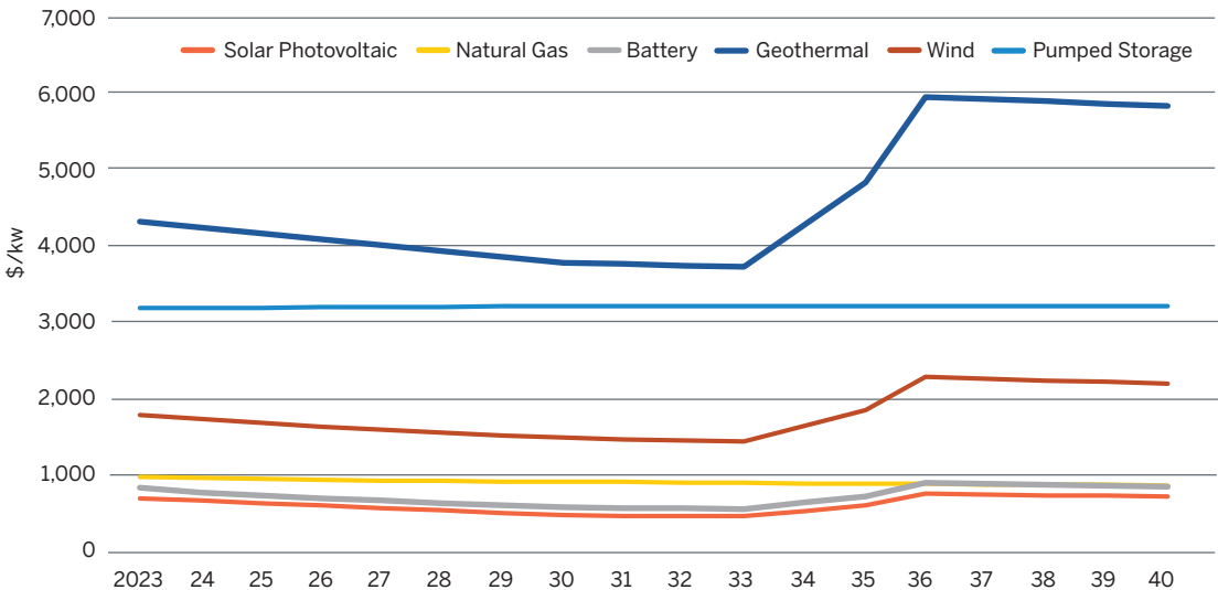
FIGURE 6 Average Overnight Build Costs by Resource Class over the Study Horizon
