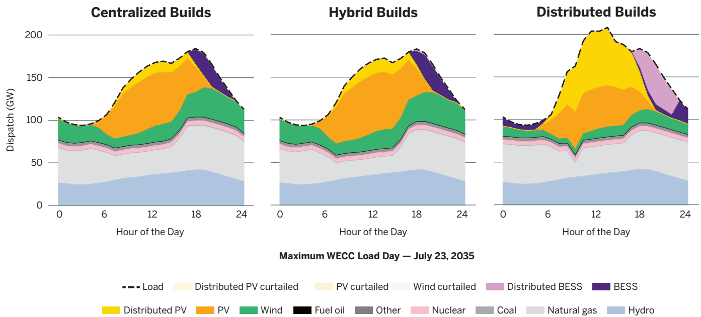
FIGURE 15 Maximum WECC Load Day Dispatch
