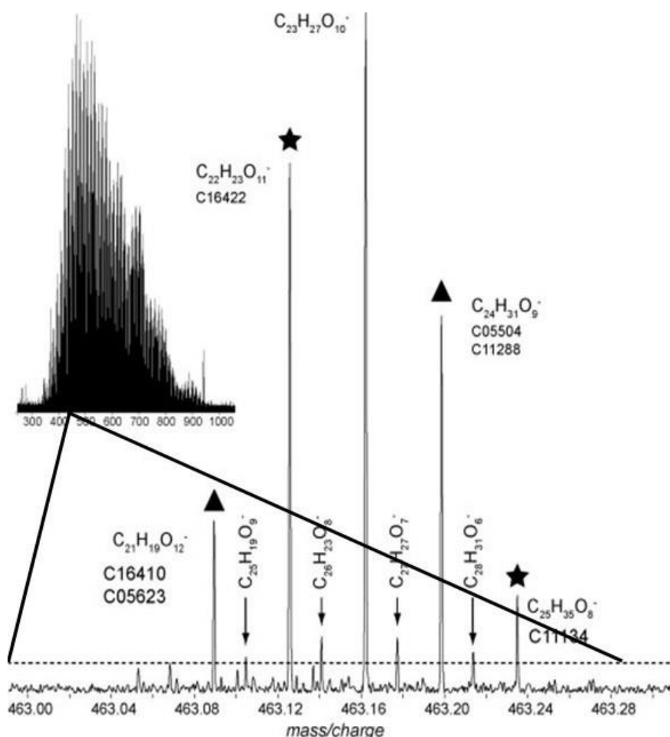
Figure 13 - Negative ion mode ESI FT-ICR MS mass spectra of DOC from whole groundwater illustrating its compositional complexity. Reproduced from Longnecker and Kujawinski (2011) with permission.
