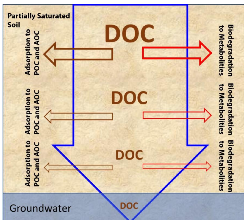
Figure 7 – DOC concentration decreases as water infiltrates from land surface to underlying groundwater due to adsorption to POC and AOC as well as biodegradation to metabolites. Mechanisms that decrease DOC concentrations as water infiltrates are: adsorption of DOC to POC, AOC and mineral surfaces; and, biodegradation to metabolites, including DIC. The weights of the arrows illustrate that adsorption may be less significant with depth because the remaining DOC is more hydrophilic with depth, and biodegradation may decrease with depth as the remaining DOC becomes less bioavailable (more resistant to biodegradation) (Mackay, 2022).
