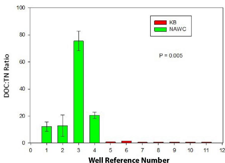
Figure 19 - DOC:TN molar ratios in groundwater suggesting greater DOC bioavailability at NAWC relative to the KB site.
