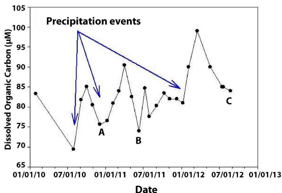
Figure 18 - Concentrations of DOC in groundwater from a single well over time in the Piedmont of South Carolina, USA. DOC concentrations increase following precipitation events and then subsequently decline due to sorption and biodegradation processes. Reproduced from Chapelle and others (2016), with permission.
