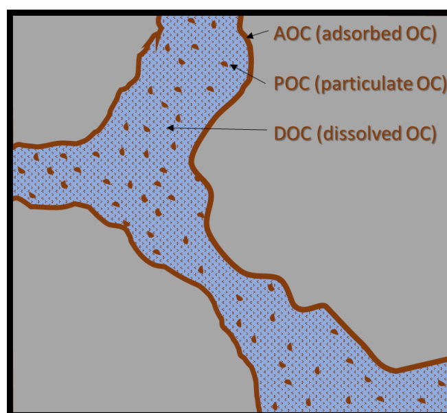
Figure 2 - Occurrence of AOC, POC and DOC in groundwater in a pore between grains or fracture walls within an aquifer. This is not a scale drawing, but meant to illustrate that typically there is a lot more organic carbon in AOC and POC than in DOC. AOC may not coat all particle surfaces nor coat them uniformly, as is illustrated here. Though not indicated, AOC may sometimes remobilize into the porewater, which increases DOC (Mackay, 2022).
