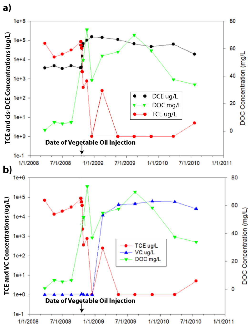
Figure 12 - Concentrations of a) TCE, cis-DCE, and DOC and b) TCE, VC, and DOC at the NAWC site in well BR-36 before and after bioremediation using emulsified vegetable oil.
