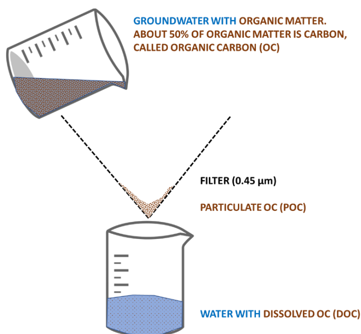
Figure 1 - Organic matter in water is typically about 50 percent carbon and is generally referred to as composed of two fractions, that captured by a 0.45 filter (POC) and that passing the filter – DOC – (Mackay, 2022).
