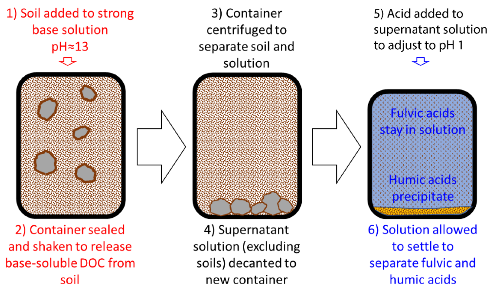
Figure 6 - Illustration of initial steps in characterizing soil organic matter for agricultural purposes. Humic and fulvic acids are extracted from soil by a strong base, then separated by acidification and settling. In the analysis of groundwater, this distinction is less useful since total DOC is generally low (Mackay, 2022).
