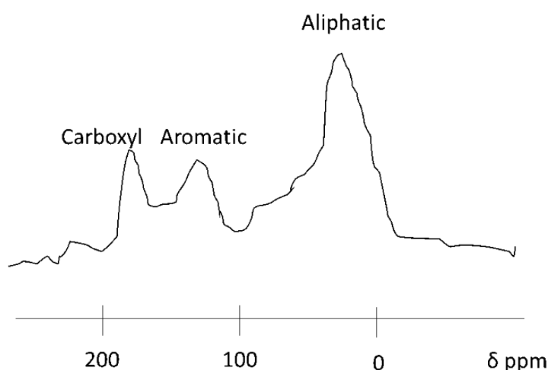
Figure 14 - An example of a ^{13}\text{C} -NMR spectrum showing the approximate relative abundance of carboxyl, aromatic, and aliphatic carbon present in the fulvic acid fraction of DOC. Data are from Aravena and others (2004).
