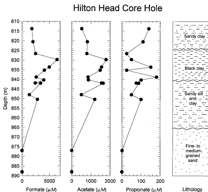
Figure 10 – Data from the Hilton Head core hole showing the relationship between concentrations of dissolved formate, acetate, and propionate in pore water of the permeable zones and confining bed within the Black Creek aquifer system (reprinted from Chapelle and Bradley, 1996, with permission).
