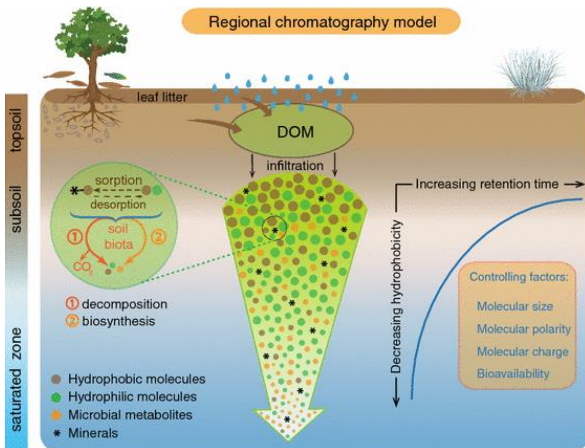
Figure 8 – Regional Chromatography Model - precipitation and surface water leaches dissolved organic matter (DOM) from vegetation and plant litter and percolates through the soil column to the saturated zone. The concentration, composition, and bioavailability of DOC are altered during transport through the soil column by various physicochemical and biological processes, including sorption, desorption, biodegradation, and biosynthesis. Hydrophobic molecules are preferentially partitioned onto soil minerals and have a longer retention time in soils than hydrophilic molecules. The hydrophobicity and retention time of colloids and dissolved molecules in soils are controlled by their size, polarity, charge, and bioavailability. Bioavailable DOC is subjected to microbial decomposition, resulting in a reduction in size and molecular weight. Novel molecules are synthesized by soil microbes, and some of these metabolites enter the DOC reservoir in groundwater. Reprinted with permission from Shen and others (2015).
