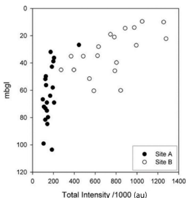
Figure 17 - Changes in total fluorescence with depth in the Penrith Sandstone (site A) and the Sherwood
