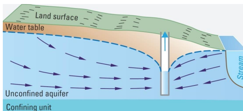
Figure 20 – Cross-sectional view of a pumping well near a river illustrating that water in the well is a mix of water from recharge that infiltrates through the vadose zone and water that seeps from the river into the aquifer (from Konikow and Bredehoeft, 2020).
