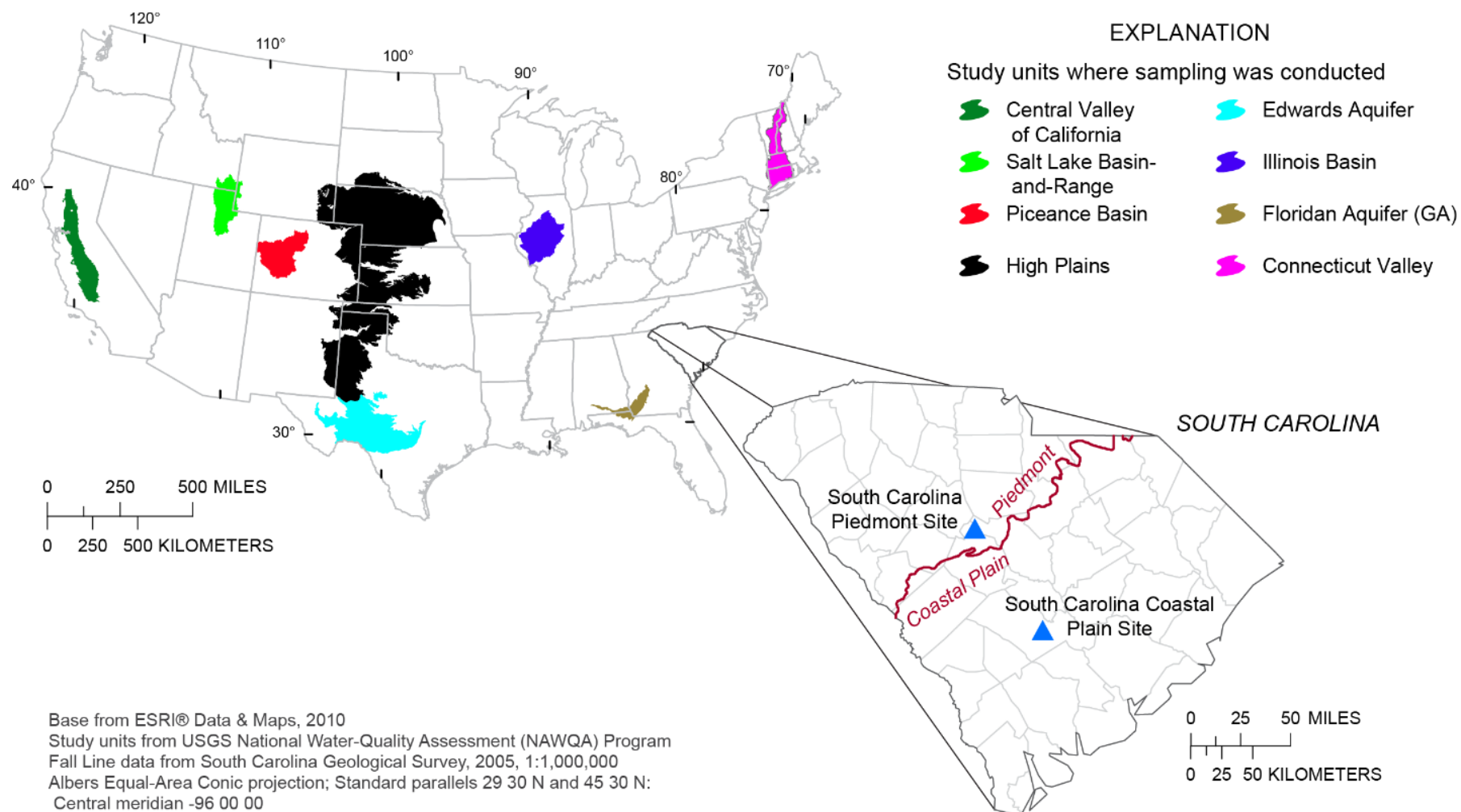
Figure 15 - Locations of the South Carolina (SC) Piedmont and SC Coastal Plain sites and locations of the eight Principal aquifers of the United States. Reprinted from Chapelle and others (2016), with permission.
