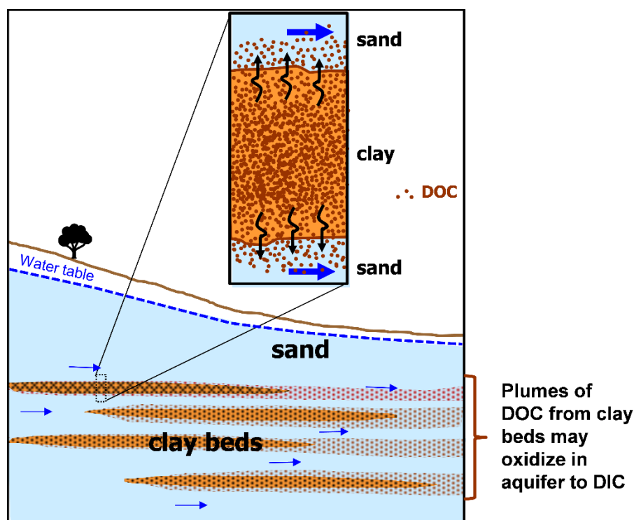
Figure 9 – Low permeability geologic units with almost no active flow (e.g., clay beds) can release old DOC by diffusion (brown dots in inset or shading) to the active flow in the permeable zones (e.g., sands), so the groundwater flowing around the clay beds may contain DOC from the clay beds that may oxidize to DIC along the flow path in the permeable zone. Only a few large clay beds are shown for clarity (Mackay, 2022).
