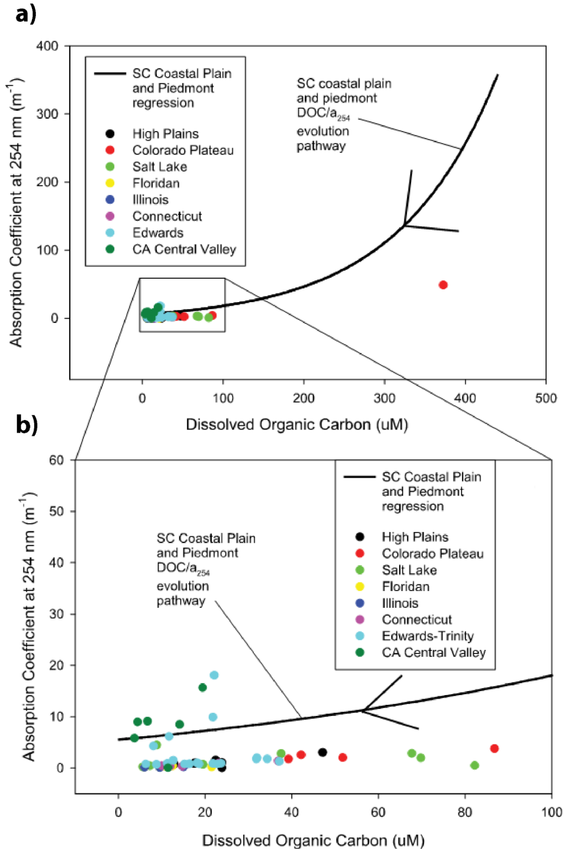
Figure 16 - DOC concentrations and UV absorbance coefficients for eight aquifer systems of the United States plotted against: a) the \text{DOC}/a_{254} evolution pathway exhibited by the SC piedmont and coastal plain aquifers for the 1-450 \mu\text{M} ( \mu\text{mol/L} ) concentration range; and, b) for the 1-100 \mu\text{M} concentration range. Reproduced from Chapelle and others (2016), with permission.
