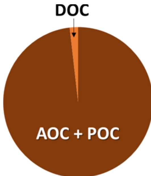
Figure 3 - DOC typically makes up a very small percentage of total organic carbon in a given volume of aquifer material. This illustration is for a clean white beach sand described in the text (Mackay, 2022).
