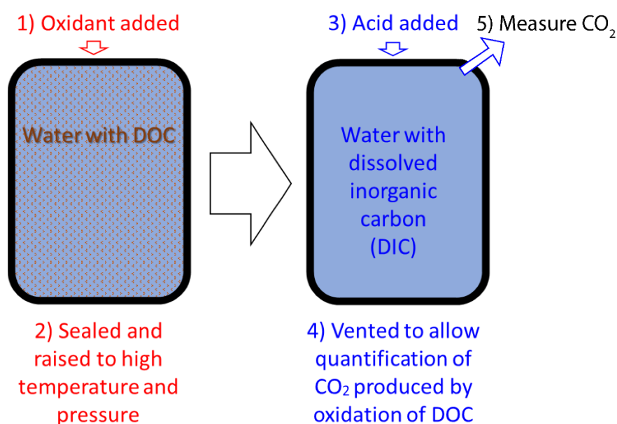
Figure 5 - The steps in quantifying low levels of DOC in water as described in the text. The DOC is oxidized to dissolved inorganic carbon (DIC), then the DIC is converted to dissolved CO 2 by acidification and the CO 2 is vented to a detector capable of quantifying total CO 2 evolved (Mackay, 2022).
