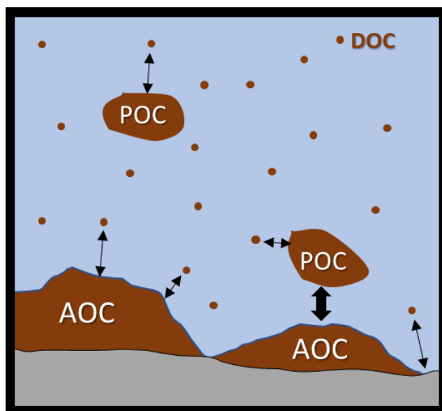
Figure 4 - AOC, POC and DOC near a grain or rock surface in an aquifer. Thin double-headed arrows represent adsorption and desorption of DOC to POC, AOC or to mineral surface. Heavier arrow represents adsorption and desorption of POC to AOC as discussed in the text. Although not illustrated in this figure, biodegradation processes discussed in later sections can convert AOC, POC and/or DOC to metabolites (products that result from breaking down the organic carbon), including dissolved inorganic carbon (DIC) (Mackay, 2022).
