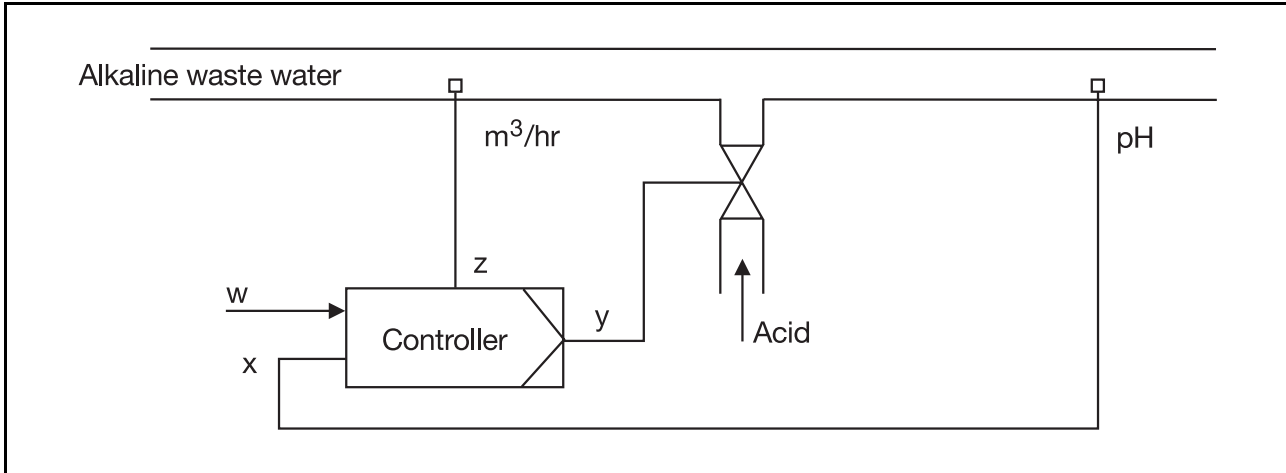
Fig. 68: Neutralization plant
