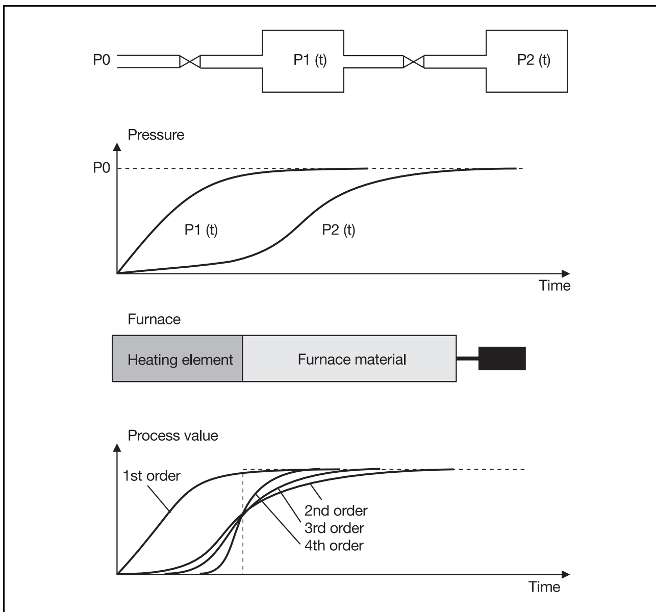
Fig. 23: Processes with delay
