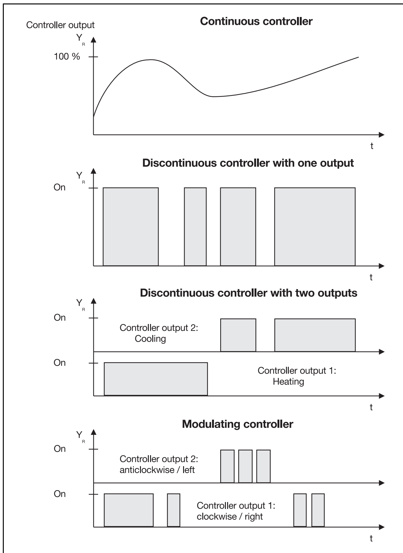
Fig. 4: Difference in controller functions
