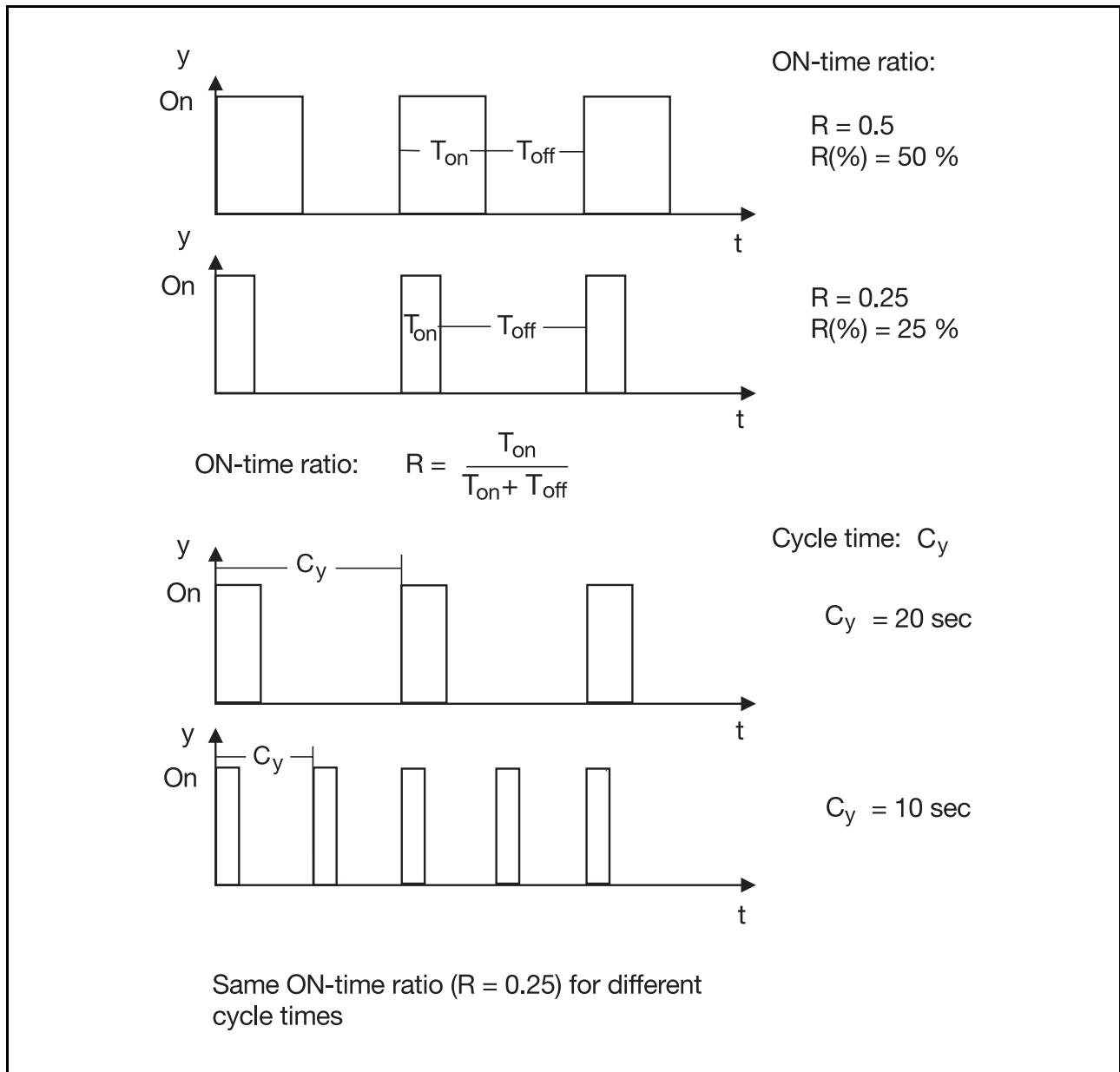
Fig. 57: Power control
