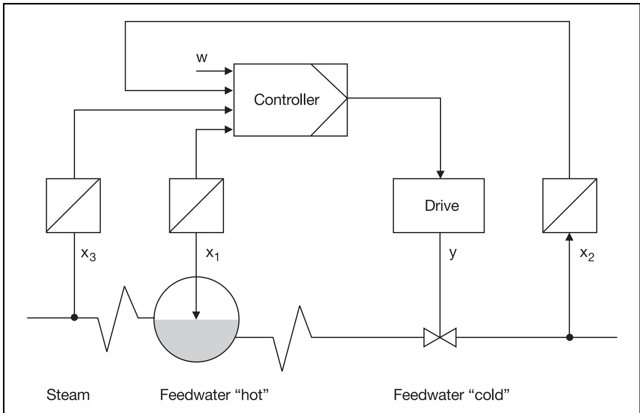
Fig. 74: Multi-component control
