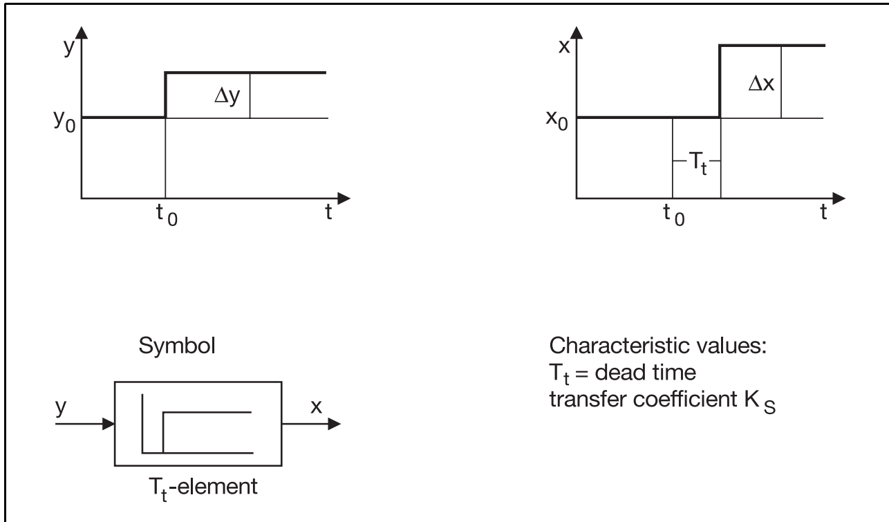
Fig. 21: Process with dead time; T_t process
