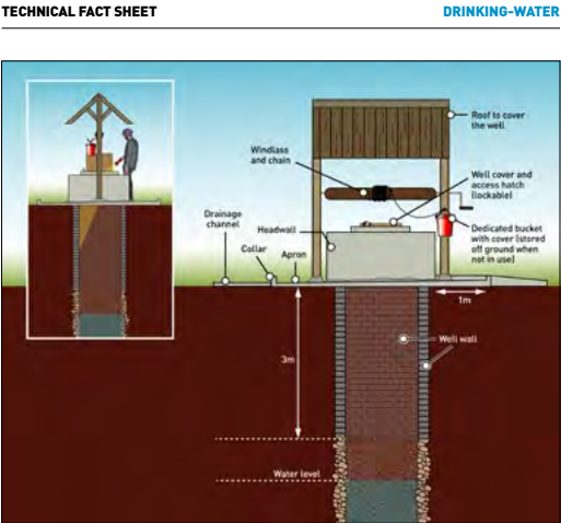
Figure 1. A common dug well with a windlass
