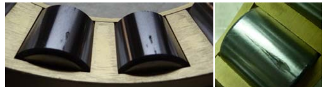
Rollers true brinelling – Cylindrical roller bearing
