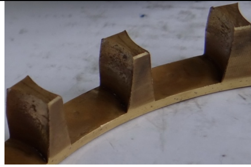
Worn cage pockets and seizure of outer surface
