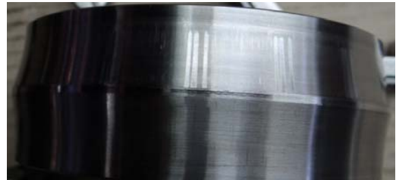
Raceway true brinelling – Spherical roller bearing
