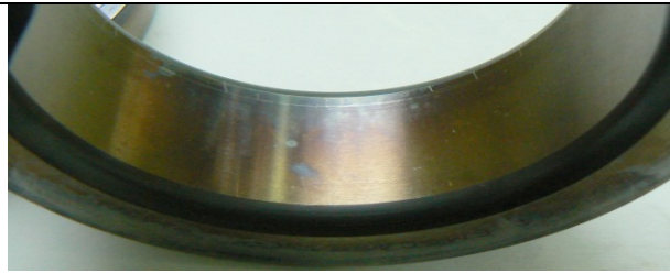
Inner ring bore – colour changed.
