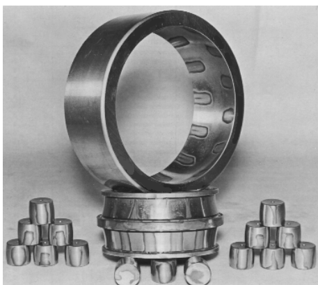
Staining in storage. Improper stored bearing in humid atmosphere, with inadequate protection.
