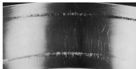
Corrosion in storage. The corrosion takes place underneath the rollers where moisture is trapped.
