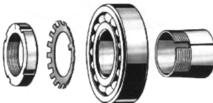
Adapter sleeve
