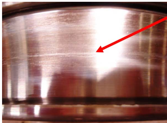
Smearing on inner ring raceway
