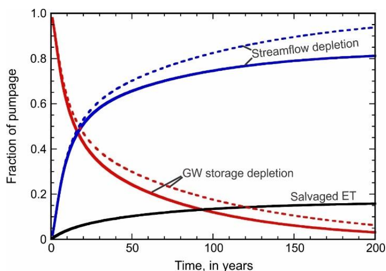
Figure 24 - Nondimensional sources of water being pumped based on annual rates for the base case model (dashed lines) and for the case with low ET (solid lines) (Konikow and Bredehoeft, 2020).
