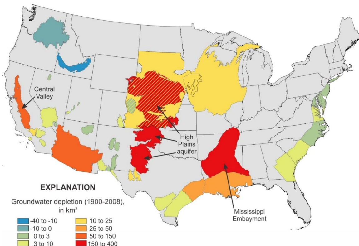
Figure 5 - Cumulative long-term volumetric groundwater storage depletion in the United States during 1900-2008, in \text{km}^3 (modified from Konikow, 2013). The three aquifers with the highest depletion volumes are identified. Hachured areas are where a shallow aquifer overlies a deeper aquifer.
