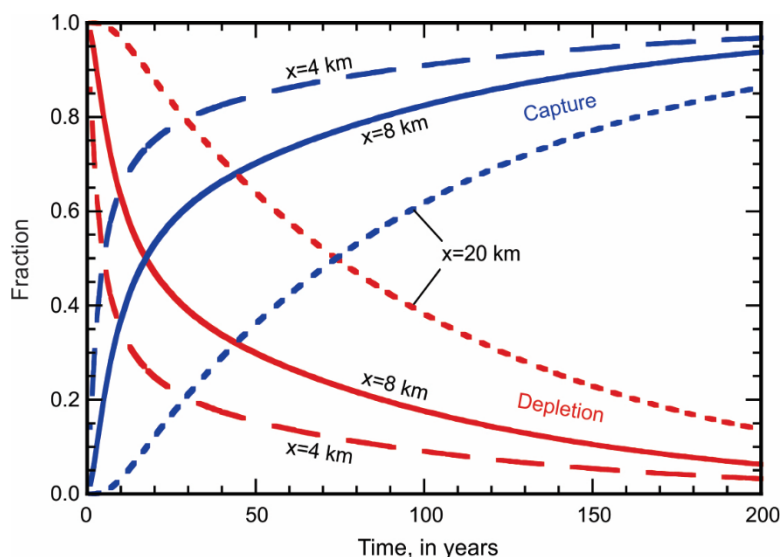
Figure ExSol 1-5 - Annual storage depletion and capture fractions for simulations of variants of the base case (Figure 17) in which the distance from the well to the stream is varied by placing it at a distance ( x ) of 4 km, 8 km (the base case), and 20 km from the river. Storage depletion fractions are shown in red and capture fractions are shown in blue (Konikow and Bredehoeft, 2020).
