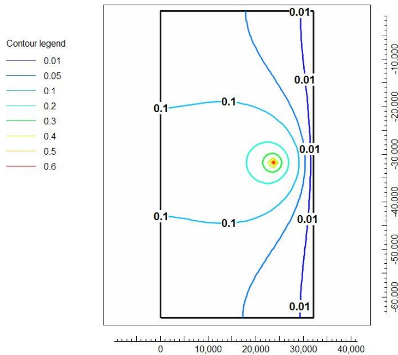
Figure ExSol 1-8. Contour map of drawdown (in m) in the aquifer after 200 years of pumping for the Base Case (Konikow and Bredehoeft, 2020).
