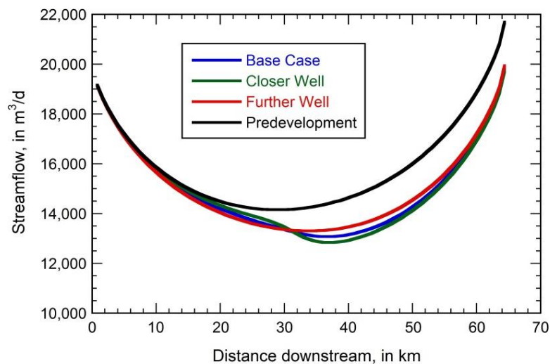
Figure ExSol 1-1 - Effect of well location on streamflow after 200 years. For comparison, streamflow is shown under steady-state predevelopment conditions (Konikow and Bredehoeft, 2020).
