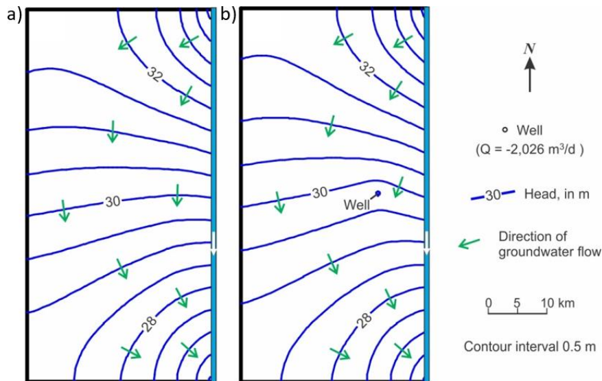
Figure 20 - Map showing calculated water-table elevations in the hypothetical stream-aquifer system for the base case in which there is no areal recharge and no ET: a) for predevelopment conditions, and b) after 200 years of pumping. The head values are relative to an arbitrary datum (Konikow and Bredehoeft, 2020).
