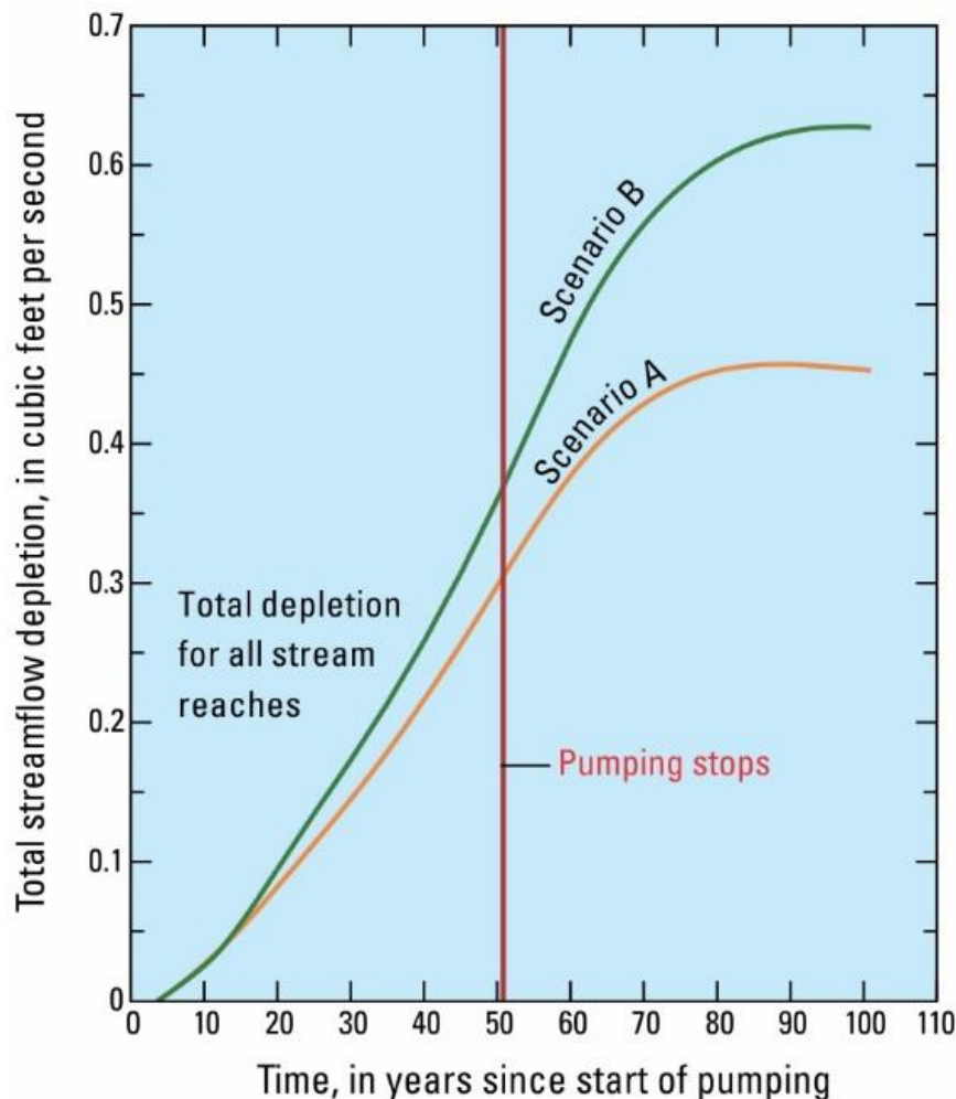
Figure 15 - Streamflow depletion as a function of time for two scenarios of groundwater pumping from the C aquifer, northeastern Arizona, USA (from Barlow and Leake, 2012, as modified from Leake et al., 2005).
