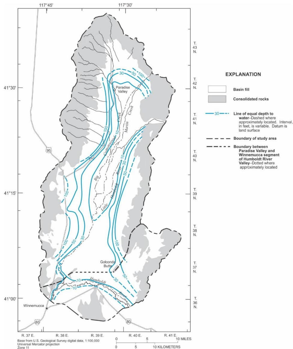
Figure 31 - Depth to groundwater in Paradise Valley, Nevada, prior to major development (pre-1969) (from Prudic and Herman, 1996).
