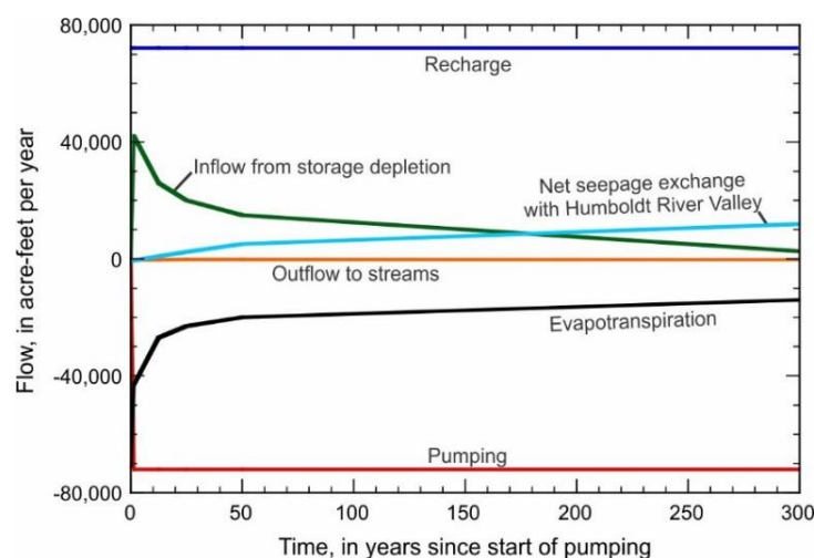
Figure 36. Model-calculated fluxes versus time for a scenario in which pumping of 72,000 ac-ft/yr ( 2.82 \text{ m}^3/\text{s} ) is distributed widely in Paradise Valley (data from Prudic and Herman, 1996, scenario 5). Recharge includes both mountain front recharge and infiltration from streams.
