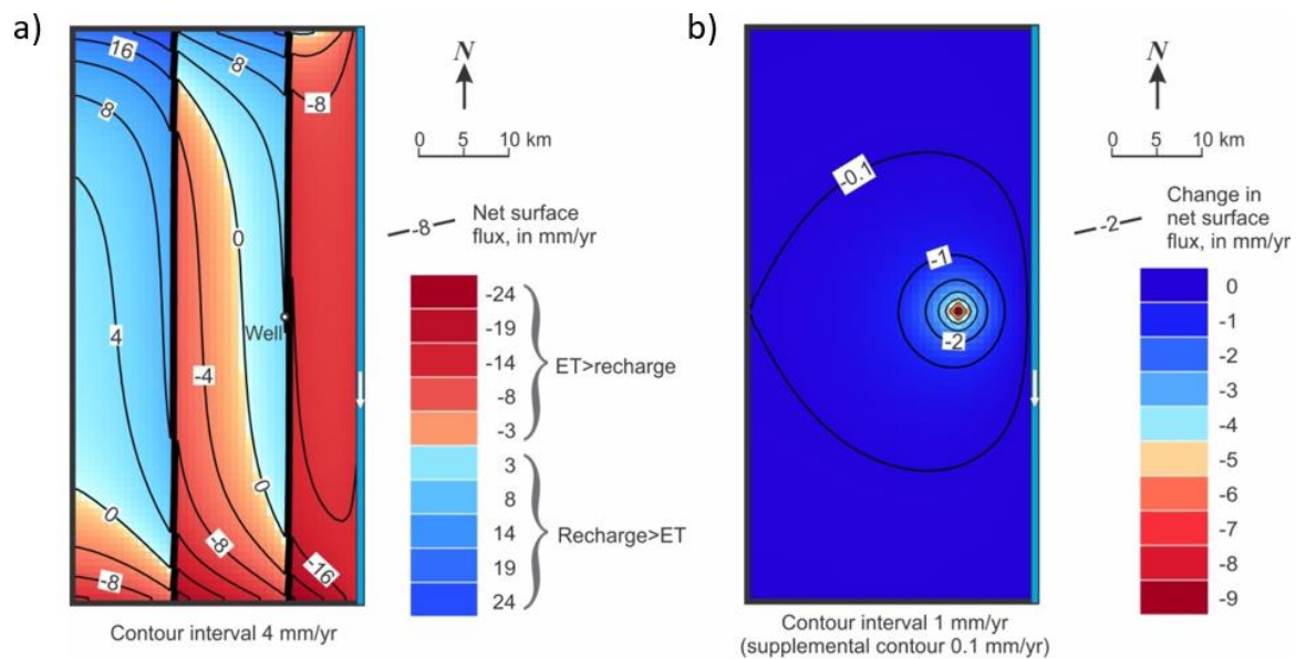
Figure 25 – Net surface flux is the difference between recharge and evapotranspiration: a) Net surface flux (recharge minus ET) for predevelopment conditions, and b) change in net surface flux after 200 years of pumping (Konikow and Bredehoeft, 2020).
