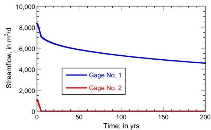
Figure ExSol 2-2 - Streamflow changes for 200 years at two gaging stations. Gage No. 1 is located at the outflow from the modeled area (reach 80) and Gage No. 2 is located at reach 46 (37km) downstream from where the river enters the modeled area) (Konikow and Bredehoeft, 2020).
