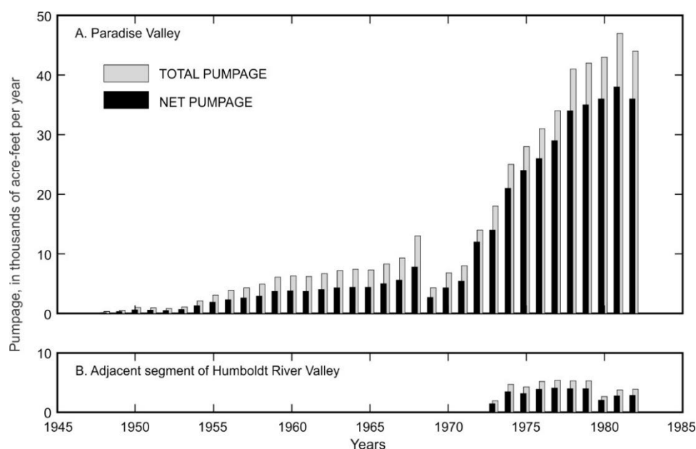
Figure 32 - Pumping in Paradise Valley and the associated part of the Humboldt River Valley (from Prudic and Herman, 1996). Net pumpage equals total pumpage minus the amount estimated to return to basin-fill aquifer through infiltration of irrigation water. [ 1,000 \text{ ac-ft} = 1.23 \text{ million m}^3 = 1.23 \times 10^{-3} \text{ km}^3 ].
