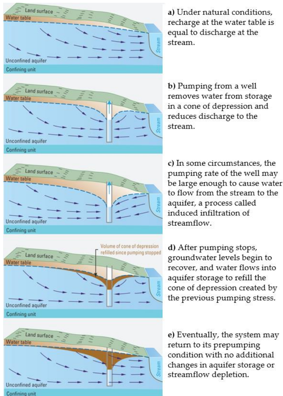
Figure 9. Effects of pumping groundwater from a hypothetical water-table aquifer that discharges to a stream. Sequence shows progressive changes to groundwater flow and streamflow before, during, and after pumping at a hypothetical well site (from Leake and Barlow, 2013; as modified from Heath, 1983; Alley et al., 1999).
