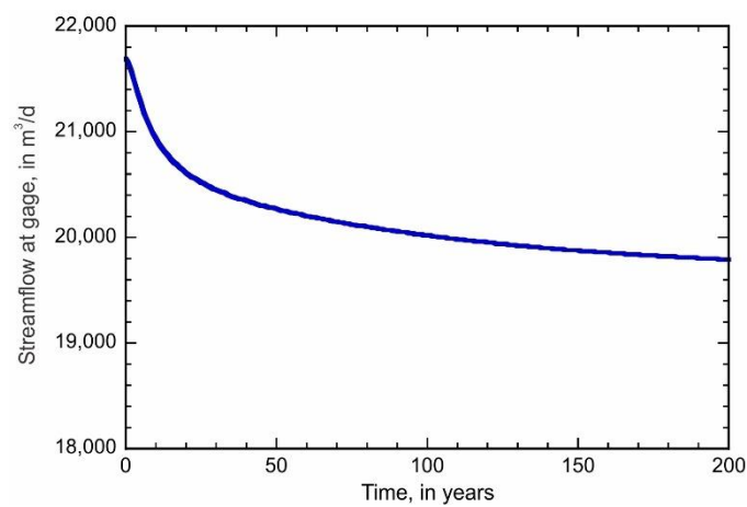
Figure Box 3-12 - Streamflow at model outlet for the Base Case of Case Study 1 (Konikow and Bredehoeft, 2020).
