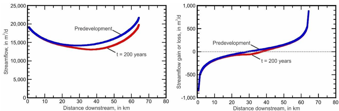
Figure Box 3-10 - Streamflow and stream Gain(+) and Loss(-) with distance downstream for the Base Case of Case Study 1 (Konikow and Bredehoeft, 2020).
