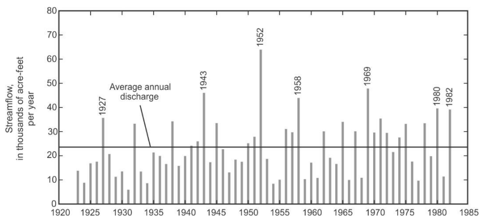
Figure 29 - Annual discharge of Martin Creek where it enters Paradise Valley, Nevada, USA. [1,000 ac-ft = 0.000123 km 3 ] (from Prudic and Herman, 1996).
