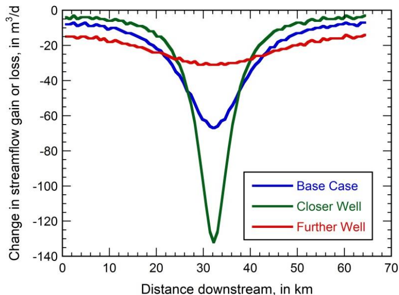
Figure ExSol 1-4 - Changes in streamflow gains and losses attributable to pumping for 200 years at three different well locations (Konikow and Bredehoeft, 2020).
