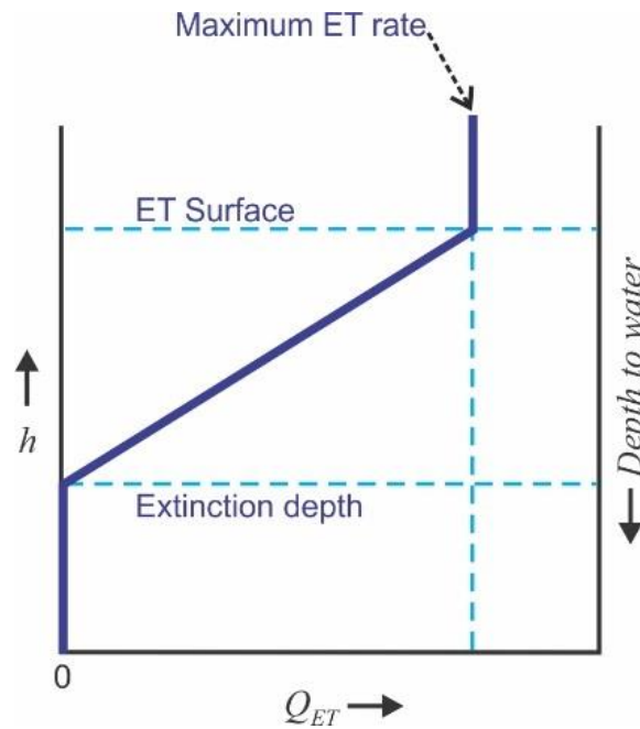
Figure 19 - The linear function relating ET rate ( Q_{ET} ) to depth of the water table in the MODFLOW-NWT model ( h is the head [water level]) (Konikow and Bredehoeft, 2020).
