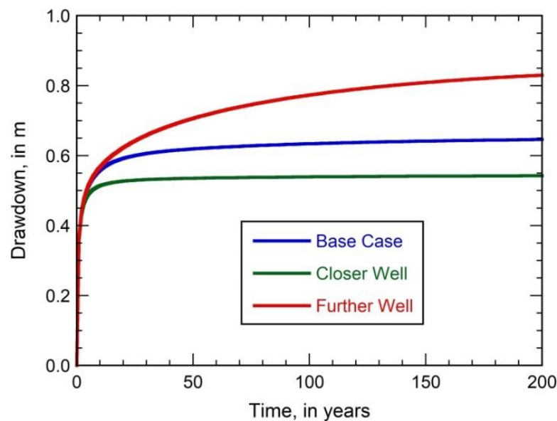
Figure ExSol 1-7 - Calculated drawdown in the pumping well for three different well locations (Konikow and Bredehoeft, 2020).
