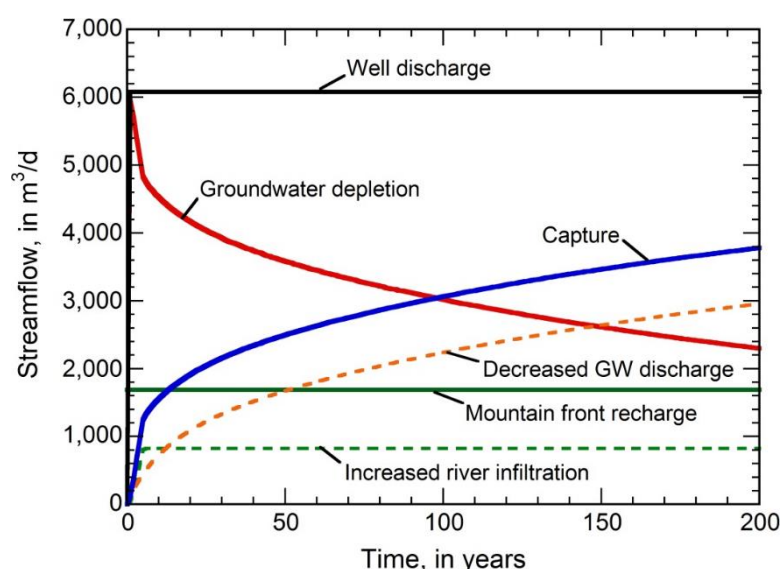
Figure ExSol 2-6 - Calculated changes in the water budget of the hypothetical desert-basin aquifer during the 200-year simulation period for the Exercise 2 case. Capture is the sum of its components represented by the dashed lines (Konikow and Bredehoeft, 2020).
