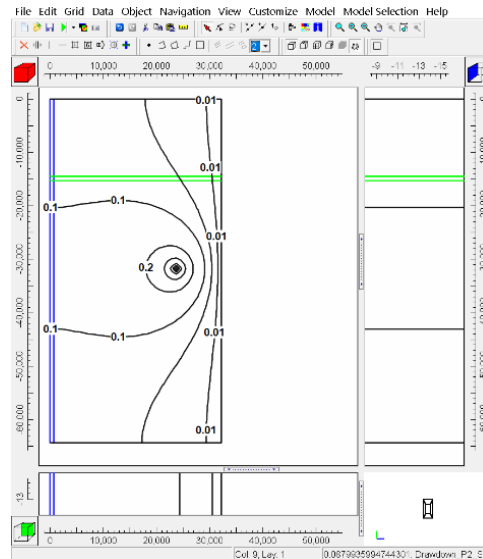
Figure Box 3-5 - Drawdown contours with the grid and object removed from view (Konikow and Bredehoeft, 2020).
