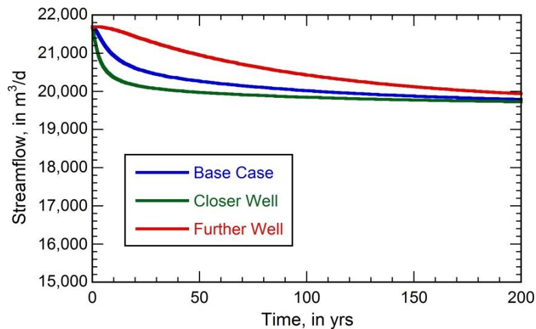
Figure ExSol 1-2 - Effect of pumping on streamflow as recorded at the stream gage at the outlet of the model during 200 years of pumping for three different well locations (Konikow and Bredehoeft, 2020).
