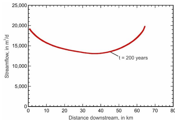
Figure Box 3-8 - Streamflow with distance downstream for the Base Case of Case Study 1 (Konikow and Bredehoeft, 2020).
