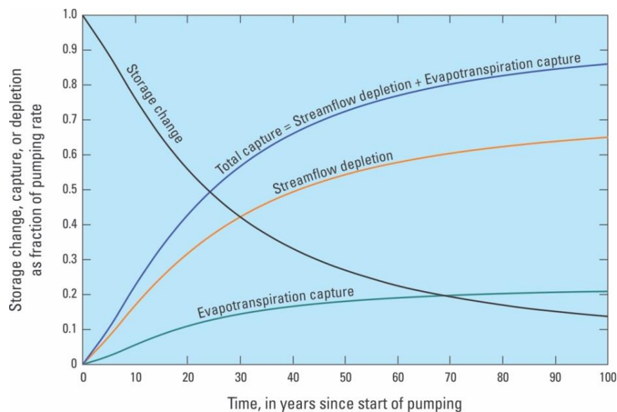
Figure 16 – Model-computed streamflow depletion, evapotranspiration capture, storage change, and total capture for the location of one hypothetical well that pumps for 100 years in the Upper San Pedro Basin, Arizona (from Barlow and Leake, 2012; after Leake et al., 2008).
