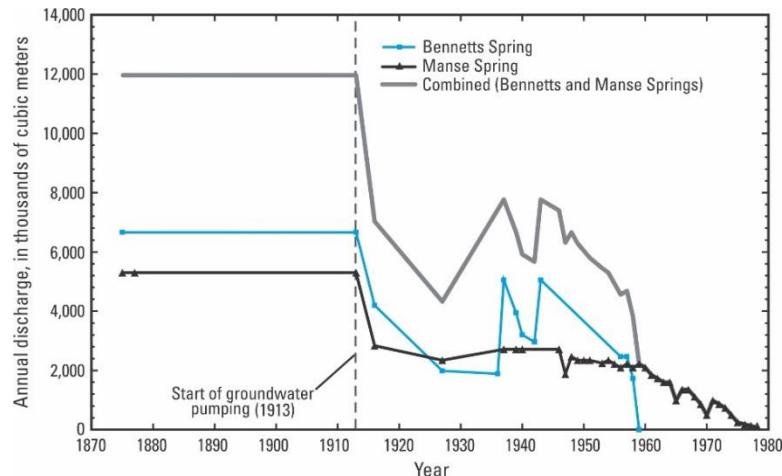
Figure 14 - Annual discharge from regional springs in Pahrump Valley, Nevada, 1875-1978, showing trend of decreasing spring flow after onset of pumping (modified from San Juan et al., 2010).
