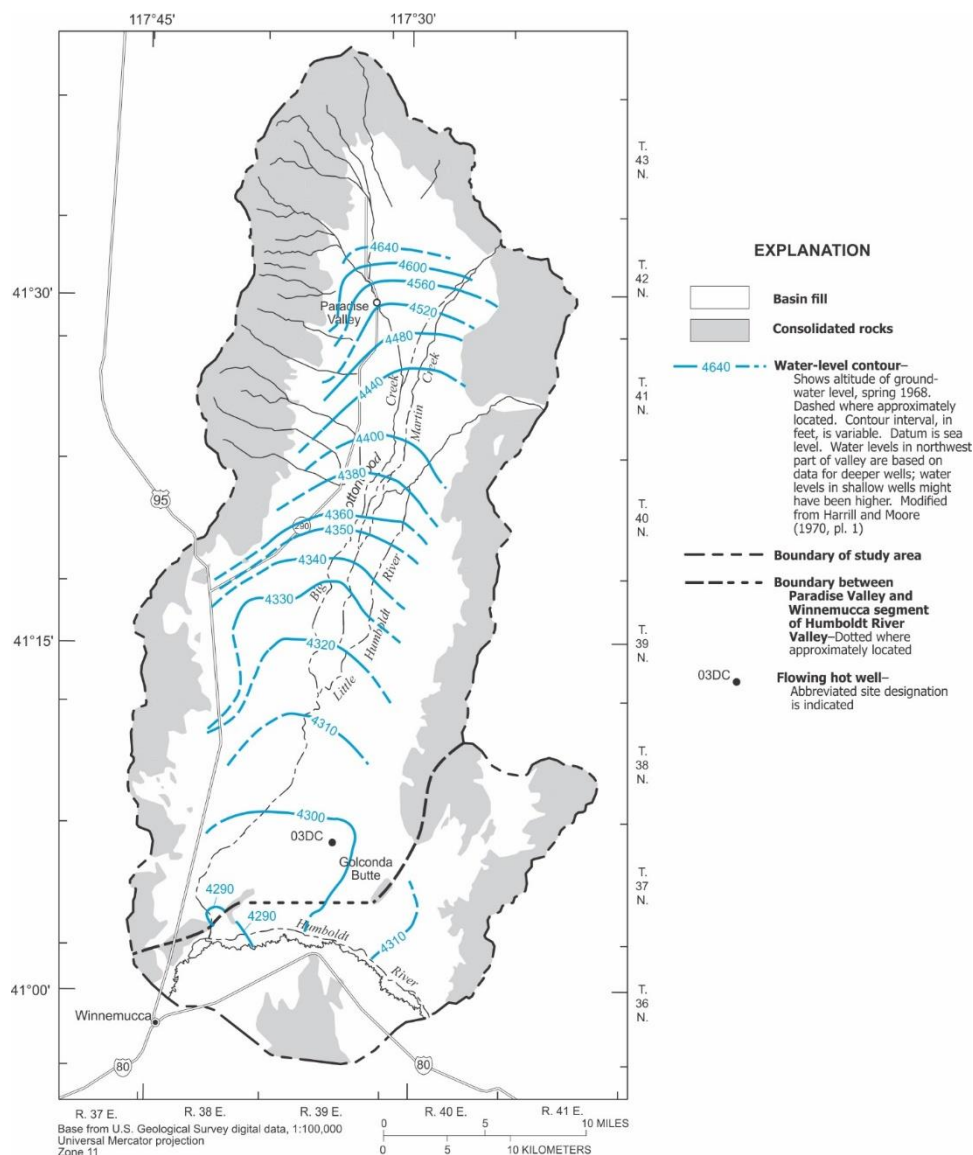
Figure 30 - Groundwater levels in Paradise Valley, Nevada, spring 1968 (from Prudic and Herman, 1996).
