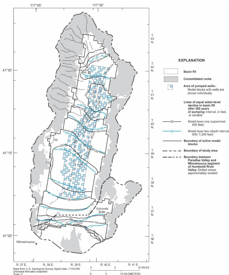
Figure 37 - Drawdown after 300 years resulting from scenario with pumping 72,000 ac-ft/yr ( 2.82 \text{ m}^3/\text{s} ) from the locations distributed widely in the area of evapotranspiration near the center of valley (from Prudic and Herman, 1996). Individual pumping wells are located in model cells shaded blue.
