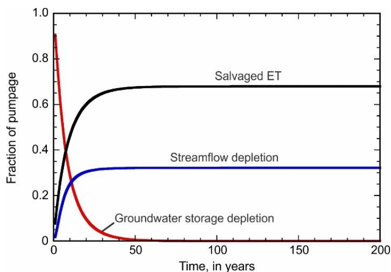
Figure 27 - Simulated nondimensional sources of water being pumped based on annual rates for the case with ET and recharge (Konikow and Bredehoeft, 2020).
