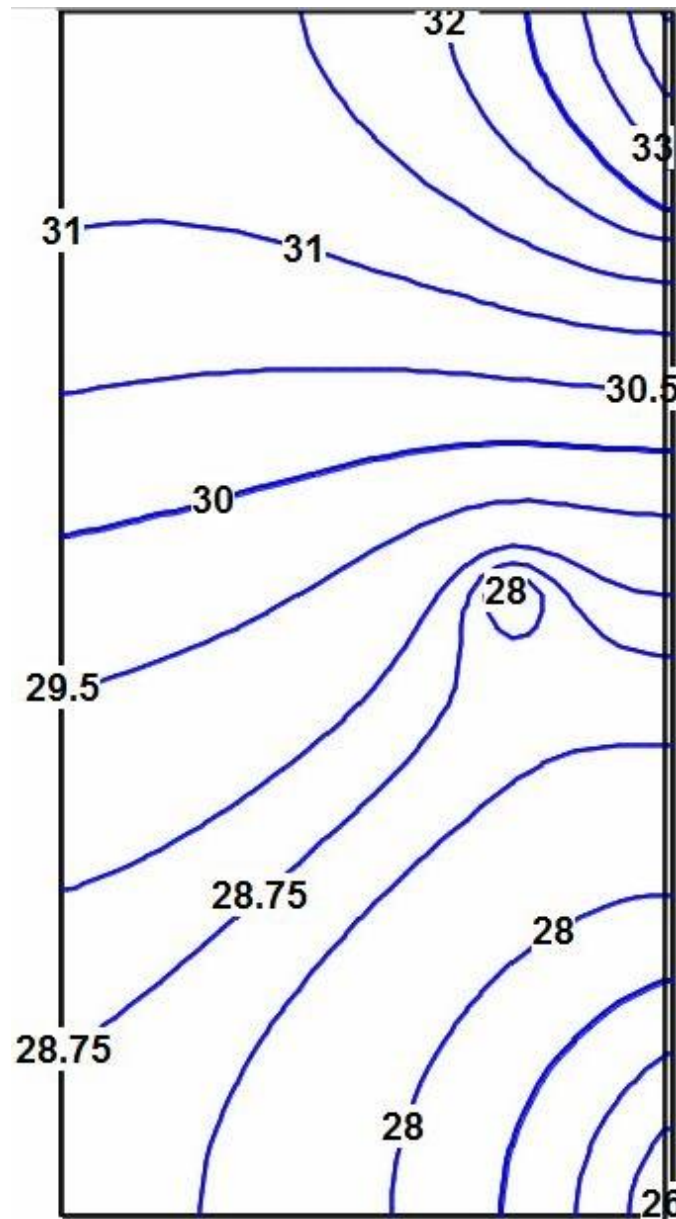
Figure ExSol 2-5 - Calculated heads (in m) in the aquifer after 200 years for conditions of Exercise 2 (with higher pumping rate). The contour interval is 0.5 m, with a supplementary contour at 28.75 m (Konikow and Bredehoeft, 2020).
