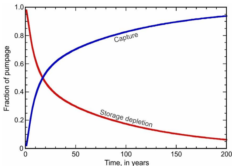
Figure Box 3-7 - Fractional sources of water entering the pumping well for the Base Case of Case Study 1 (Konikow and Bredehoeft, 2020).
