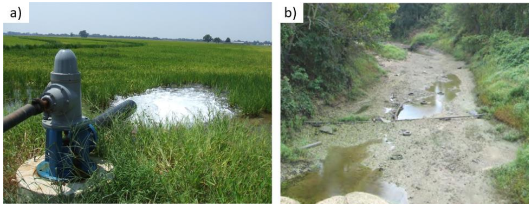
Figure 8 - There is a relation between groundwater pumping and streamflow depletion. a) Groundwater pumped from the Mississippi River alluvial aquifer for flood irrigation of a rice field in the Mississippi Delta, USA (Photograph by David E. Burt, Jr., United States Geological Survey; source : Barlow and Leake, 2012). b) A Delta stream (Big Sunflower River) that is nearly dry during the summer because of loss of base flow (Photograph by Matt Hicks, United States Geological Survey; source : Barlow and Clark, 2011).
