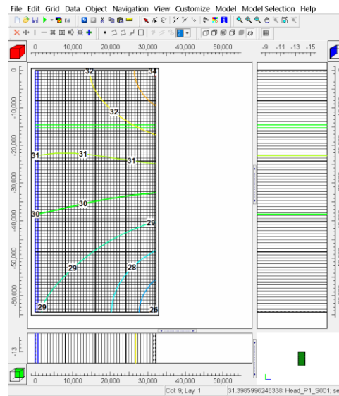
Figure Box 3-2 - Head contours for undeveloped conditions (Konikow and Bredehoeft, 2020).
