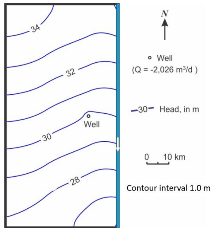
Figure 26 - Calculated water-table elevations after 200 years of pumping for the case in which there is both diffuse areal recharge and ET. Head is relative to an arbitrary datum. (Konikow and Bredehoeft, 2020).
