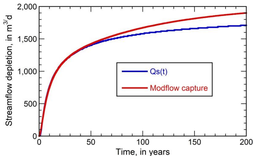
Figure ExSol 3-1 - Streamflow depletion estimates for analytical and numerical solutions for the Base Case scenario. The Q_s(t) (blue curve) is the streamflow depletion calculated using the analytical solution developed by Glover and Balmer (1954). The red curve represents capture calculated from the water budget data of the numerical solution using MODFLOW-NWT for the Base Case (Konikow and Bredehoeft, 2020).
