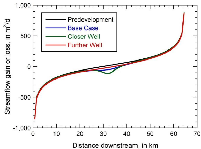
Figure ExSol 1-3 - Changes in streamflow along the length of the river for predevelopment conditions and after 200 years of pumping at three different well locations (Konikow and Bredehoeft, 2020).
