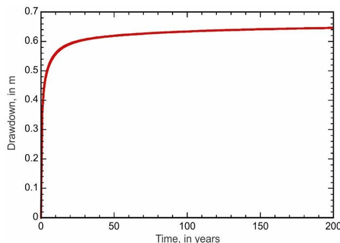
Figure Box 3-11 - Drawdown at the pumping well location for the Base Case of Case Study 1 (Konikow and Bredehoeft, 2020).
