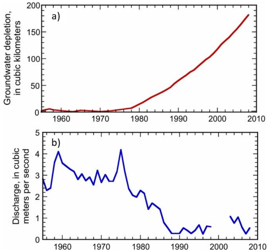
Figure 10 - Relation between groundwater depletion and stream discharge. a) Cumulative groundwater depletion in the Mississippi Embayment regional aquifer system, USA, 1955 through 2008 (Konikow, 2013). b) Annual minimum mean daily streamflow for the Big Sunflower River, Mississippi, USA, showing effects of withdrawals from the aquifer on base flow of the stream and indicating streamflow depletion after the late 1970s; data are missing for 1998-2002 (modified from Welch et al., 2010).
