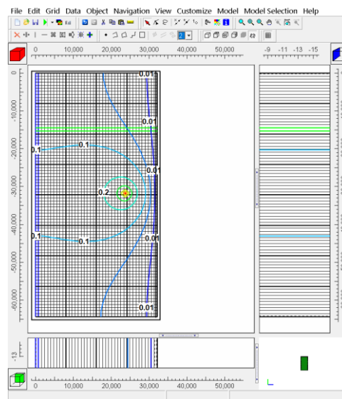
Figure Box 3-4 - Drawdown contours after 200 years of pumping including two contour lines for smaller drawdown (Konikow and Bredehoeft, 2020).
