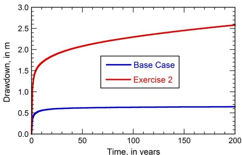
Figure ExSol 2-4 - Calculated drawdown in the pumping well for Base Case and Exercise 2 (with higher pumping rate) (Konikow and Bredehoeft, 2020).
