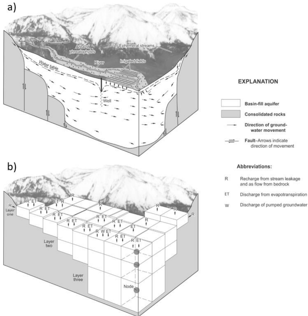
Figure 35 - Schematic three-dimensional diagram that illustrates how the groundwater system in Paradise Valley was subdivided into a finite system of rectangular cells for the purpose of numerical analysis (modified from Prudic and Herman, 1996).
