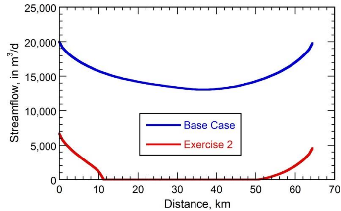
Figure ExSol 2-1 - Streamflow variations with distance after 200 years (Konikow and Bredehoeft, 2020).
