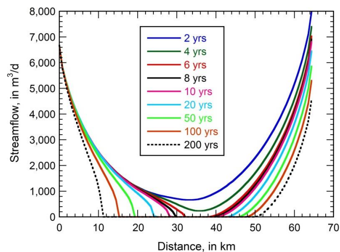
Figure ExSol 2-3 - Changes in the streamflow profile during the 200-year simulation period showing growth in the length of the dry central reaches after year 5 (Konikow and Bredehoeft, 2020).
