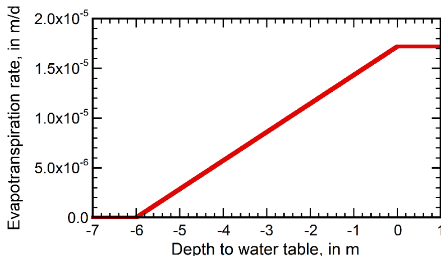
Figure 23 - Relation between evapotranspiration rate and depth to the water table as represented in the MODFLOW model for the Low-ET Case (Konikow and Bredehoeft, 2020).
