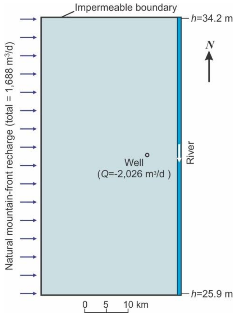
Figure 17 - Hypothetical and idealized desert basin aquifer with a perennial river along its eastern side and mountain front recharge along its western side (modified from Barlow and Leake, 2012).
