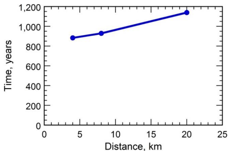
Figure ExSol 1-6 - Relation between time for model to reach a new steady-state condition and the distance from the pumping well to the river (Konikow and Bredehoeft, 2020).
