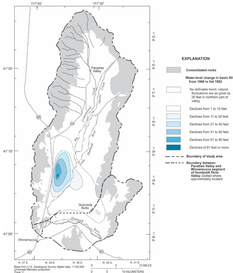
Figure 34 - Water-table decline, 1968 to 1982 (from Prudic and Herman, 1996).
