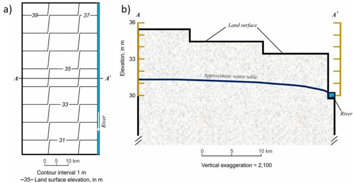
Figure 18 - Topography of the hypothetical stream-aquifer system; a) map view, b) cross-sectional view along line A-A', showing approximate predevelopment water table. Water depth in the river is not shown to scale (Konikow and Bredehoeft, 2020).
