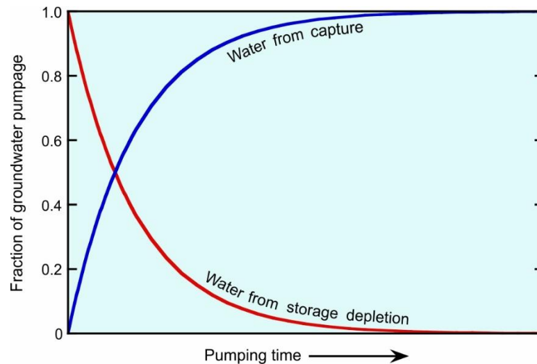
Figure 4 - Sources of water to a well can change with time ( from Konikow and Leake, 2014, as modified from Alley et al., 1999, and Barlow and Leake, 2012 ).
