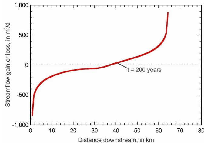
Figure Box 3-9 - Streamflow Gain(+) and Loss(-) with distance downstream for the Base Case of Case Study 1 (Konikow and Bredehoeft, 2020).
