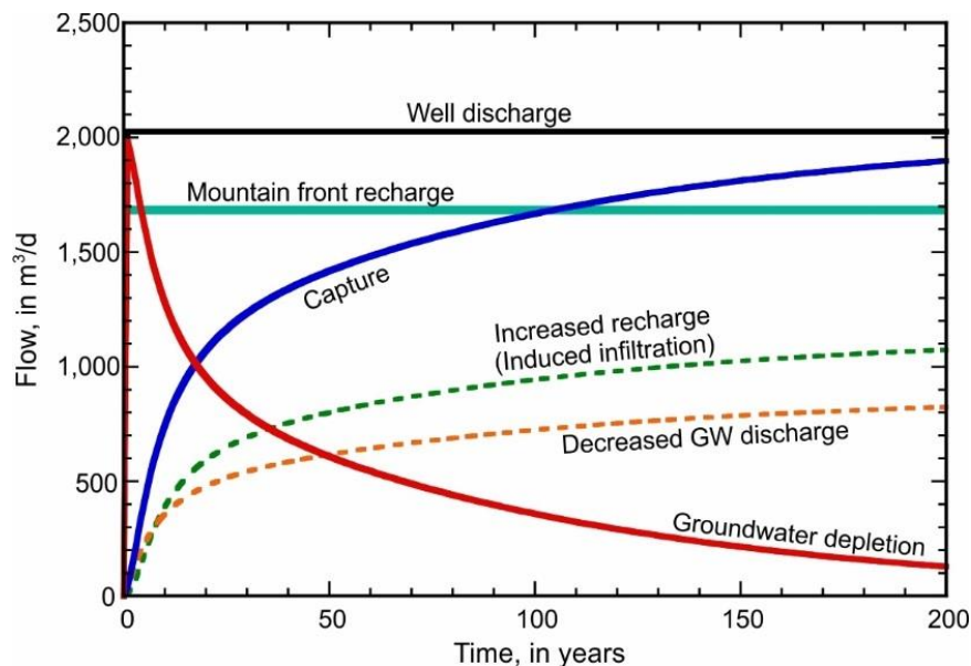
Figure 21 - Calculated changes in the water budget of the hypothetical desert basin aquifer during the 200-year simulation period for the base case model. Capture is the sum of its components represented by the dashed lines (Konikow and Bredehoeft, 2020).
