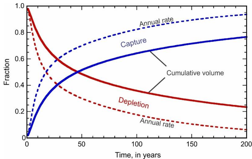
Figure 22 - Nondimensional sources of water being pumped based on both annual rates (dashed lines) and cumulative volumes (solid lines) for the base case model (Konikow and Bredehoeft, 2020).
