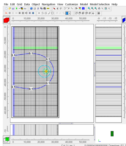
Figure Box 3-3 - Drawdown contours after 200 years of pumping (Konikow and Bredehoeft, 2020).
