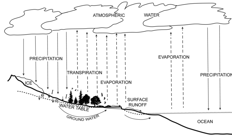
Hydrologic cycle
