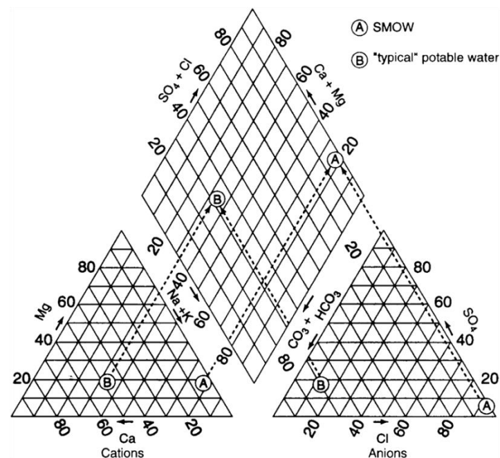
Piper diagram. The acronym SMOW is Standard Mean Ocean Water.
