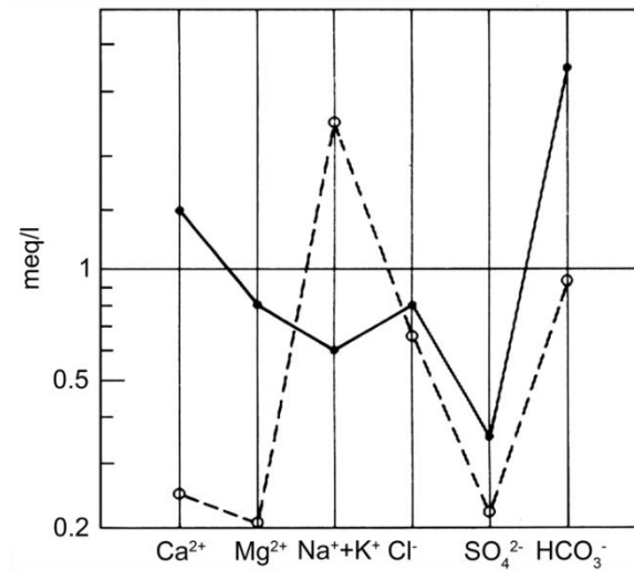
Schoeller Diagram (Freeze and Cherry, 1979, p. 251)
