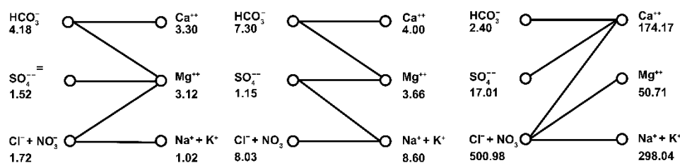
Examples of Taussig diagrams (Mandel & Shiftan, 1981). Left: Ca – Mg – \text{HCO}_3 facies (TDS \approx 520 mg/L); Center: Na – Cl – \text{HCO}_3 facies (TDS \approx 1120 mg/L); Right: Na – Ca – Cl facies (TDS \approx 29,800 mg/L).
