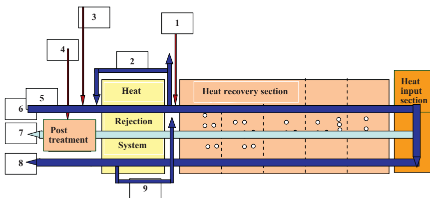
Fig. 31. MSF process scheme with input and output concentrations of additives and brine characteristics [6].
