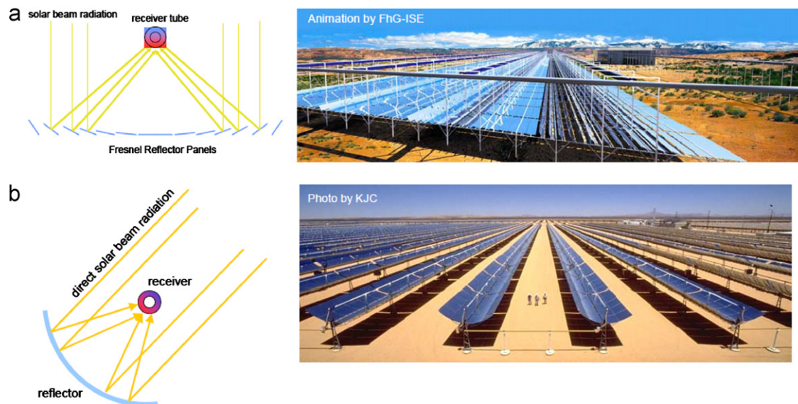
Fig. 16. Principle of line focusing concentrating solar collector systems [6]. (a) Animation of a linear Fresnel type concentrating solar thermal collector field for direct steam generation. (b) Parabolic trough solar field of the 5 × 30 MW solar electricity generating system (SEGS) in Kramer Junction, California.
