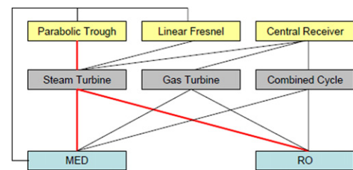
Fig. A6. Parabolic Trough with Steam Cycle.
