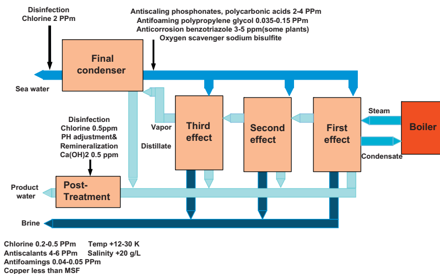
Fig. 35. MED process scheme with input and output concentrations of additives and brine characteristics.
