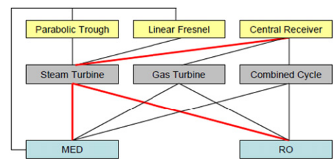
Fig. A3. Central Receiver with Steam Turbine.
