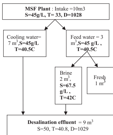
Fig. 32. Flow chart of reference MSF process with salinity (S, in g/L), temperature (T, in °C) and density (D, in g/L).
