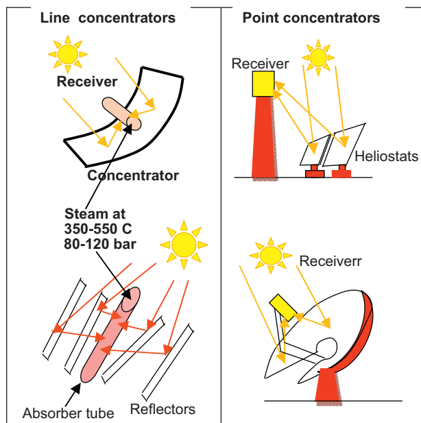
Fig. 15. The four mainstream CSP-technologies for the production of high-temperature solar heat for power generation and process steam: parabolic trough (upper left), linear Fresnel (bottom left), solar tower (upper right) and dish Stirling (bottom right) [11].
