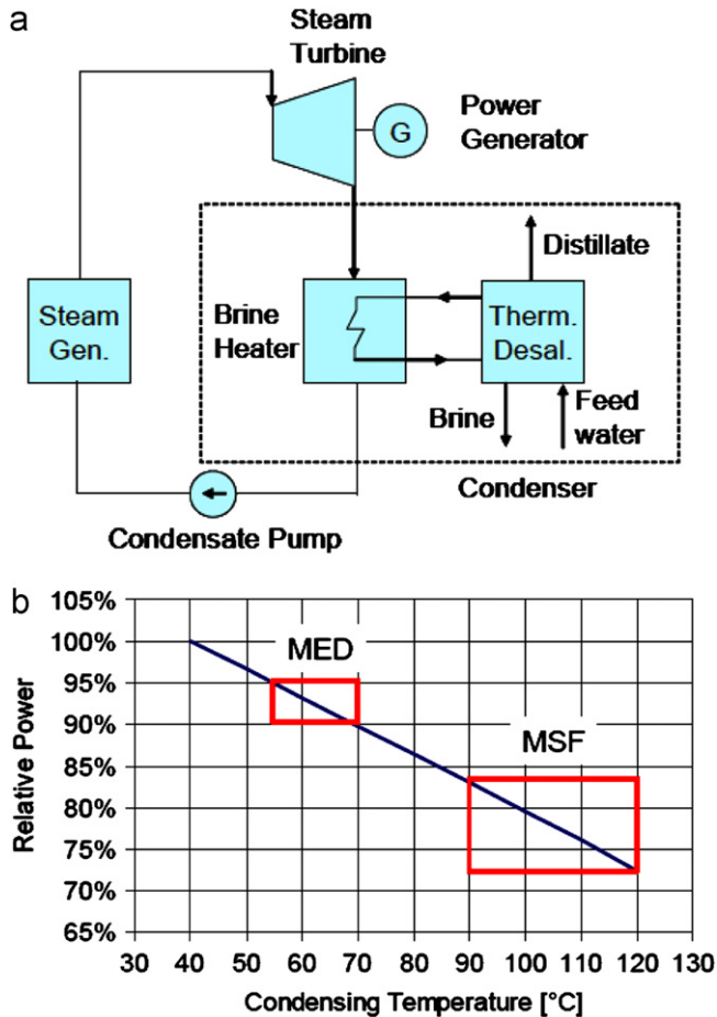
Fig. 6. (a) Principle of substituting the condenser of a steam cycle power plant by a thermal desalination unit [5,6]. (b) Typical reduction of steam turbine power capacity at increasing condensing temperature. The rectangle show the typical operating range of MED and MSF plants [5,6].
