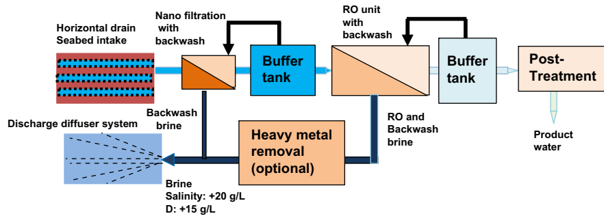
Fig. 41. Scheme of RO process including horizontal drain seabed intake, nano-filtration unit, buffer tank for backwash of nano-filtration membranes and discharge diffuser system.
