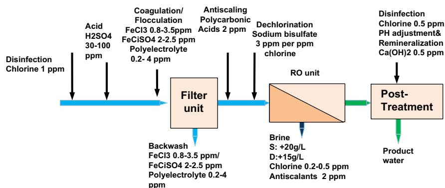
Fig. 37. RO process scheme with input and output concentrations of additives and brine characteristics, modified.
