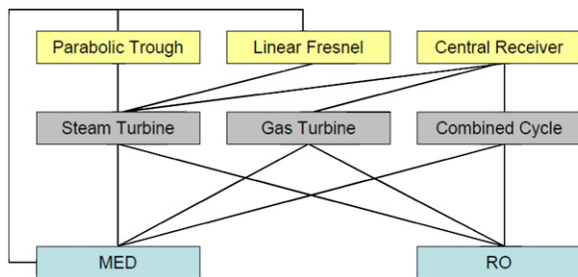
Fig. 23. Options of combining concentrating solar power (CSP) with desalination technologies [5,6].
