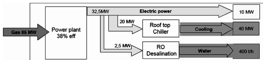
Fig. 21. Conventional solution for power, cooling and water for a hotel resort in Aqaba [6].
