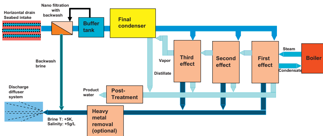
Fig. 40. Scheme of A-MED process including horizontal drain seabed intake, nano-filtration unit, buffer tank for backwash of nano-filtration membranes and discharge diffuser system.
