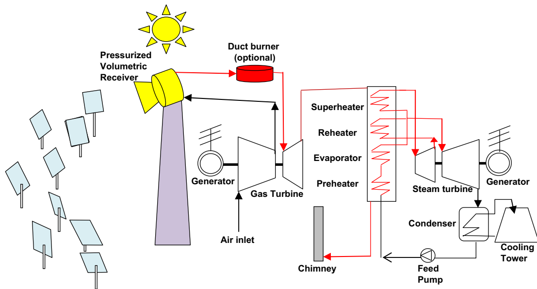
Fig. 19. Solar tower used for gas turbine operation in a combined cycle power plant [6].
