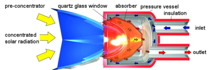
Fig. 20. Pressurized air heated by solar energy using a volumetric receiver [6].
