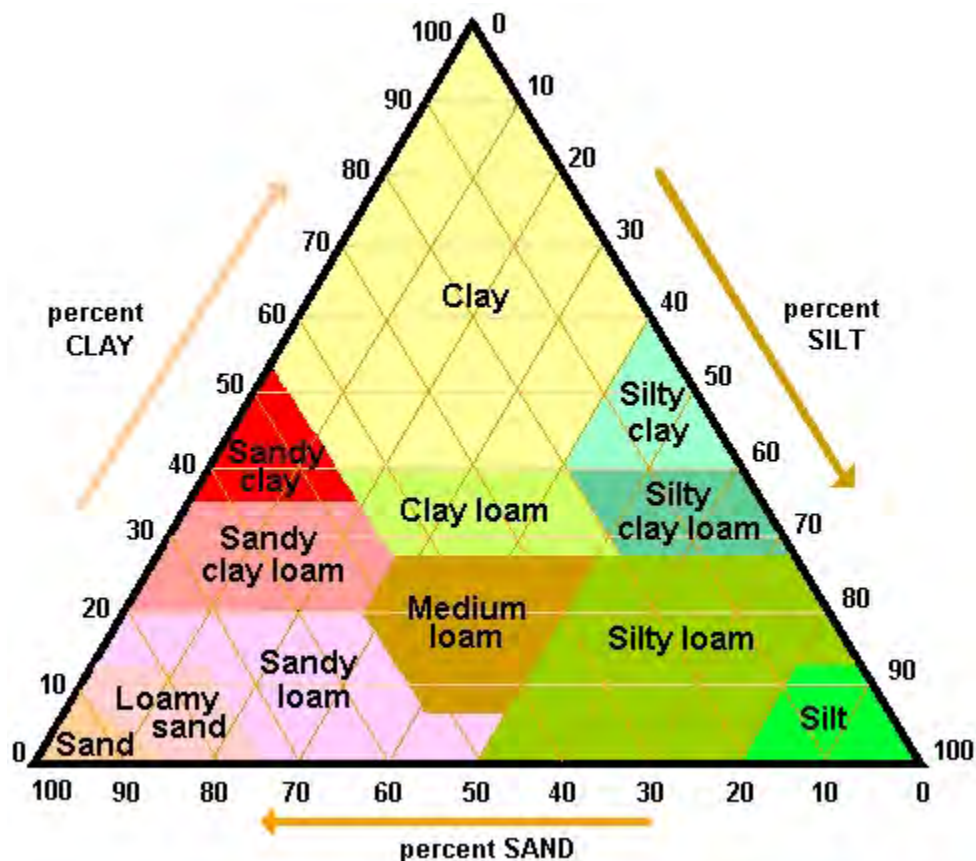
Figure 6-1: Soil Triangle
