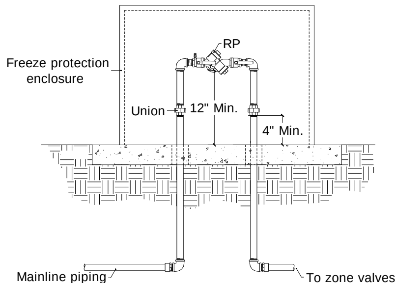
Figure 4-8: RP assembly
