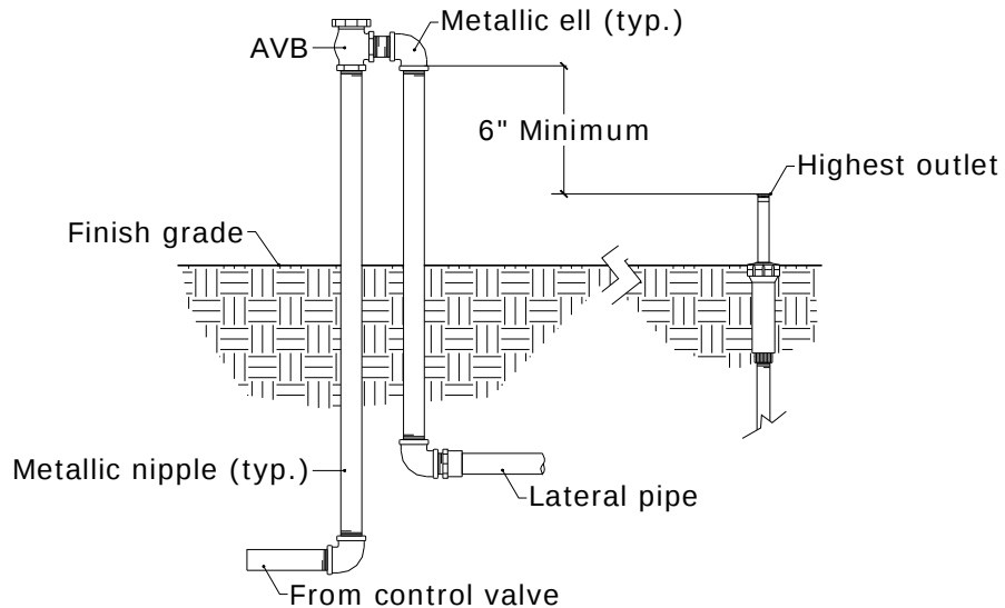
Figure 8-1: AVB assembly
