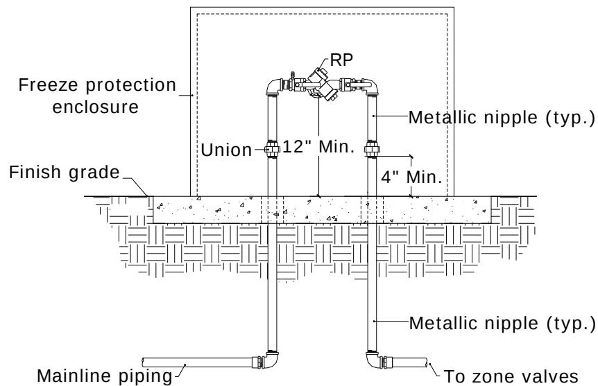
Figure 8-3: RP assembly
