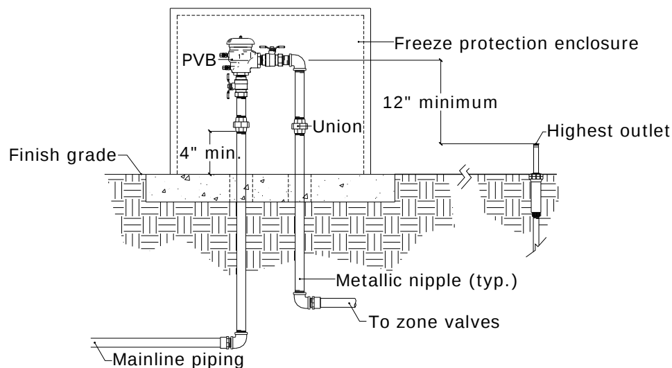
Figure 8-2: PVB assembly
