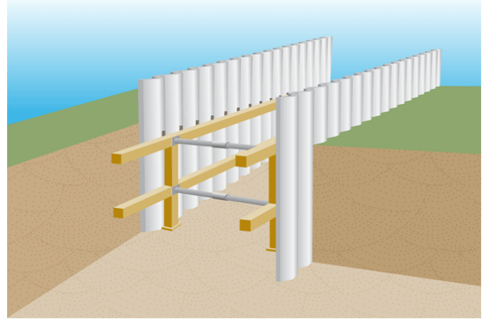
'Shoring the sides of an excavation by 'close sheeting'
