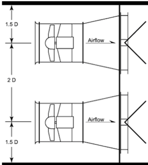
Vaneaxial Fans in Parallel
