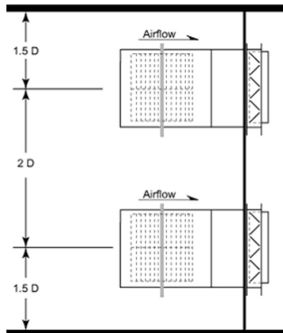
Double Width Centrifugal Fans in Parallel
