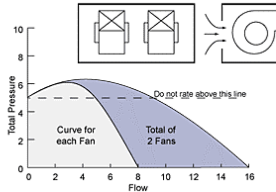
Two Fans in Parallel
