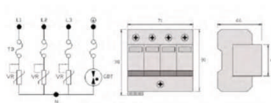
Electrical diagram and dimensions of BD2-100
