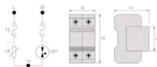
Electrical diagram and dimensions of BD2-60
