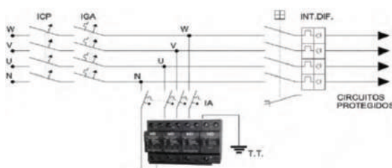
Circuit Diagram
