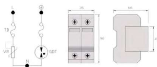
Electrical diagram and dimensions of BD2-40
