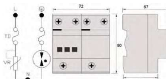
Electrical diagram and dimensions of BD2-100
