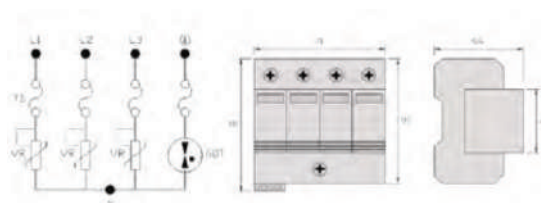
Electrical diagram and dimensions of BD4-60
