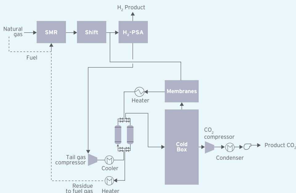
Figure 4-9: Process Flow Diagram of the Cryogenic Separation by Air Liquide (Cryocap™ H 2 Technology)
