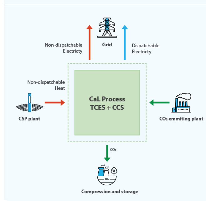
Figure 4-16: Schematic of Calcium Looping Capture for both CCS & TCES
