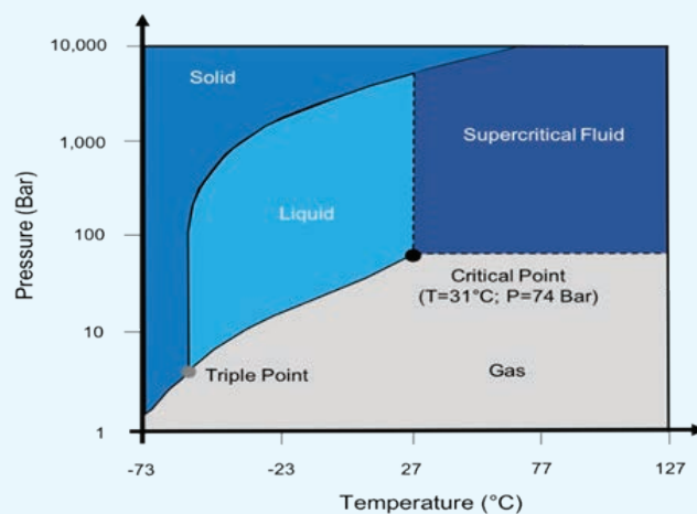
Figure 4-17: Phase Diagram of CO 2 Showing the Various Phase Stability Regions
