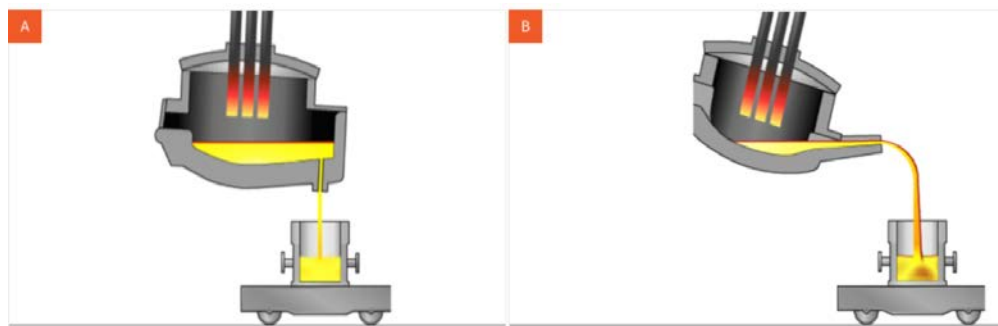
Figure 2.25. Different types of electric arc furnaces (EAF) [32].
