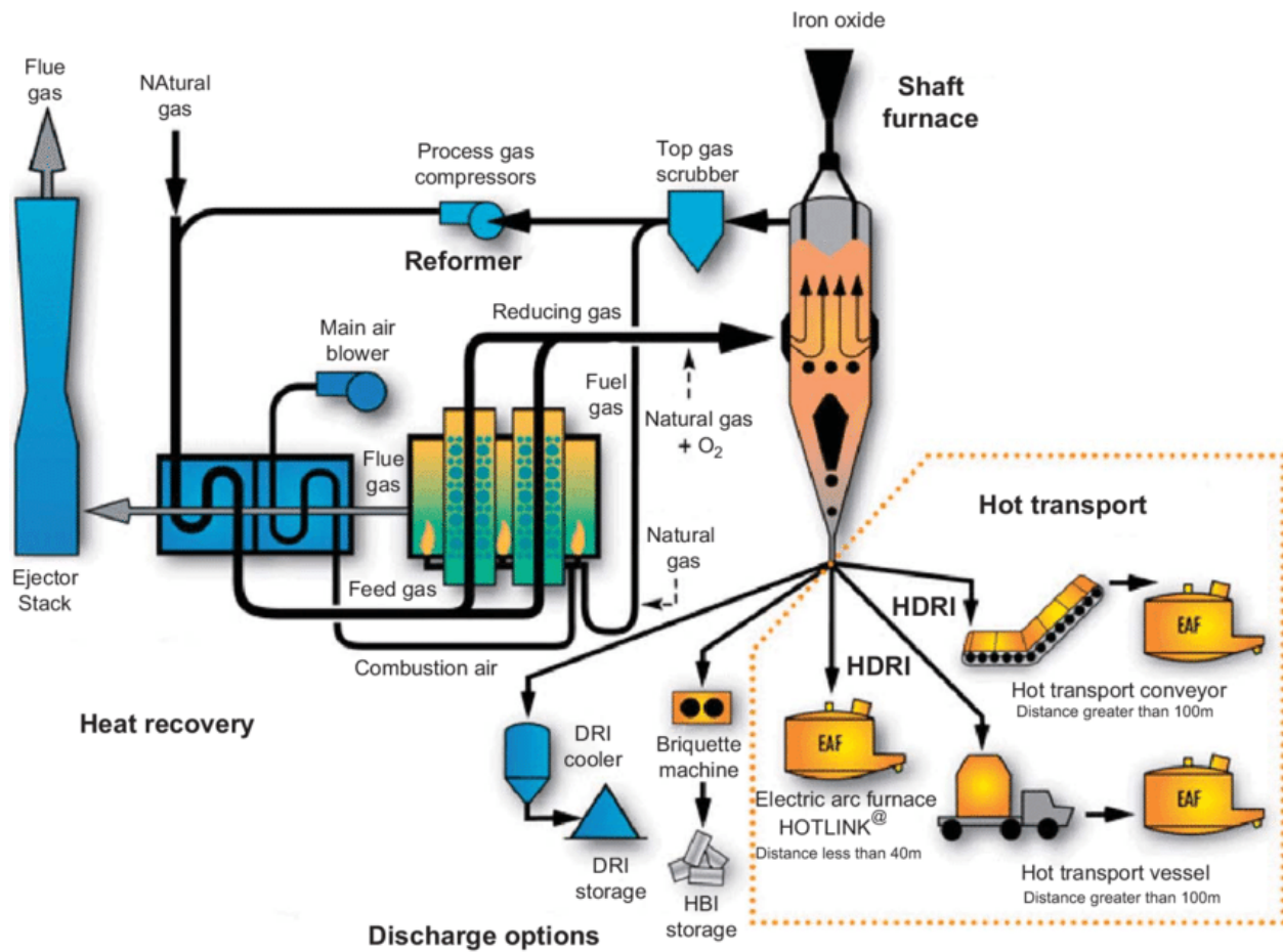
Figure 2.21. Process flowsheet for the Midrex DRI process [27]
