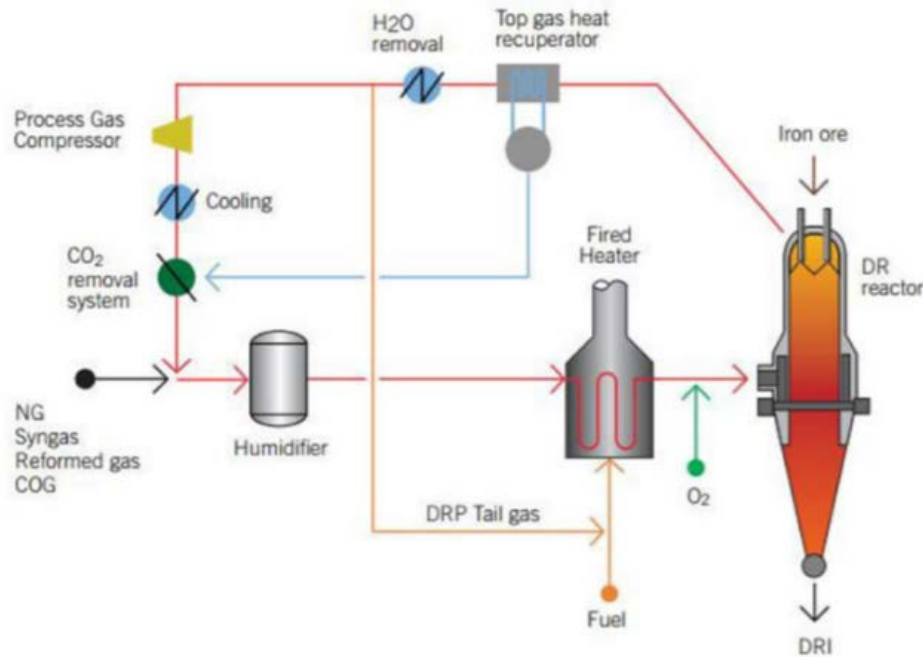
Standard Energiron process flowsheet
