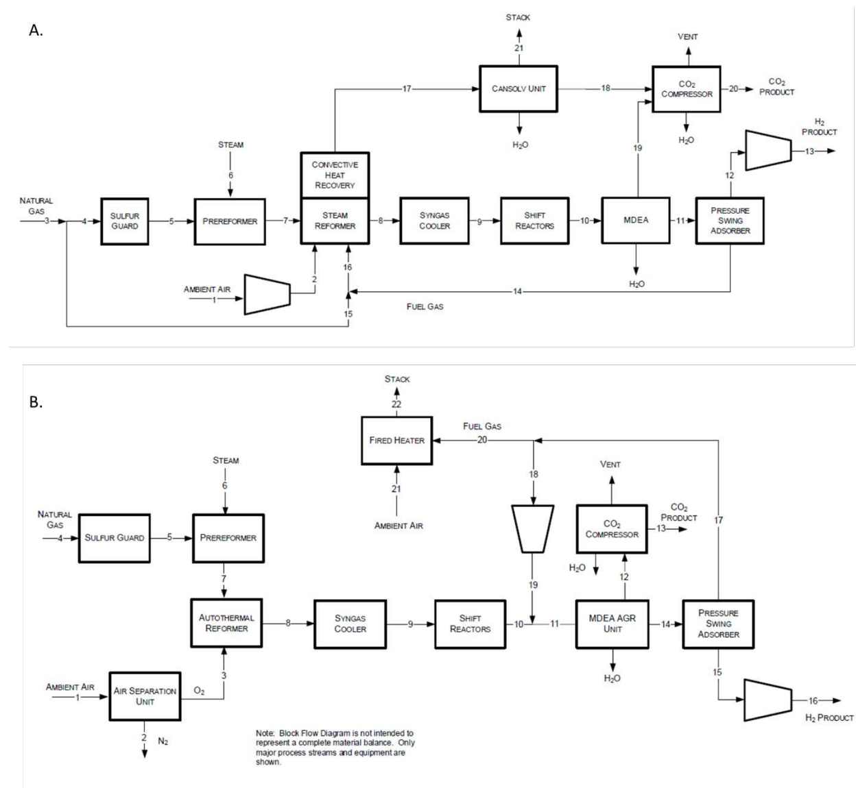
Figure 4.4. Block Flow Diagrams of state-of-the-art (A) SMR + CCS and (B) ATR + CCS technologies for hydrogen production.
