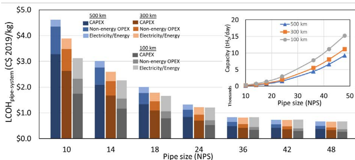
Figure 4.19. LCOH pipe-system is divided into: CAPEX pipe-system , Non-Energy OPEX pipe-system and Electricity /Energy pipe-system versus pipe size (NPS). Inset: Pipeline H 2 capacity (tH 2 /day) versus pipe size (NPS) as a function of the distance between compressor stations.
