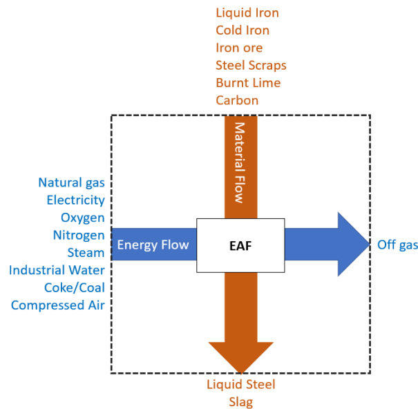
Figure 2.24. Energy and material flow for electric arc furnace (EAF) steelmaking
