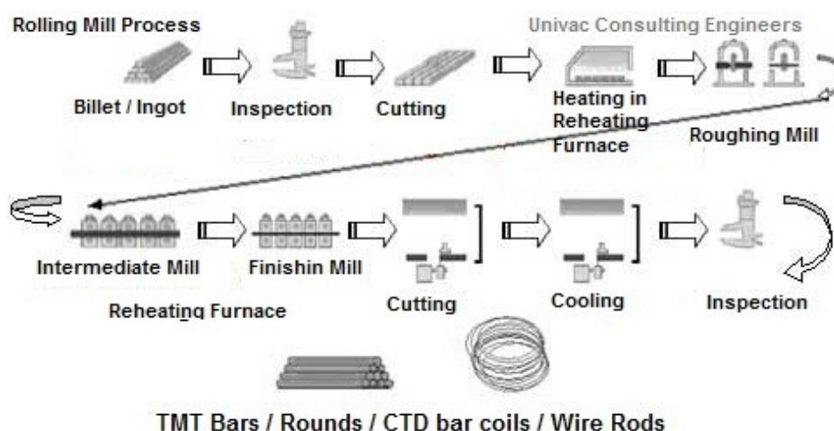
Figure 2.30. Hot rolling diagram [41]
