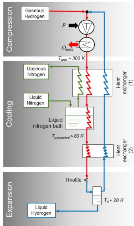
Figure 4.16. Joule-Thomson process with liquid nitrogen precooling.
