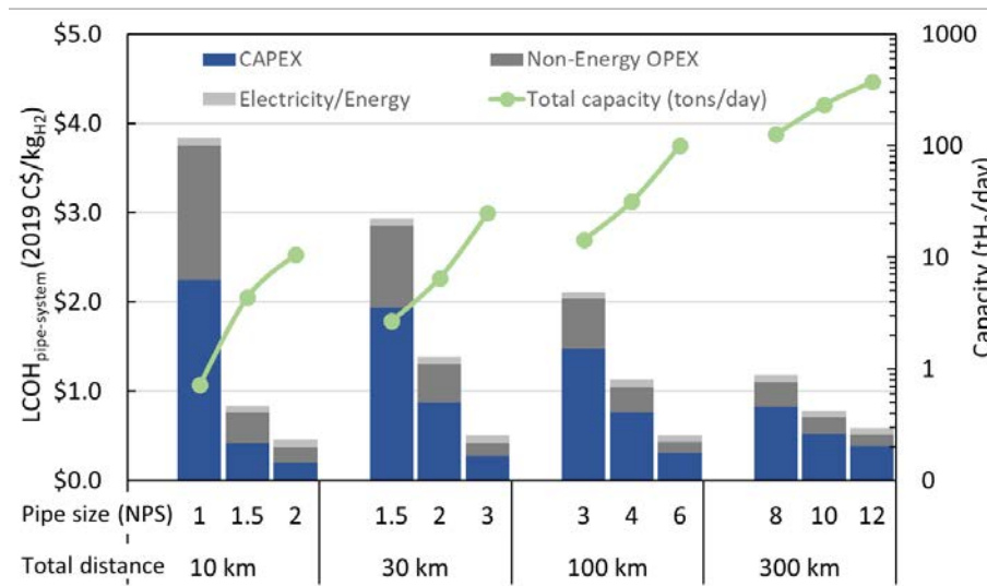
Figure 4.20. LCOH_{pipe-system} divided into: CAPEX_{pipe-system} , Non-Energy\ OPEX_{pipe-system} and Electricity/energy_{pipe-system} at different pipe sizes (NPS) and pipeline lengths, versus resulting capacities.
