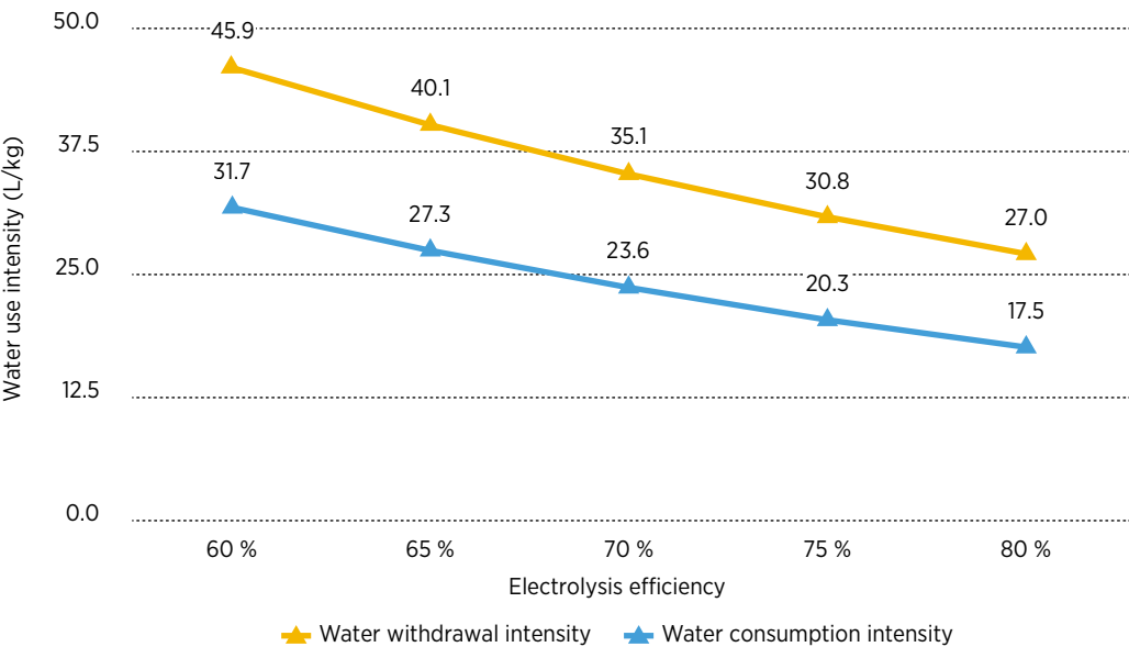
FIGURE 2.4 Relations between hydrogen conversion efficiency and water withdrawal and consumption intensities of a typical electrolysis project
