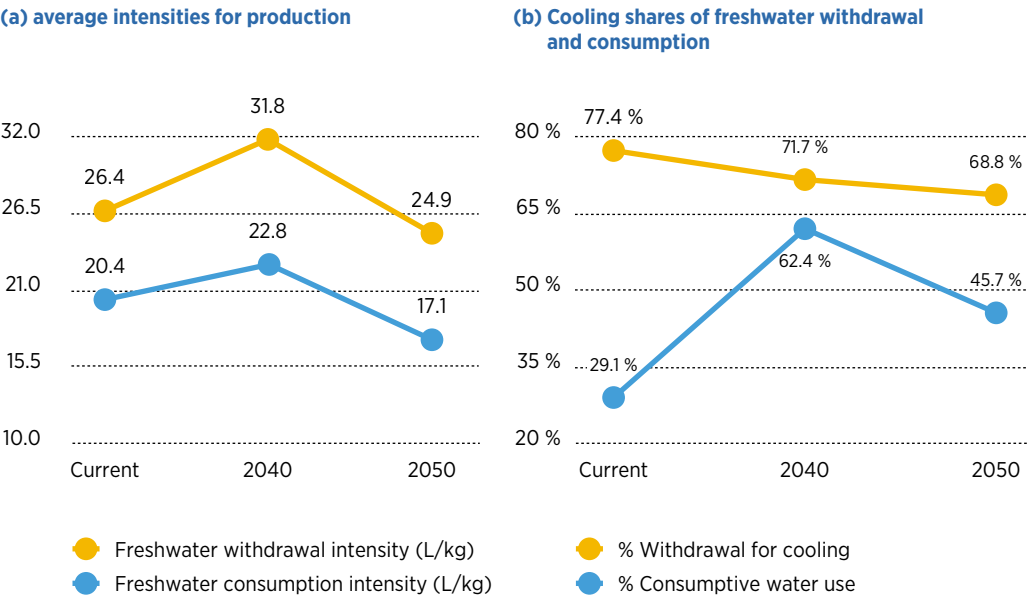
FIGURE 3.3 Freshwater for hydrogen production and cooling, today to 2050
