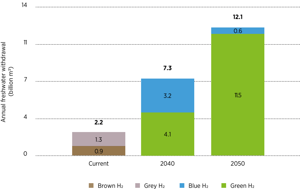
FIGURE 3.2 Current and projected freshwater withdrawal for global hydrogen production, by hydrogen production pathway
