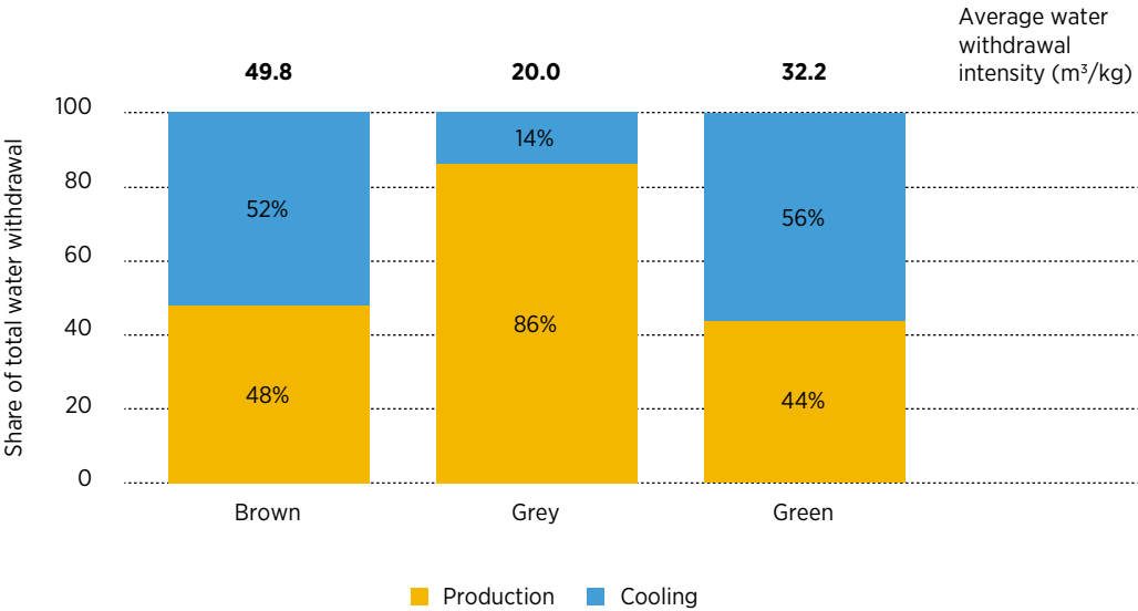
FIGURE 2.2 Share of the water withdrawal needs of production and cooling in the overall water demand of hydrogen production examples
