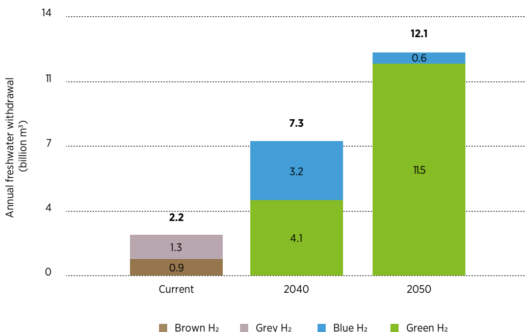
FIGURE S2 Current and projected freshwater withdrawal for global hydrogen production, by pathway
