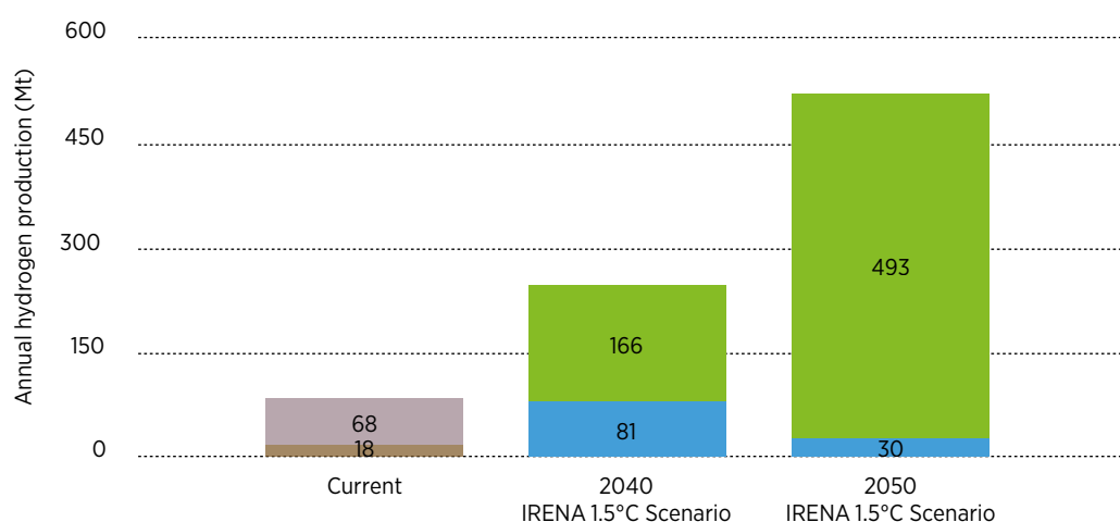
FIGURE 3.1 Current and projected future global hydrogen production under the 1.5°C Scenario
