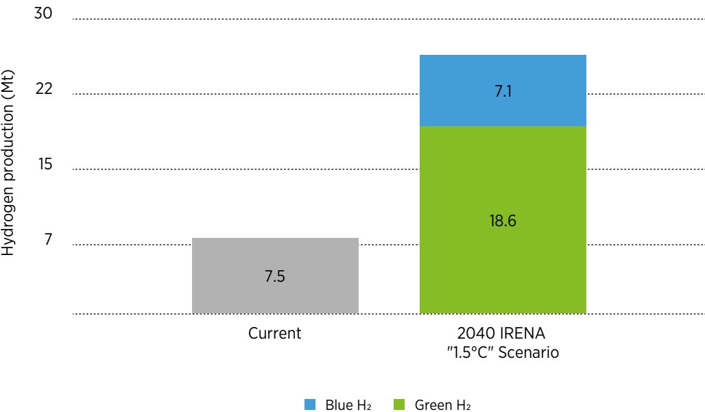
FIGURE 4.11 Current and projected hydrogen production in Europe
