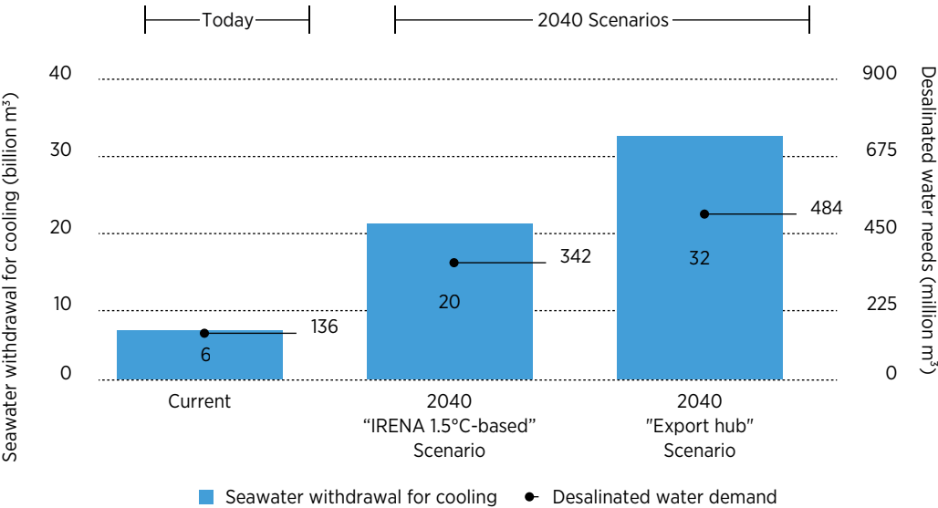
FIGURE 4.7 Current and projected seawater withdrawals and desalinated seawater requirements of hydrogen production in the Gulf Cooperation Council countries
