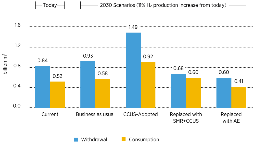
FIGURE 4.4 Annual water withdrawal and consumption requirements of coal-based hydrogen production in the Yellow River Basin under four scenarios
