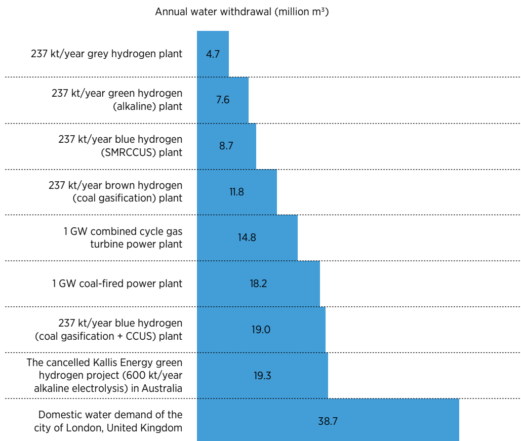
FIGURE 2.5 Annual water withdrawal of typical hydrogen production projects, thermal power plants and municipalities
