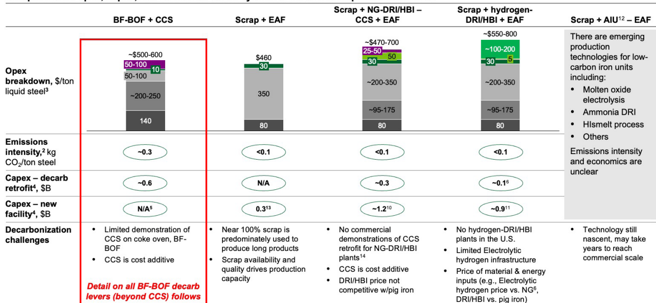
Figure 3.3.1: Costs above represent the perspective of steel producers | 1. Largely labor and mill maintenance | 2. Emissions intensity per ton of liquid steel assumes that grid decarbonization reaches 100% and is contingent on a carbon capture rate of 90% | 3. Assumes a scrap ratio of 60%, combined with iron units in EAF and a scrap ratio of 20% in BF-BOF | 4. Reflects costs for a 1.2 MT steel facility. Retrofit reflects the cost of CCS or hydrogen installation on an existing facility | 5. There are no domestic plans to build additional BF-BOF mills. | 6. Cost of retrofitting NG-DRI/HBI to hydrogen | 7. Scrap use is highly variable; many steelmakers will fluctuate the use of iron ore and scrap as the costs of these inputs change due to external conditions. | 8. The assumed range uses the cost difference between merchant and integrated DRI/HBI production. | 9. The range assumes an electrolytic hydrogen price of $2–$4/kg. | 10. Includes new NG-DRI/HBI built with CCS | 11. Includes electrolyzer | 12. Alternative iron units | 13. Cost to build a new EAF | 14. Recent deployment announcement by Nucor
