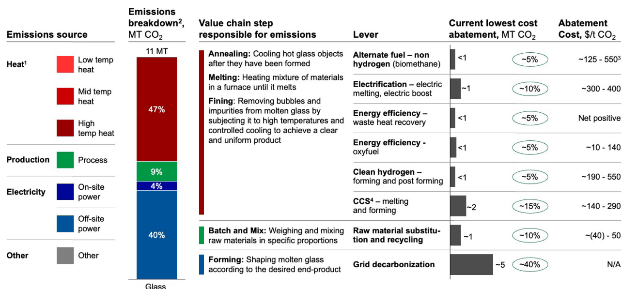
Figure 3.8.1: Glass production that can be abated using various levers (e.g., CCS, energy efficiency, electrification) | 1. Temperature ranges are defined as low-temperature heat (-30°C to 200°C), medium-temperature heat (200°C to 400°C), and high-temperature heat (400+°C). | 2. Breakdown of 2021 glass production emissions | 3. The lower bound represents estimates for biomethane forming in container glass, and the higher bound represents estimates for biomethane melting in container glass. | 4. The displayed cost estimates are based on the capture costs from various sources (see the appendix for details) with transport (GCCSI, 2019) and storage (BNEF, 2022) costs of ~$10–40/t; all figures are in 2022 dollars. All CCS figures represent retrofits, not new-build facilities. The lower-bound costs represent a NOAK plant in a low-cost retrofit scenario with low inflation. The higher-bound costs represent a FOAK plant in a high-cost retrofit scenario with high inflation.
