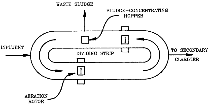
Figure 5. Oxidation ditch flow diagram.
