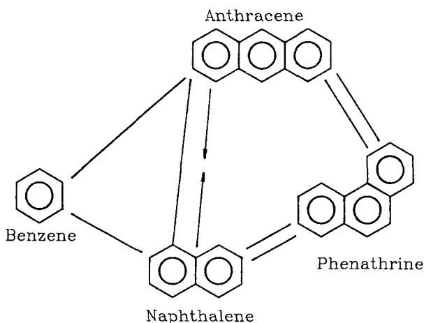
Figure 6. Proposed relationship between benzene and the PAHs used in the study.
