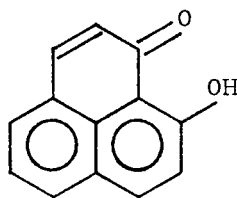
4 hydroxyperinapthenone
