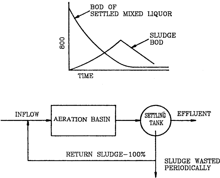
Figure 4. Extended aeration activated sludge.
