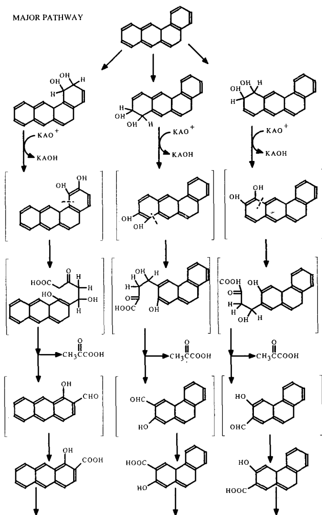
Figure 8. Proposed pathways for the metabolism of benz(a)anthracene by Beijerinckia strain B1. Reprinted from Mahaffey, et al., App & Env Mic , Oct. '88, p. 2421.
