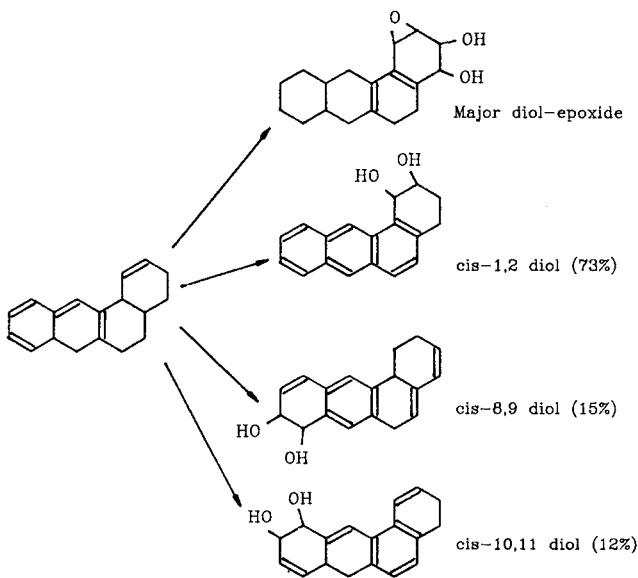
Figure 7. Chemical transition structure.
