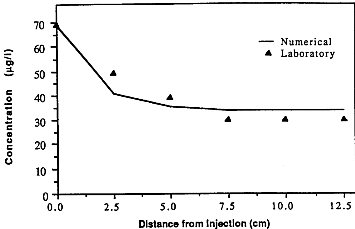
Figure 5. Prediction of the CTC profile at a detention time of 125 min. and with k = 0.030 \mu\text{g/mg cell-day} and K_s = 4.5 \mu\text{g/l} .
