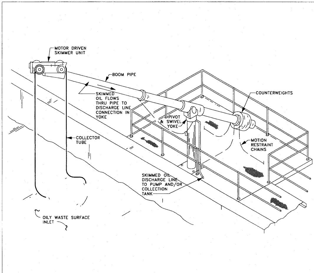
Figure 16 Tube Type Oil Skimmer Installation
