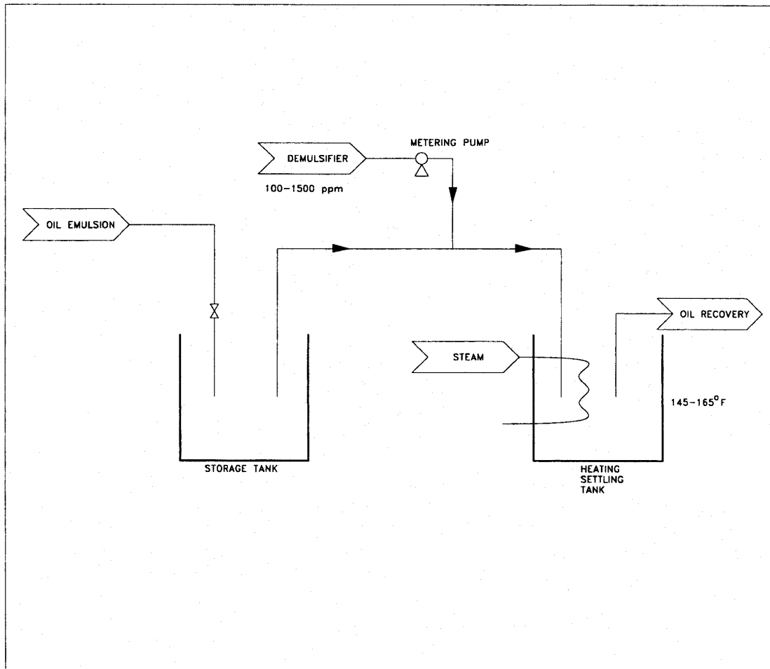
Figure 26 Oil Emulsion Treatment Schematic
