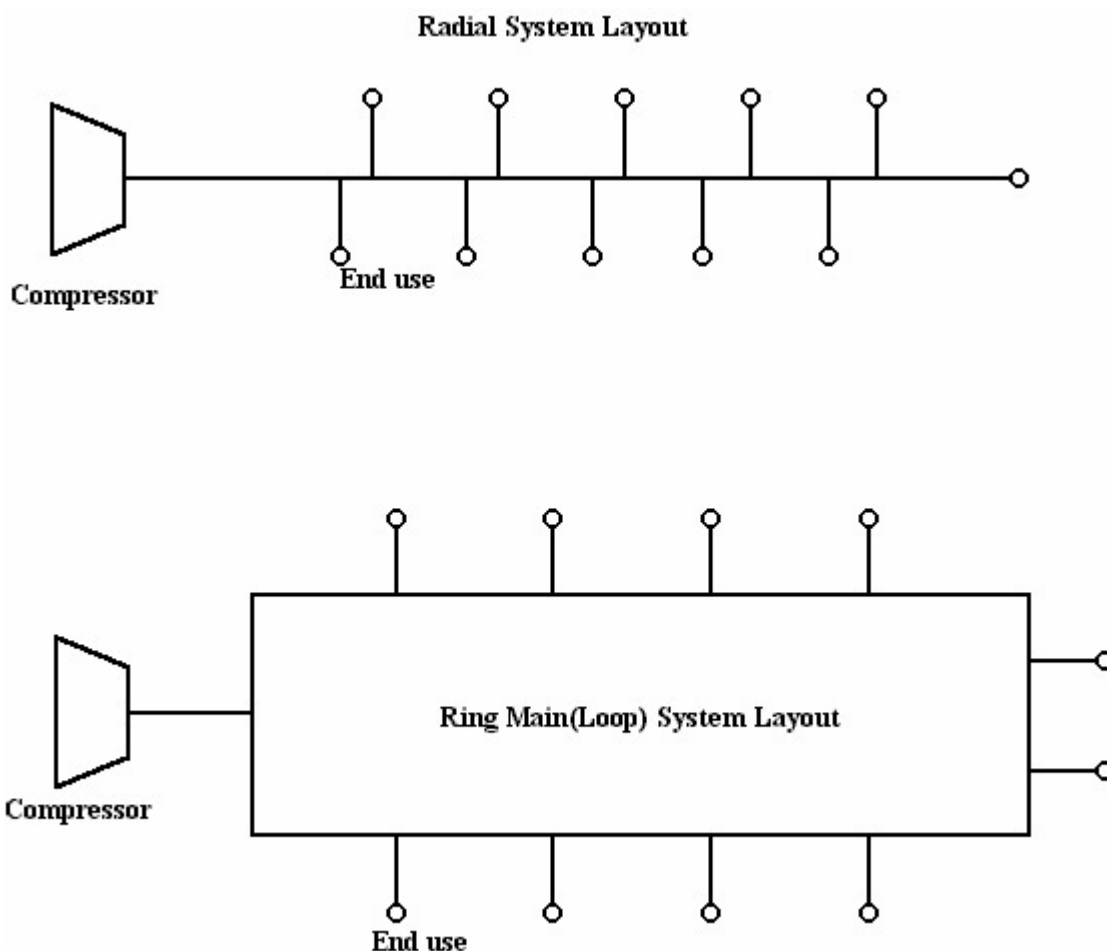
Figure 3-2: Types of piping layout
