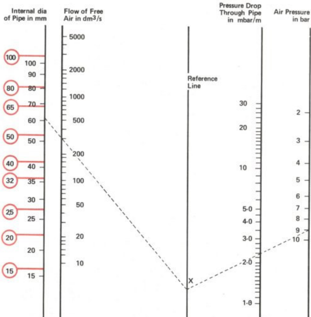
Figure 3-1: Pressure drop calculations
