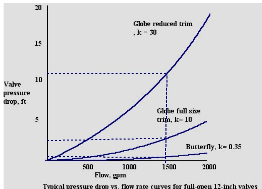
Typical pressure drop vs. flow rate curves for full-open 12-inch valves Figure 7-3: Pressure drop of Globe & Butterfly Valves
