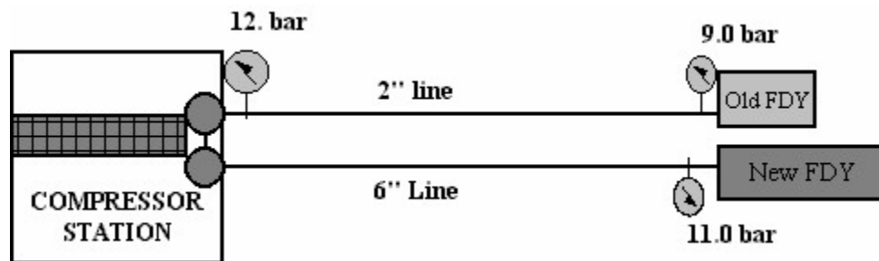
Figure 7-2: Compressed air system piping schematic
