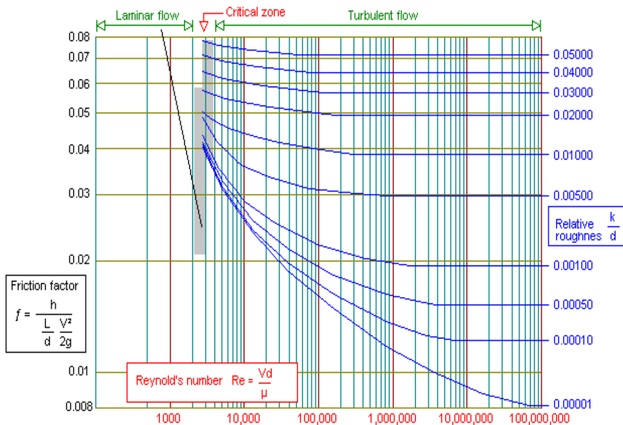
Figure 2-1: Estimation of friction factor
