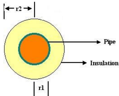
Figure 6-2: Insulated pipe section
