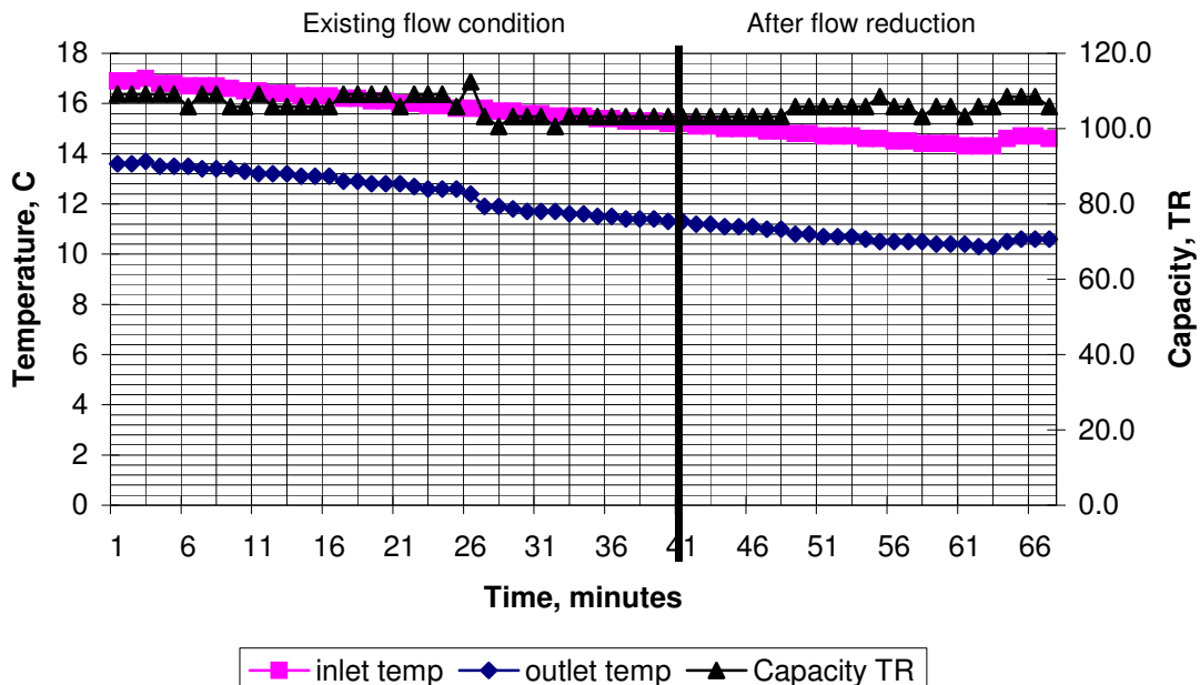
Figure 7-4: Chiller performance
