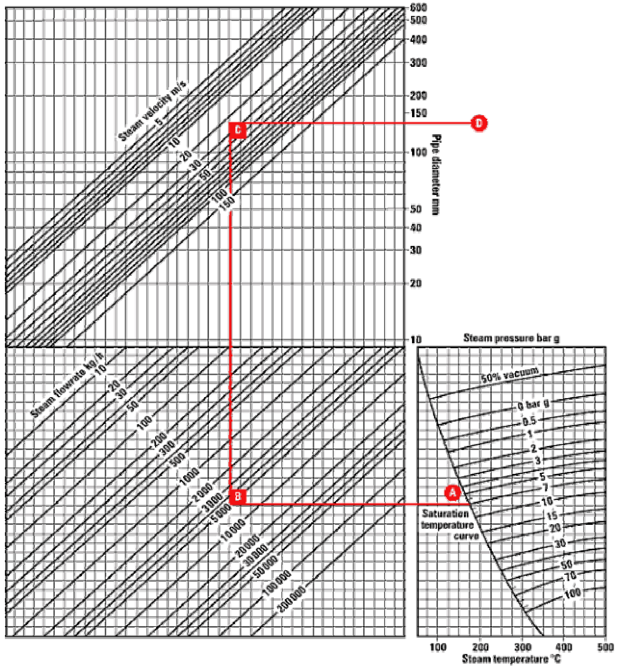
Figure 4-1: Steam pipe sizing
