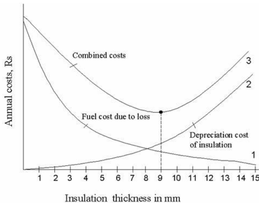
Figure 6-1: Economic insulation thickness
