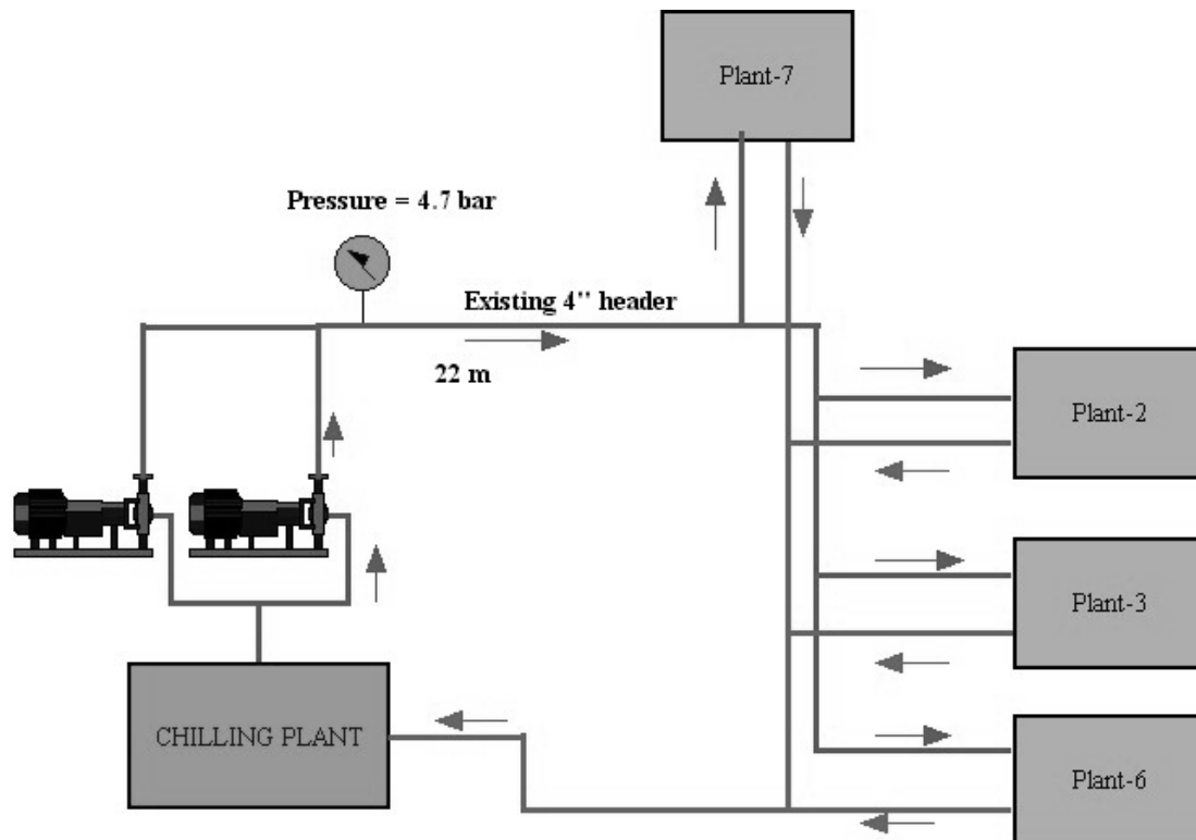
Figure 7-1: Chilled water system piping schematic
